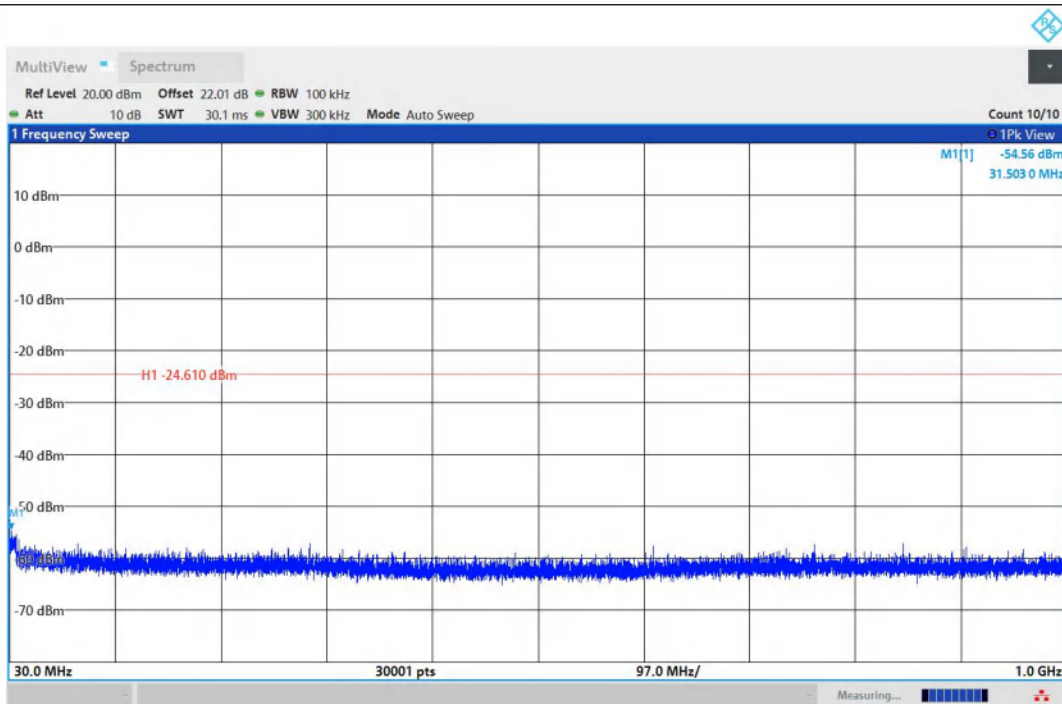
11B-Ant1-2412-30~1000-PASS
