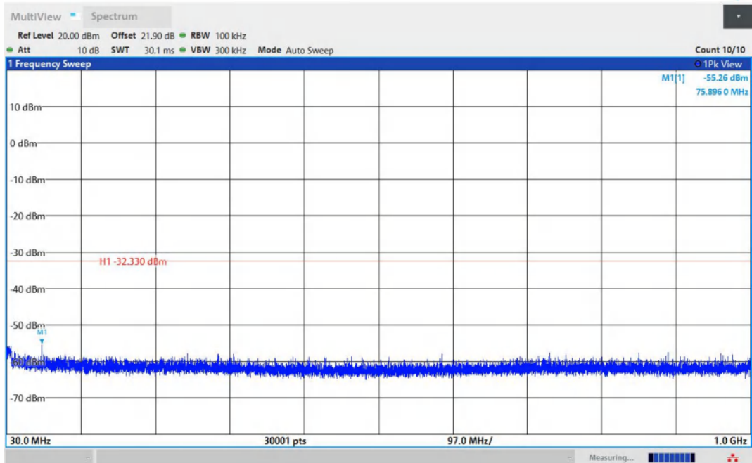
11N40MIMO-Ant2-2452-30~1000-PASS
