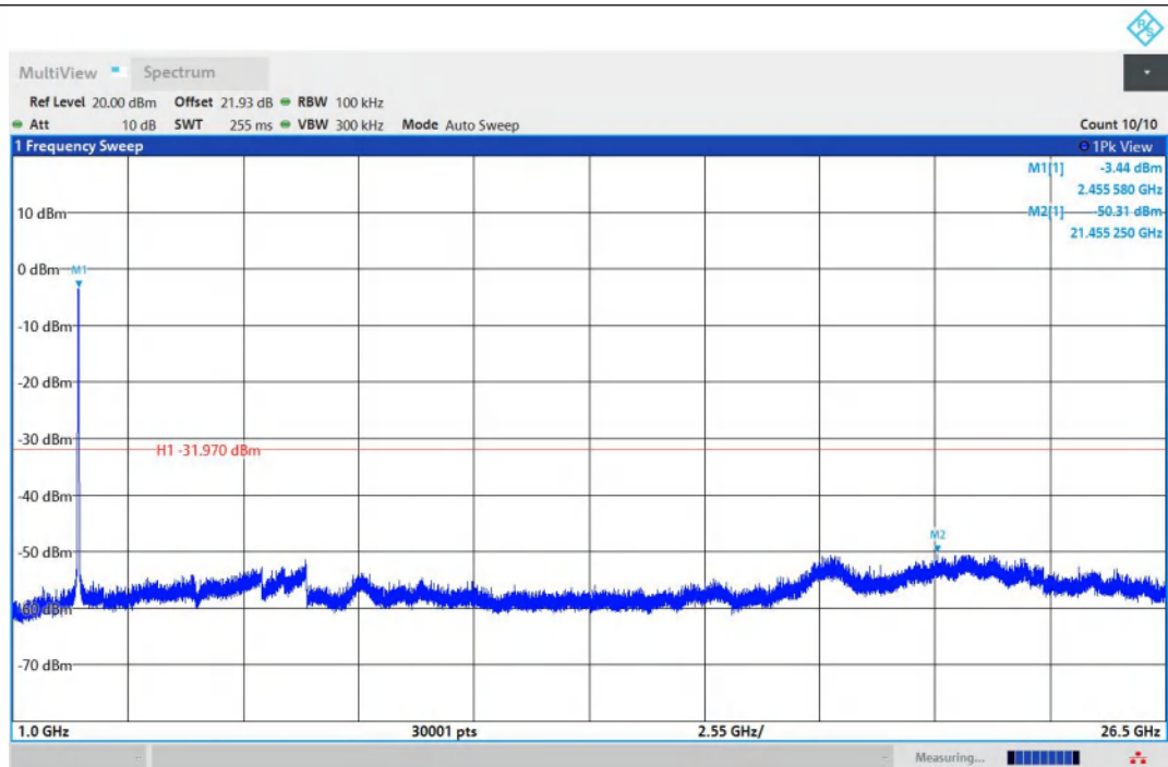
11N40MIMO-Ant1-2452-1000~26500-PASS
