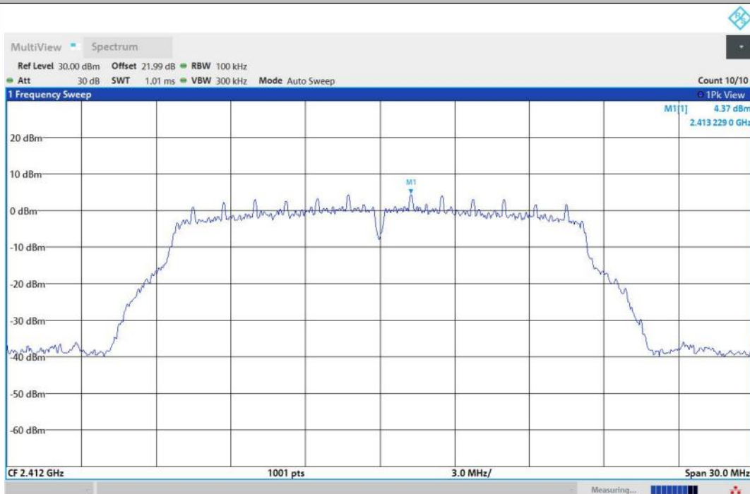
11G-Ant2-2412-0~Reference-PASS
