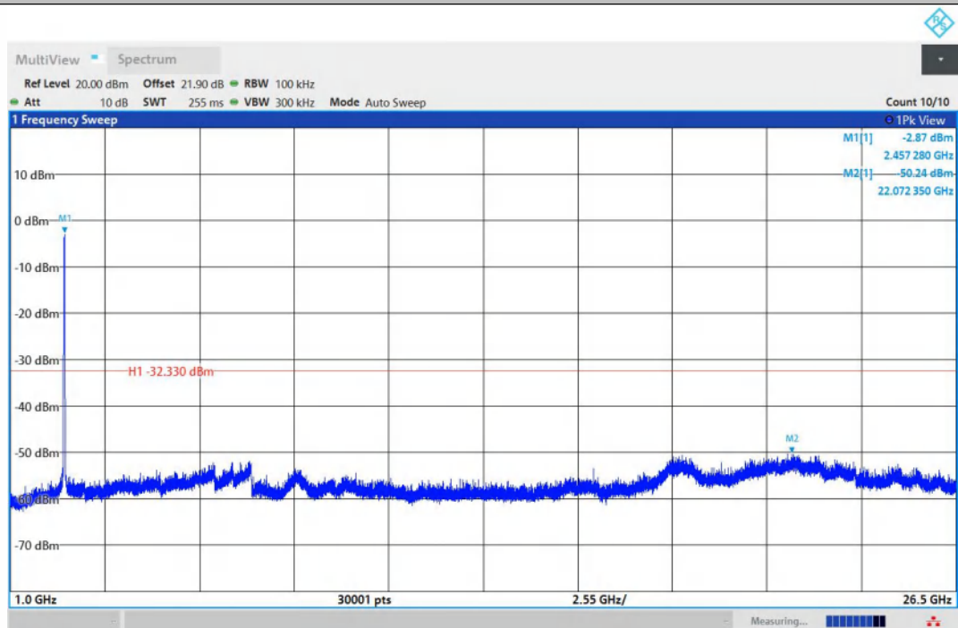
11N40MIMO-Ant2-2452-1000~26500-PASS
