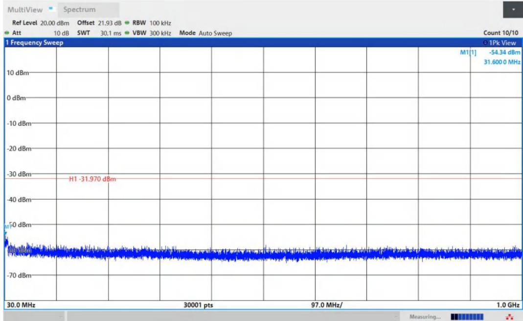
11N40MIMO-Ant1-2452-30~1000-PASS
