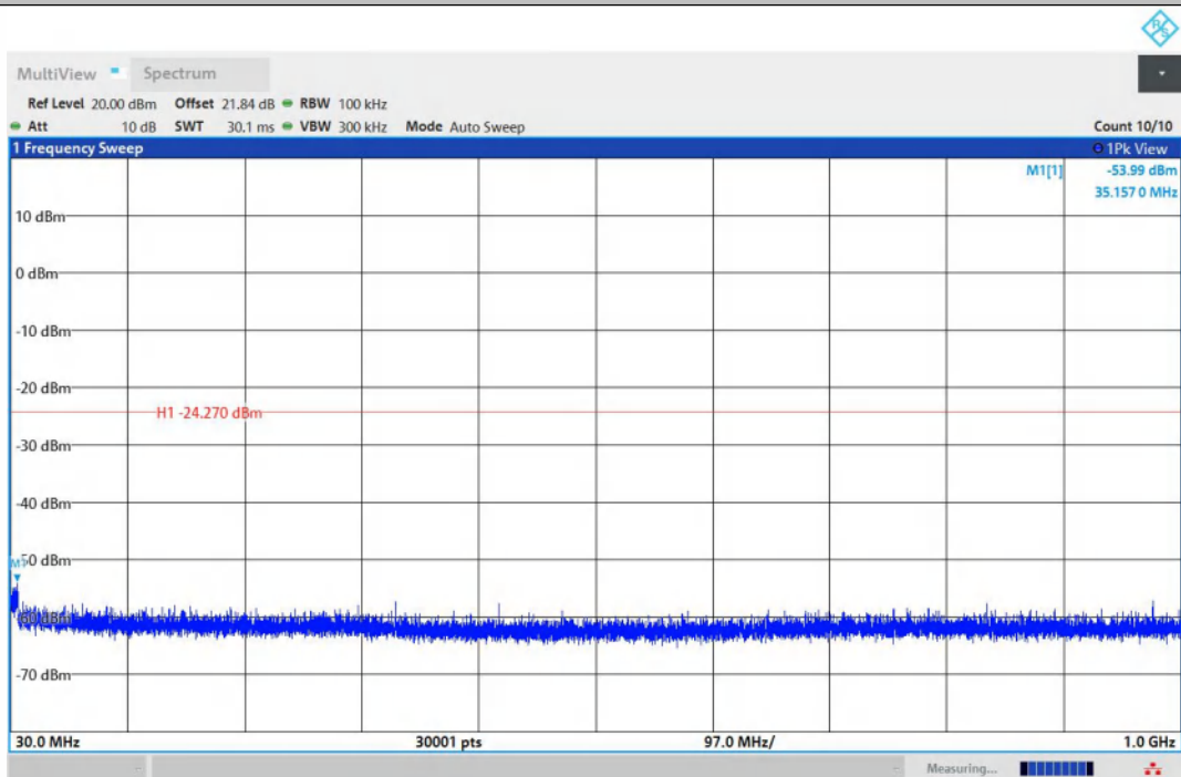
11B-Ant2-2437-30~1000-PASS
