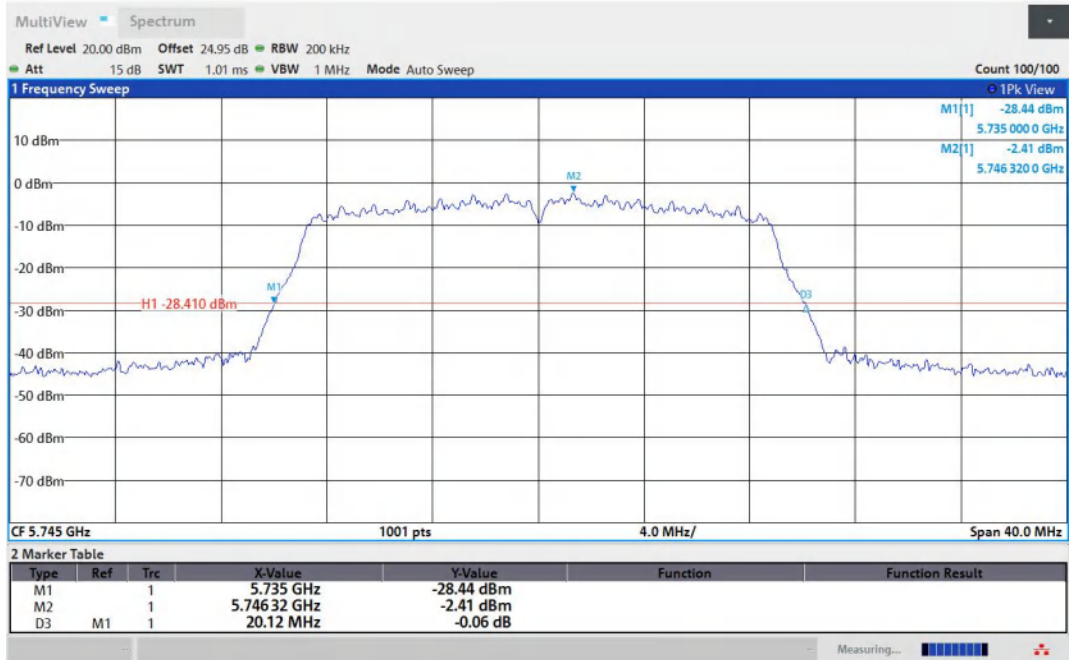
11AC20MIMO-Ant1-5745
