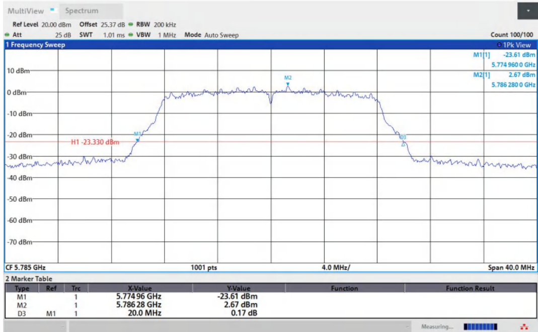
11A-Ant1-5785
