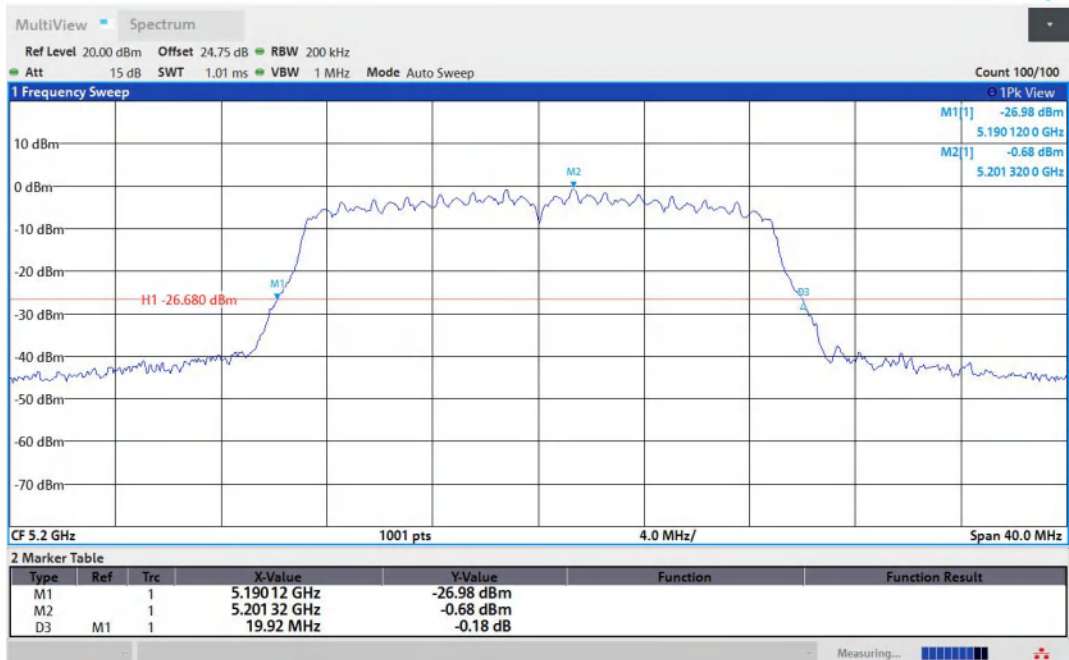
11AC20MIMO-Ant2-5200
