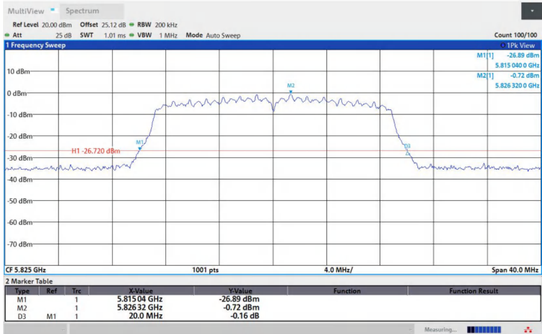
11N20MIMO-Ant2-5825
