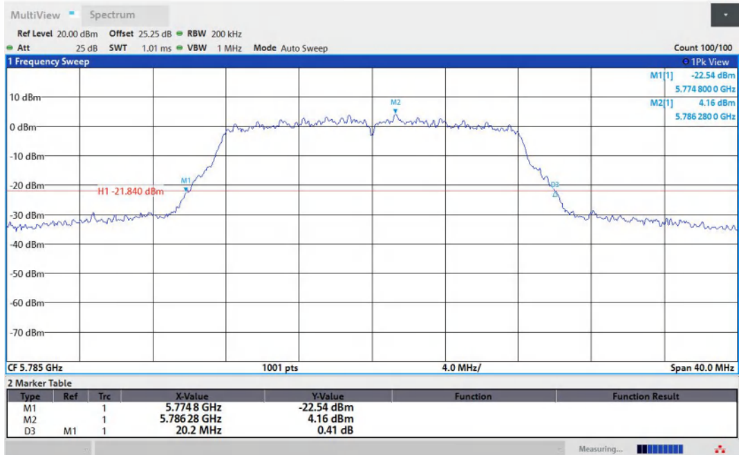
11A-Ant2-5785
