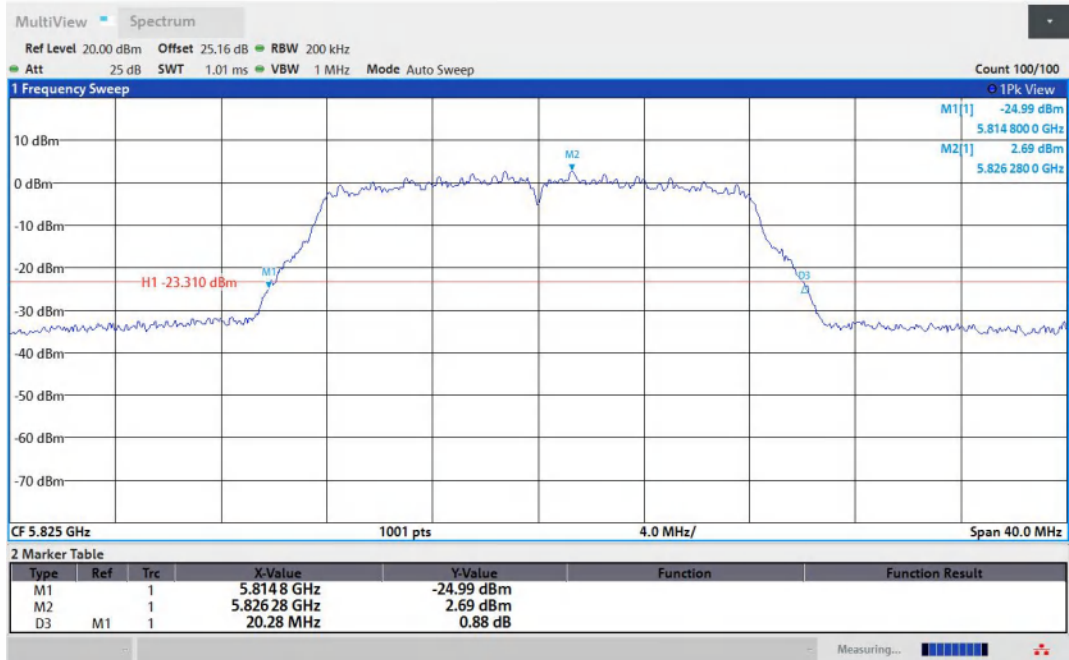
11A-Ant1-5825
