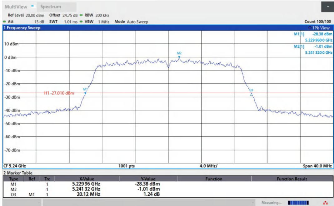
11AC20MIMO-Ant1-5240
