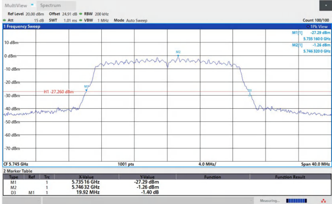
11AC20MIMO-Ant2-5745
