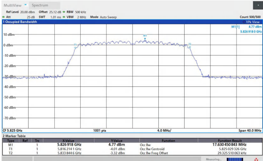
11N20MIMO-Ant2-5825
