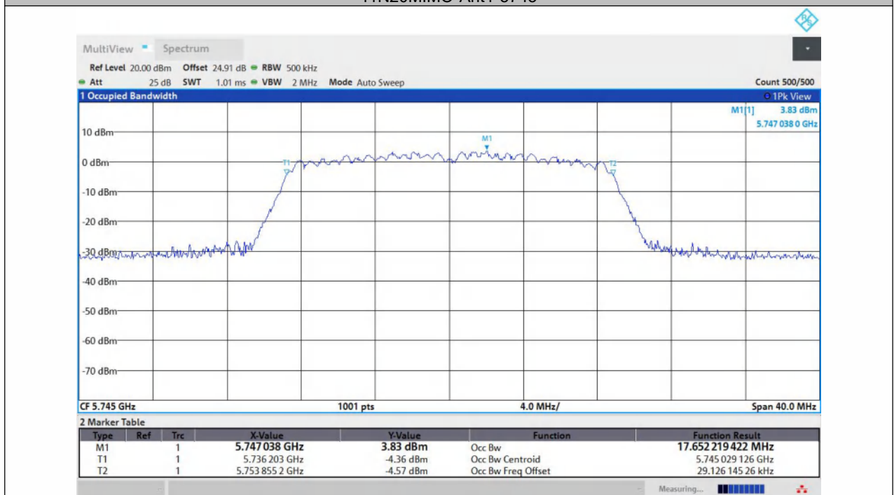
11N20MIMO-Ant2-5745
