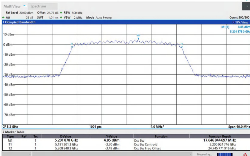
11AC20MIMO-Ant2-5200
