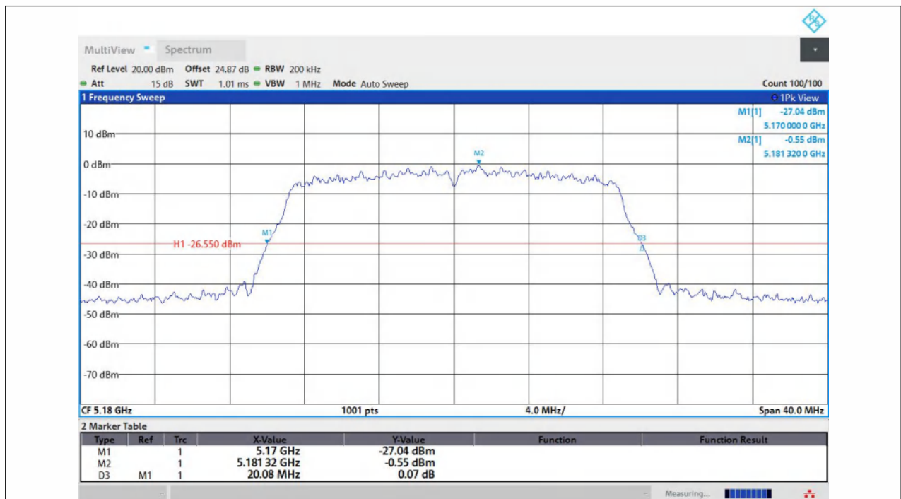
11AC20MIMO-Ant1-5180
