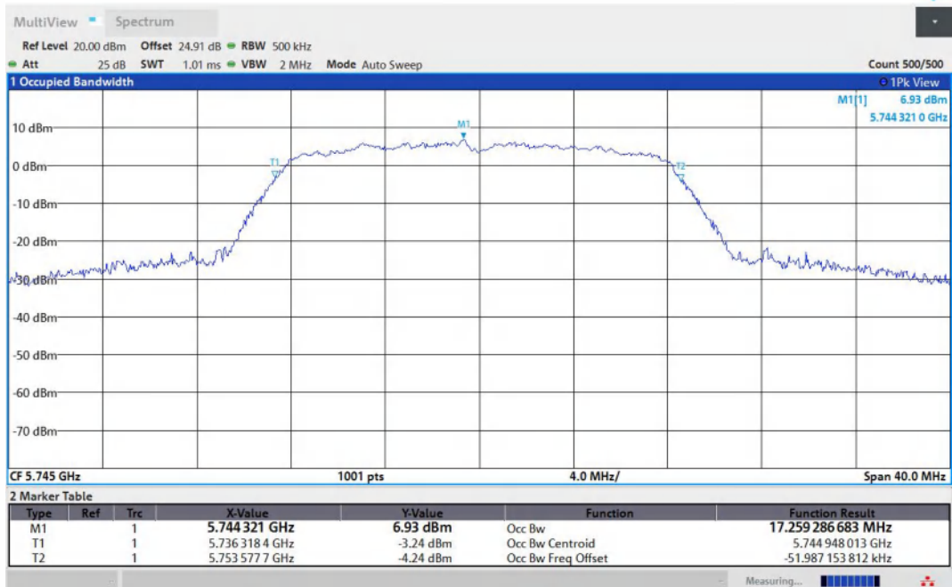
11A-Ant2-5745
