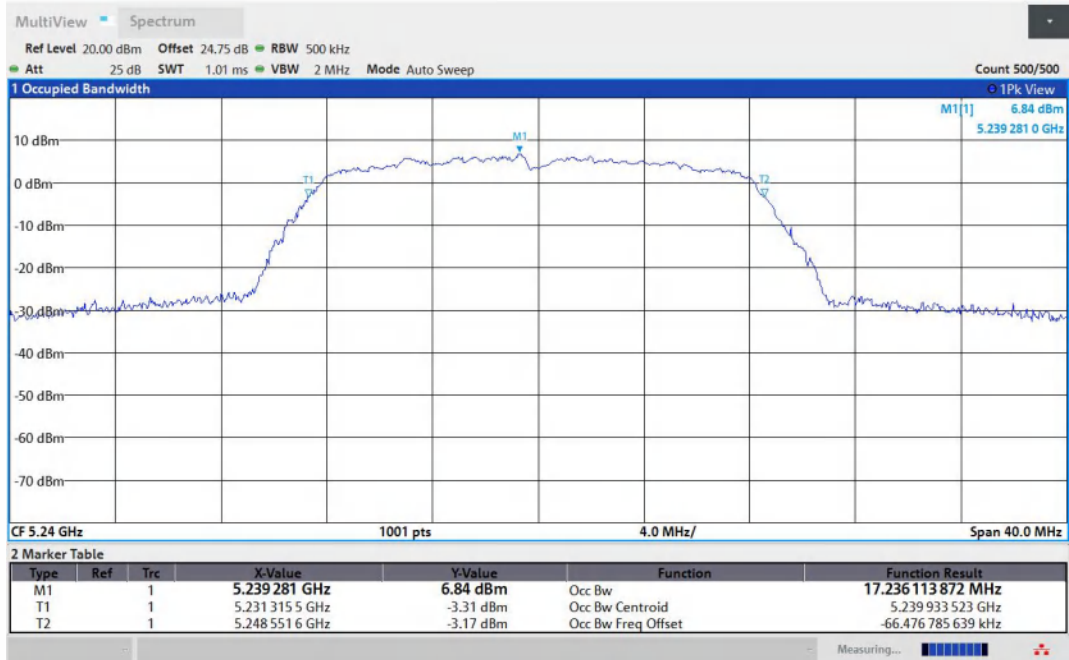
11A-Ant1-5240
