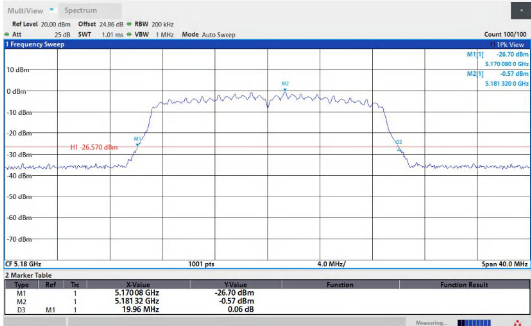
11N20MIMO-Ant2-5180
