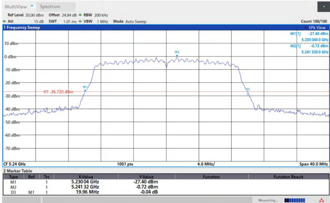
11AC20MIMO-Ant2-5240
