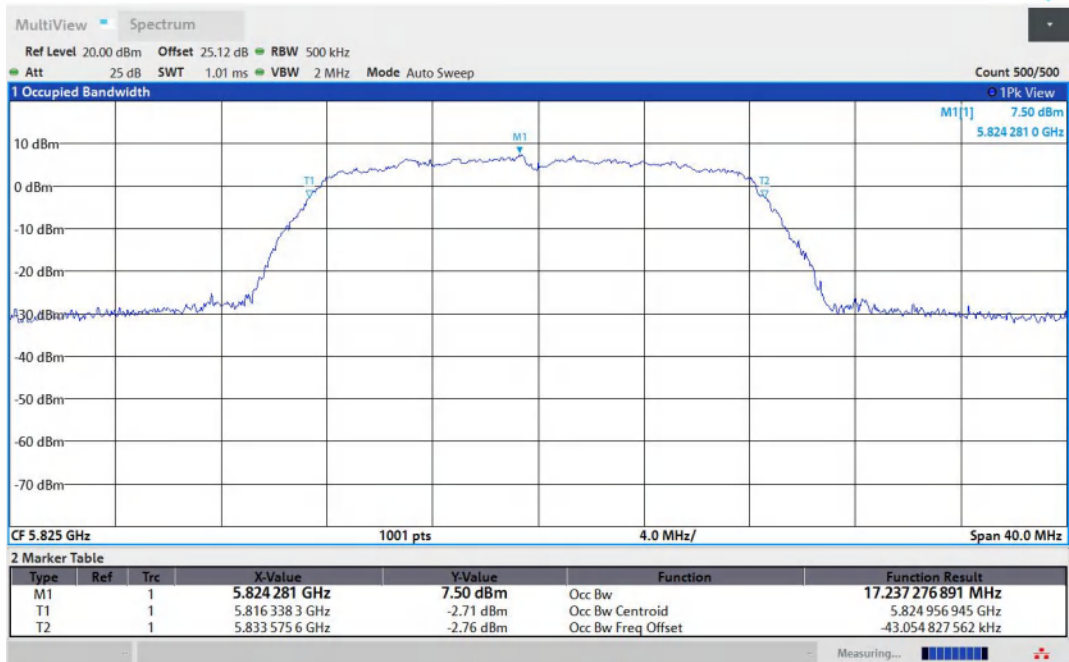
11A-Ant2-5825
