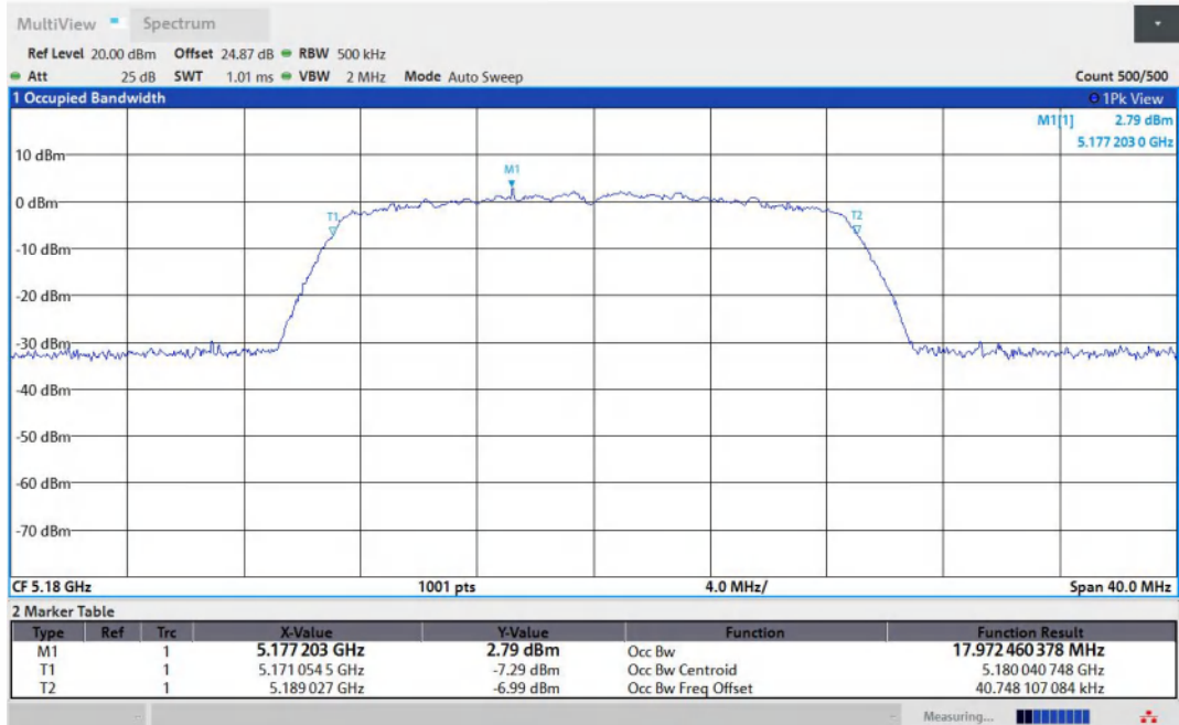
11AC20MIMO-Ant1-5180
