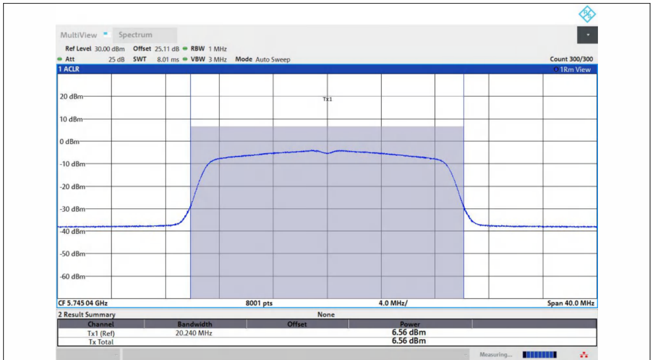
11N20MIMO-Ant1-5745-PASS
