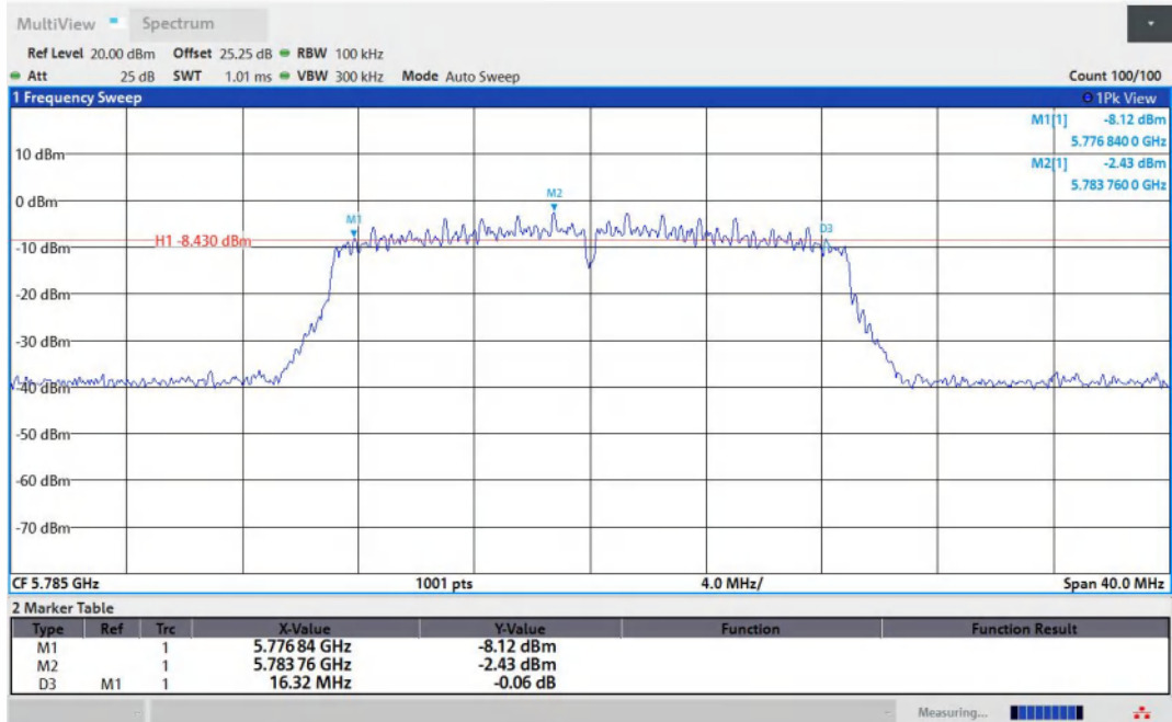
11AC20MIMO-Ant2-5785-PASS
