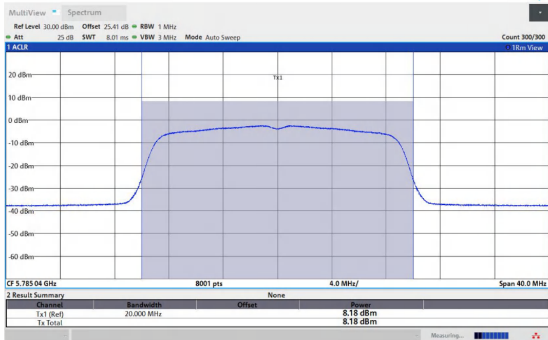
11N20MIMO-Ant2-5785-PASS
