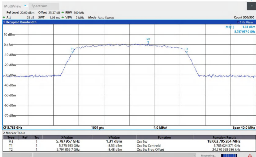
11AC20MIMO-Ant1-5785
