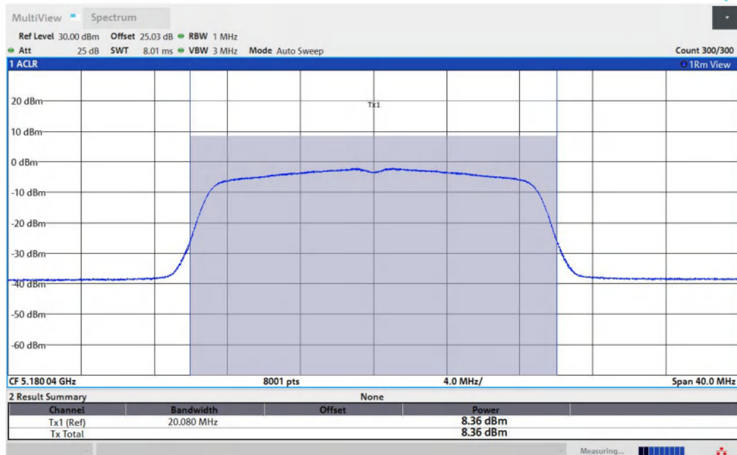
11AC20MIMO-Ant1-5180-PASS
