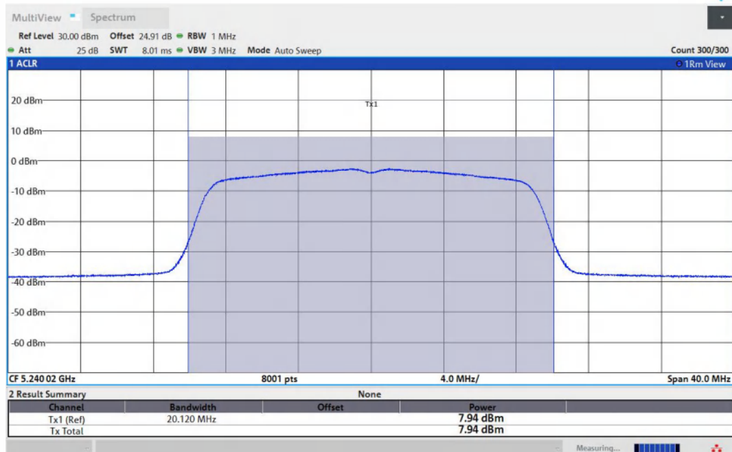
11AC20MIMO-Ant1-5240-PASS
