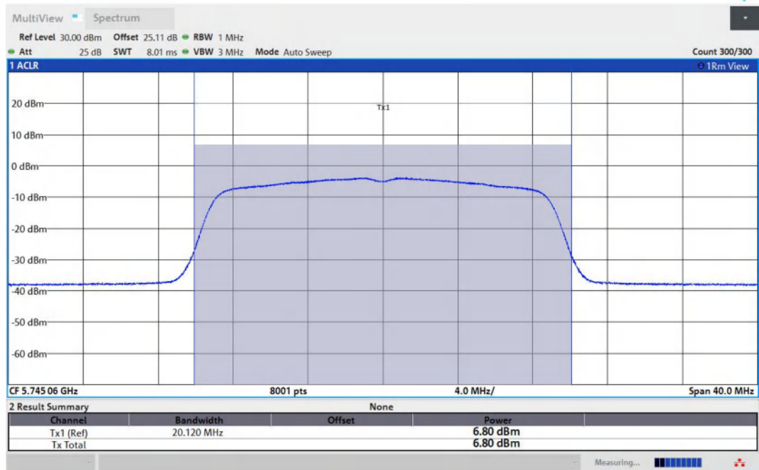
11AC20MIMO-Ant1-5745-PASS
