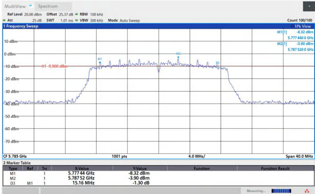
11N20MIMO-Ant1-5785-PASS
