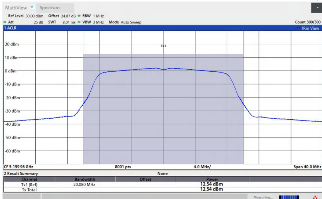
11A-Ant1-5200-PASS
