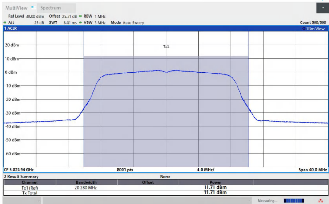
11A-Ant1-5825-PASS
