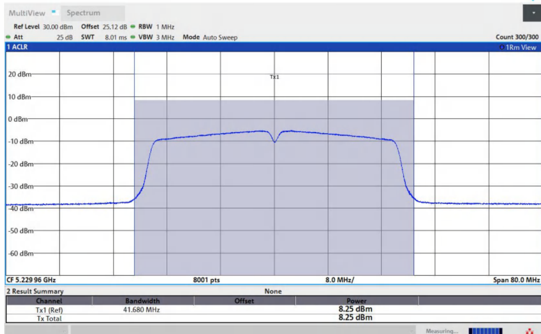
11N40MIMO-Ant1-5230-PASS
