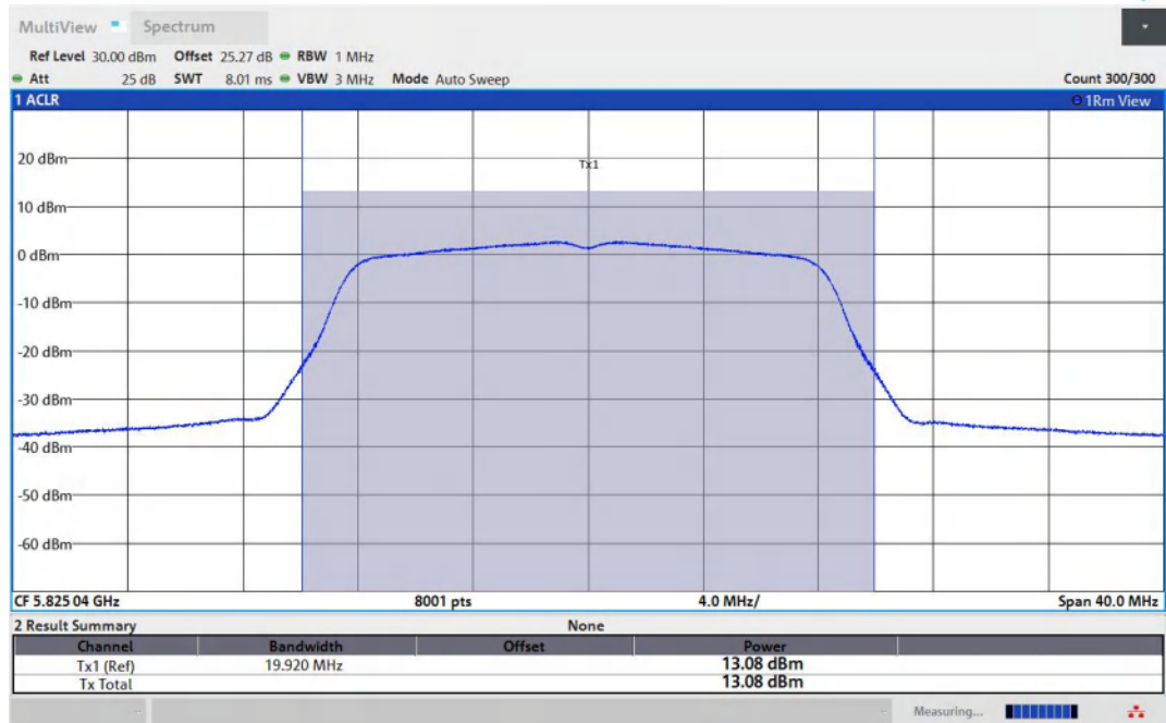
11A-Ant2-5825-PASS
