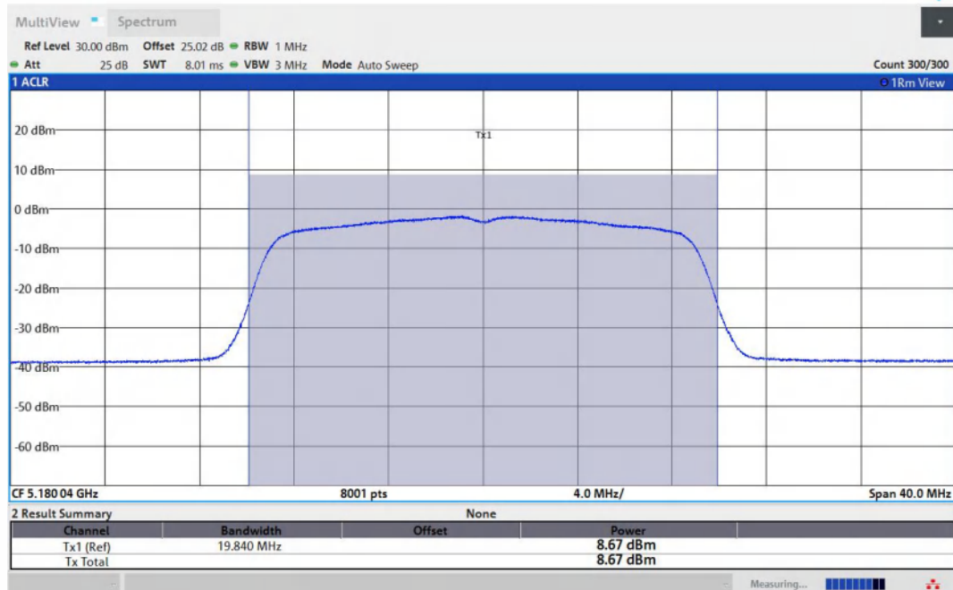
11AC20MIMO-Ant2-5180-PASS
