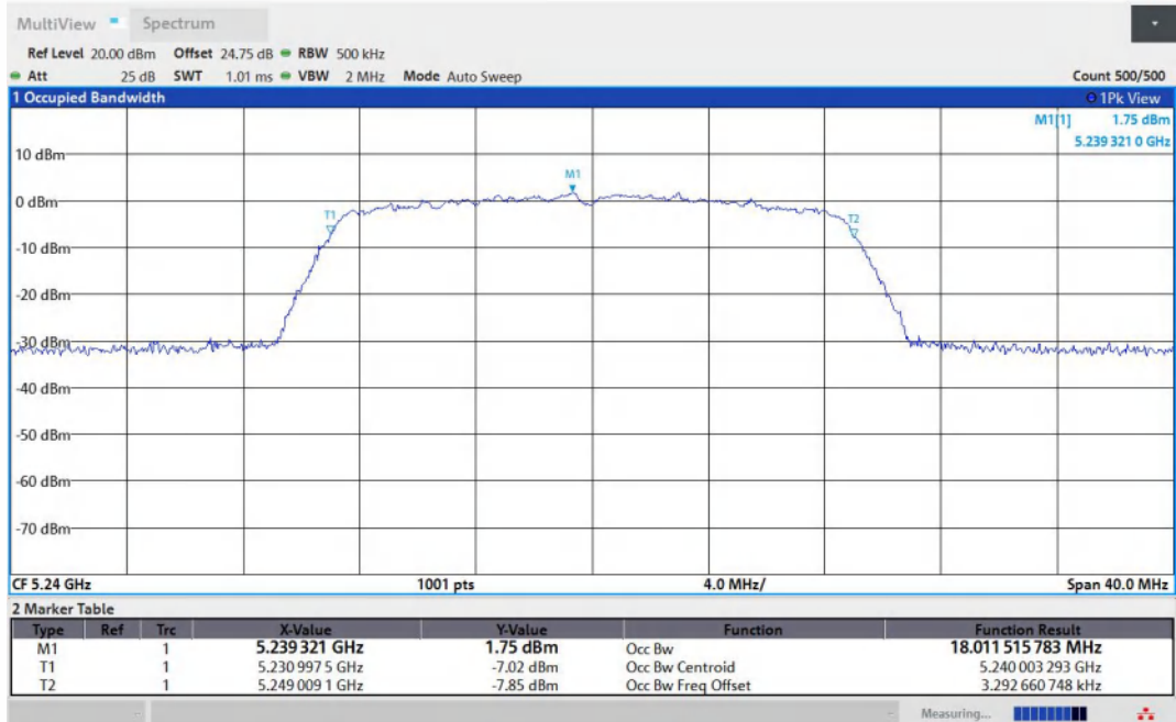
11AC20MIMO-Ant1-5240
