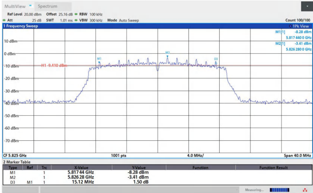
11N20MIMO-Ant1-5825-PASS
