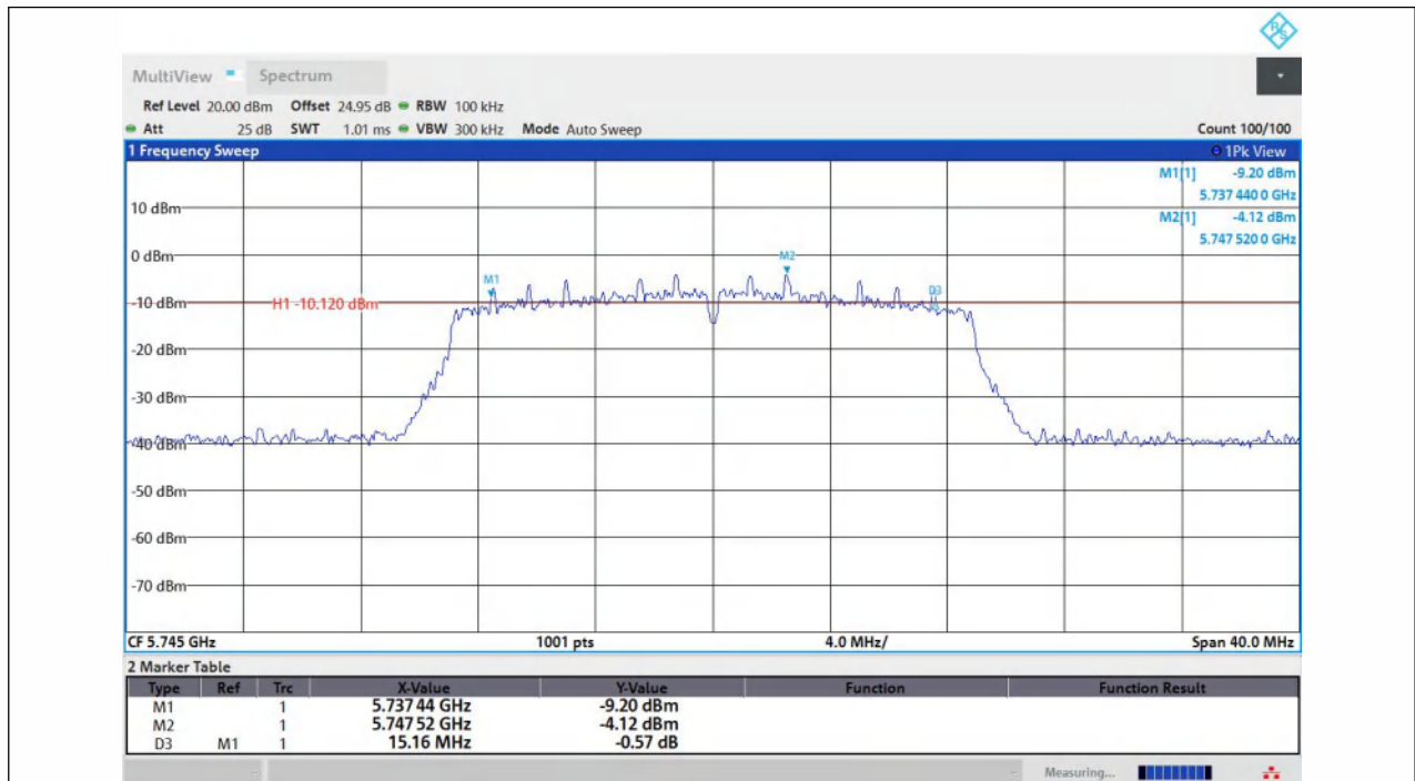
11AC20MIMO-Ant1-5745-PASS
