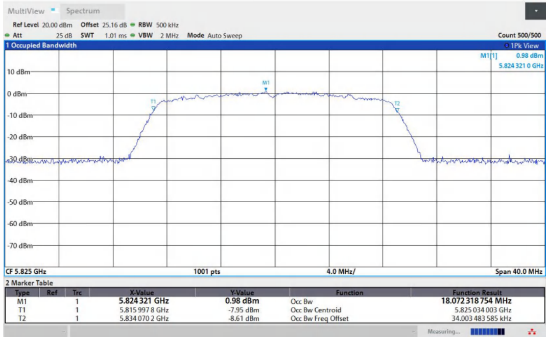
11AC20MIMO-Ant1-5825
