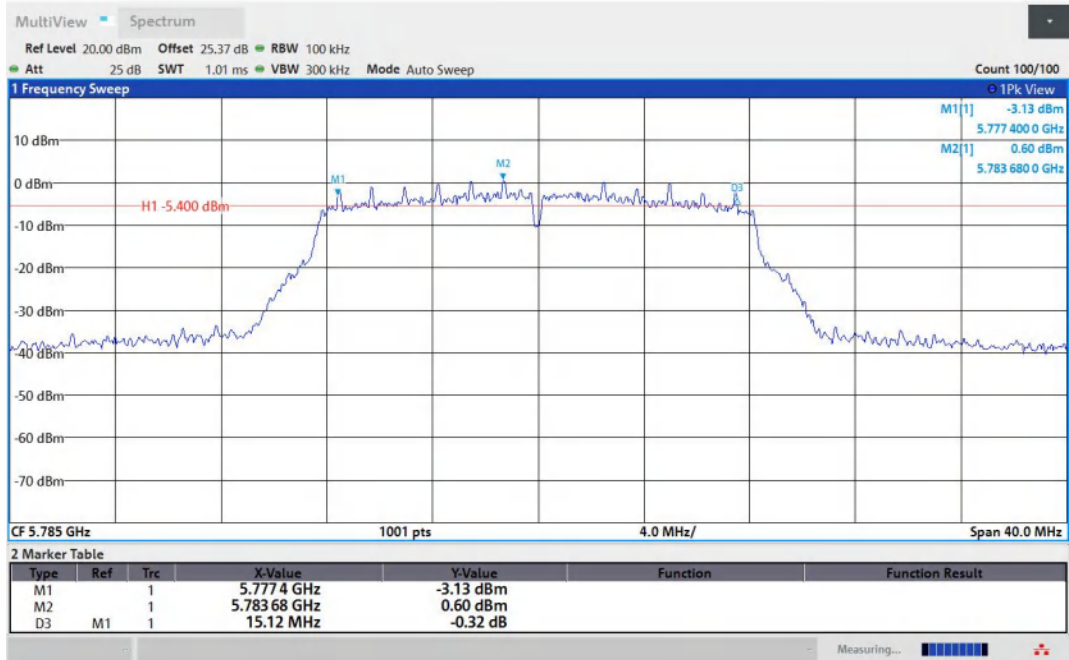
11A-Ant1-5785-PASS
