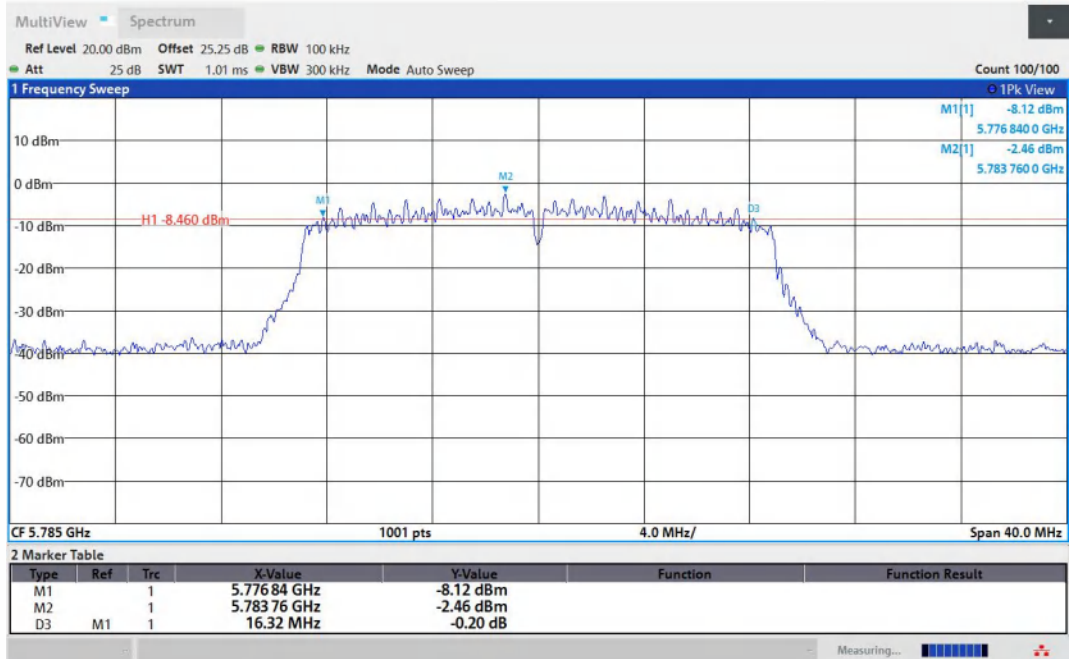
11N20MIMO-Ant2-5785-PASS
