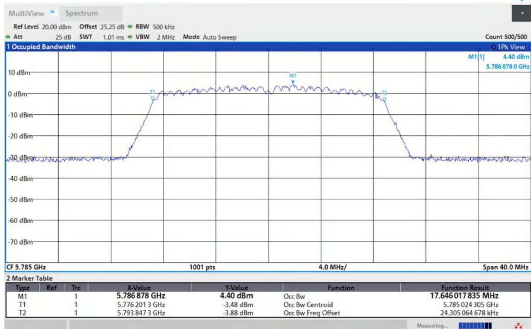
11AC20MIMO-Ant2-5785
