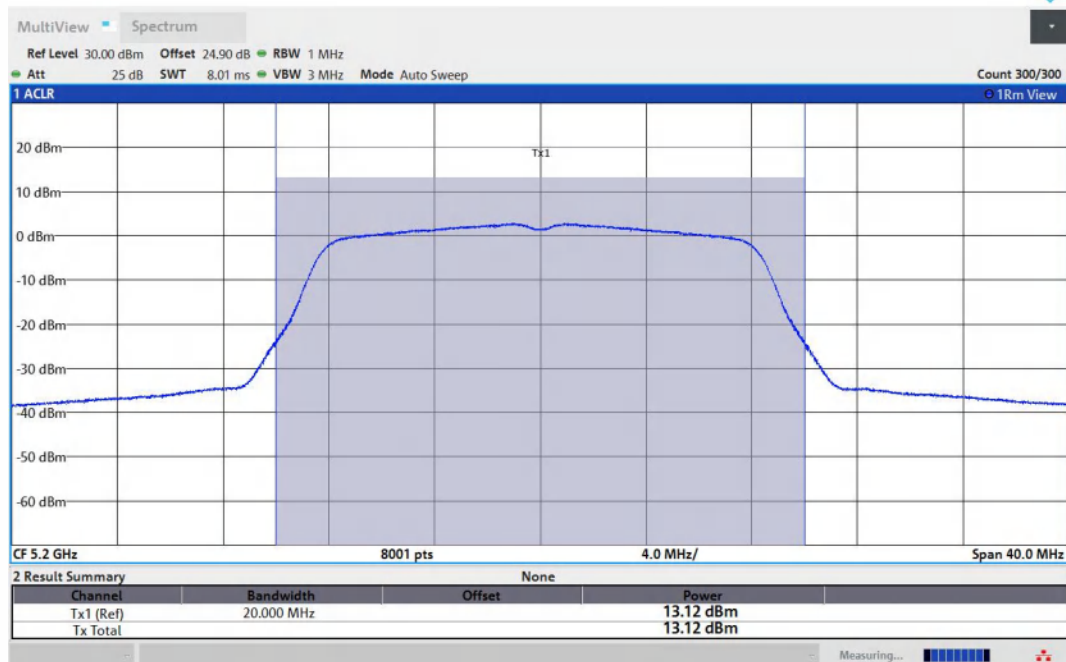
11A-Ant2-5200-PASS
