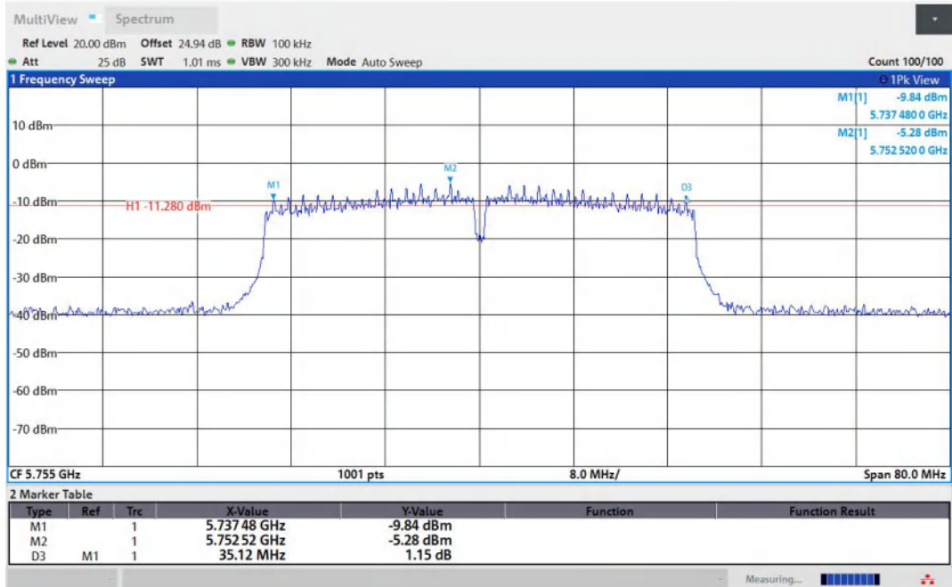
11N40MIMO-Ant2-5755-PASS
