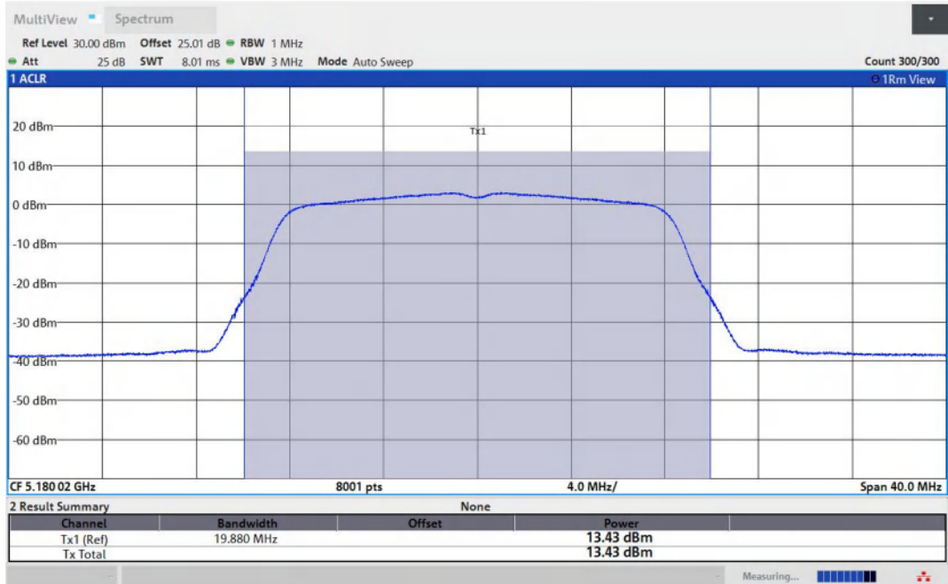
11A-Ant2-5180-PASS
