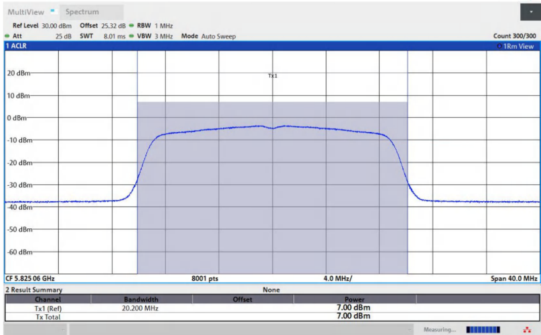
11N20MIMO-Ant1-5825-PASS
