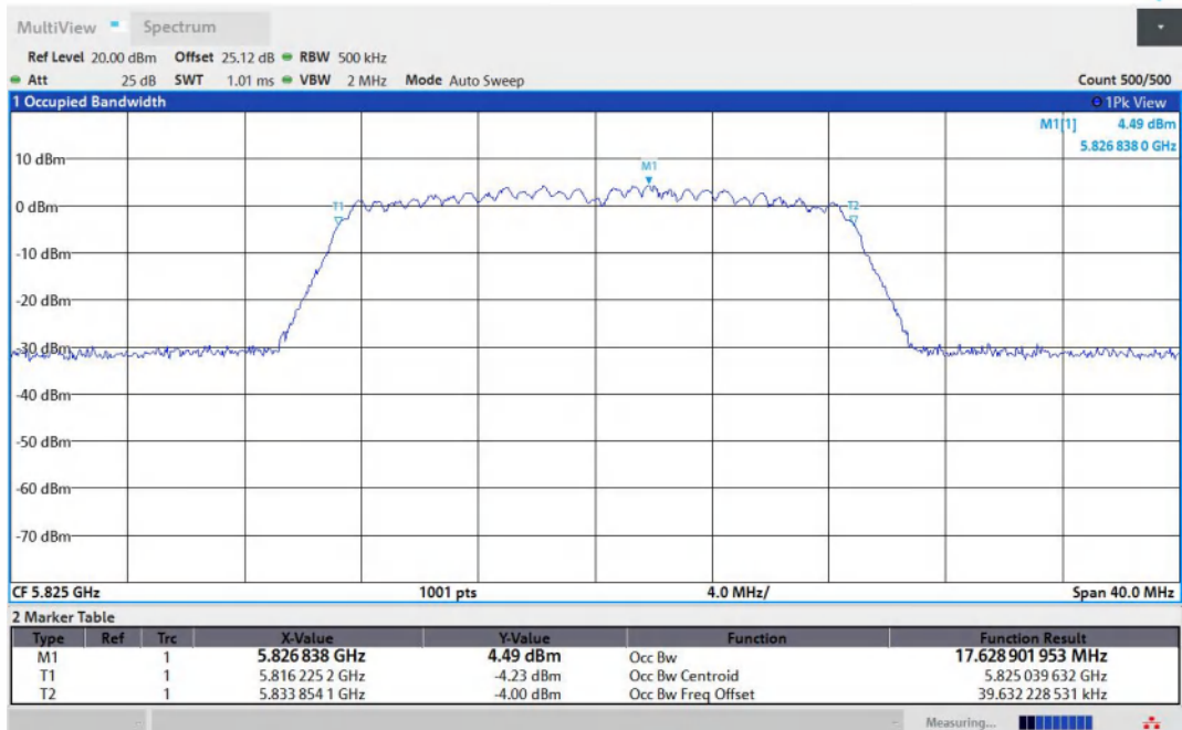
11AC20MIMO-Ant2-5825
