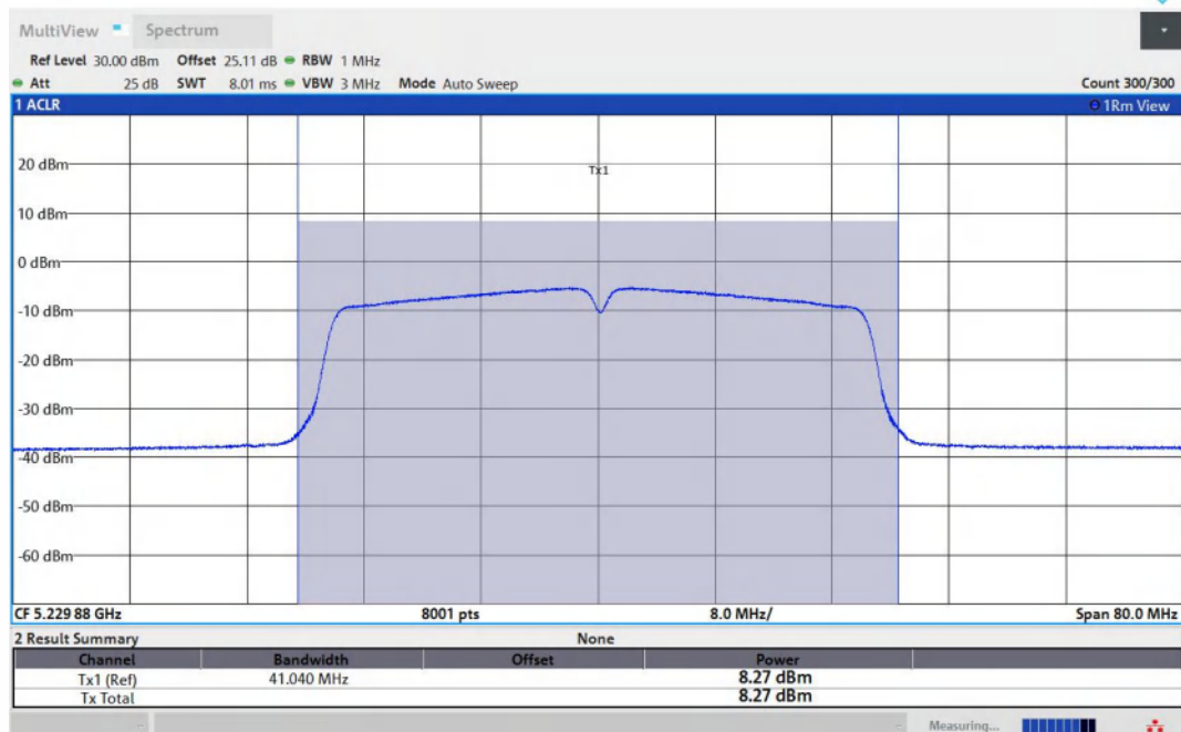
11AC40MIMO-Ant1-5230-PASS
