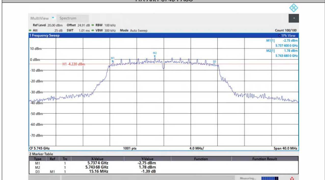
11A-Ant2-5745-PASS
