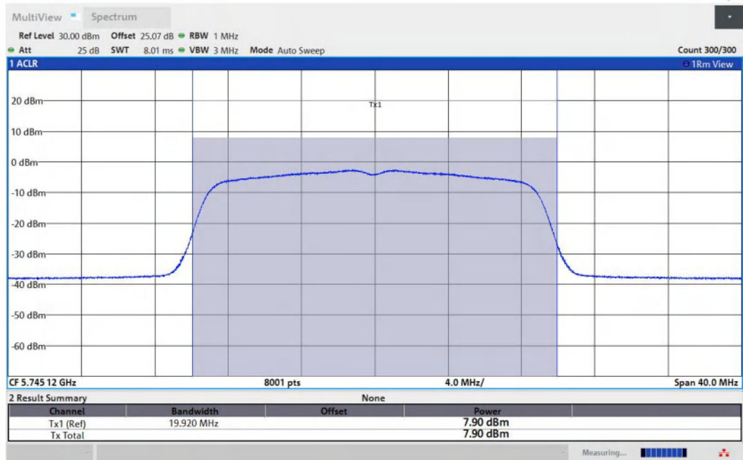
11AC20MIMO-Ant2-5745-PASS
