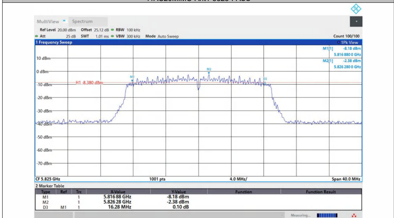
11AC20MIMO-Ant2-5825-PASS
