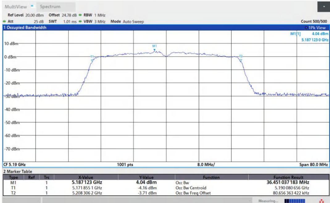
11AC40MIMO-Ant2-5190
