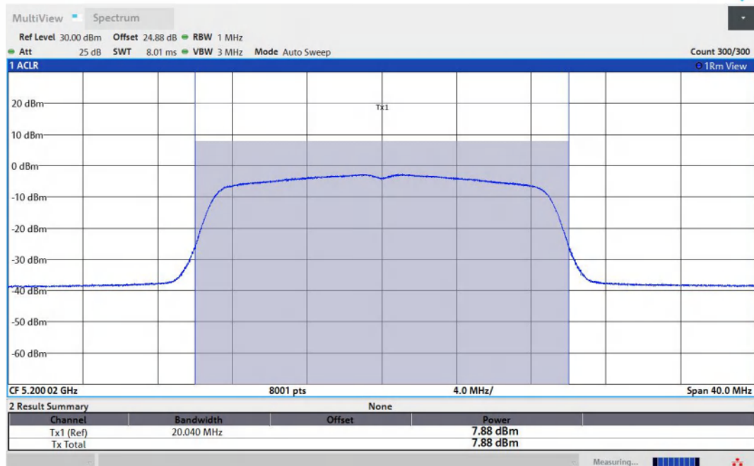
11AC20MIMO-Ant1-5200-PASS
