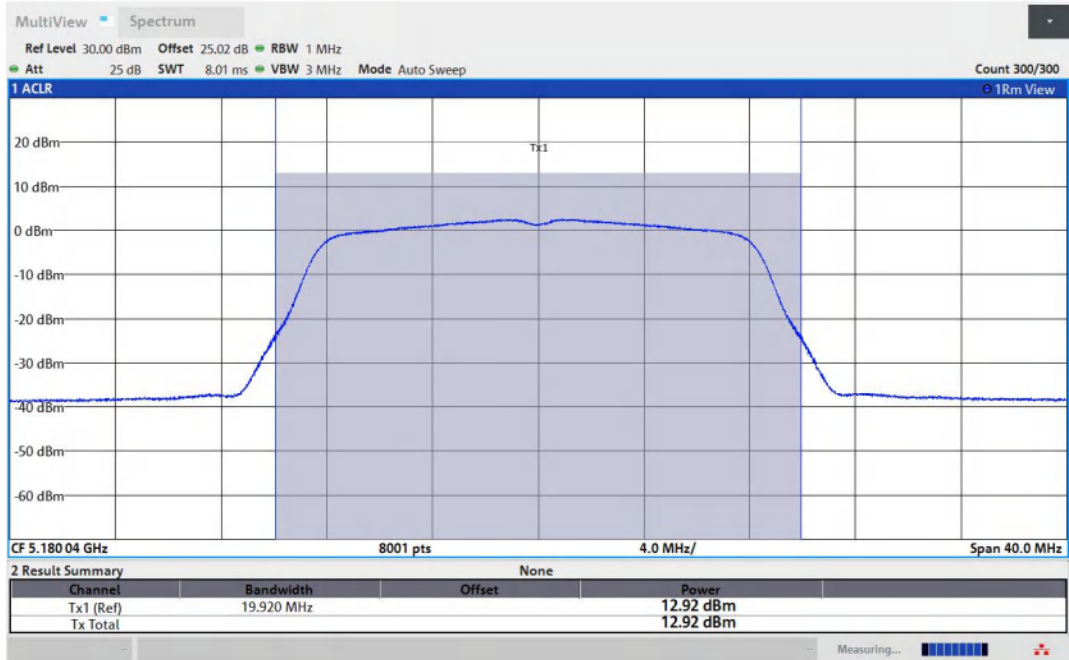
11A-Ant1-5180-PASS
