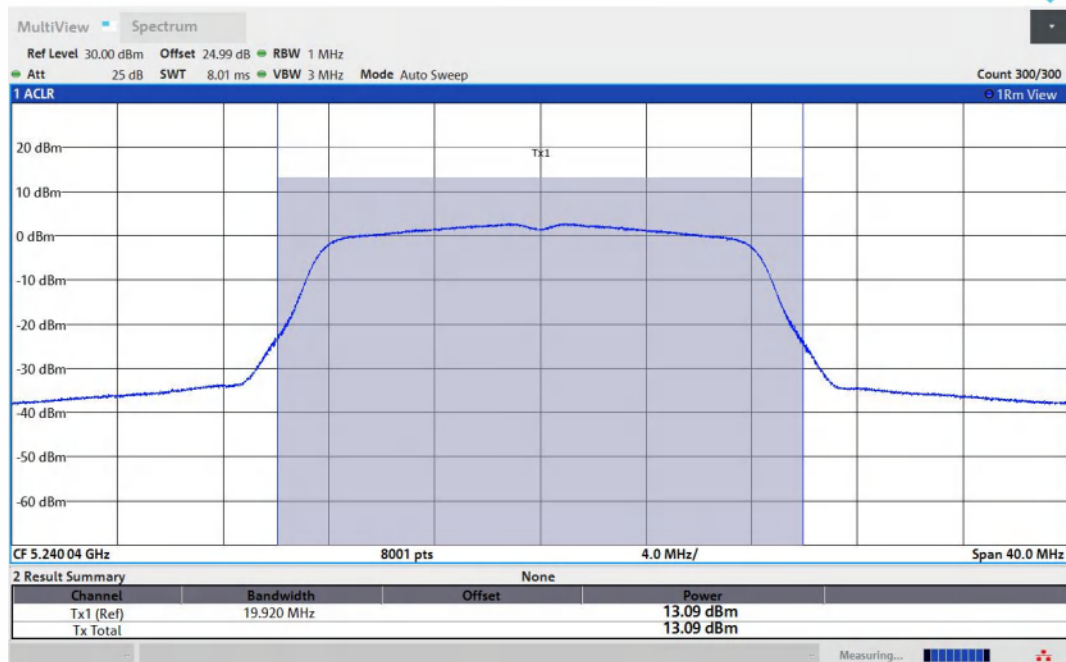
11A-Ant2-5240-PASS
