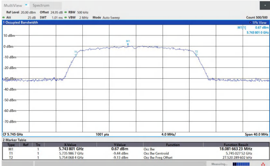
11AC20MIMO-Ant1-5745
