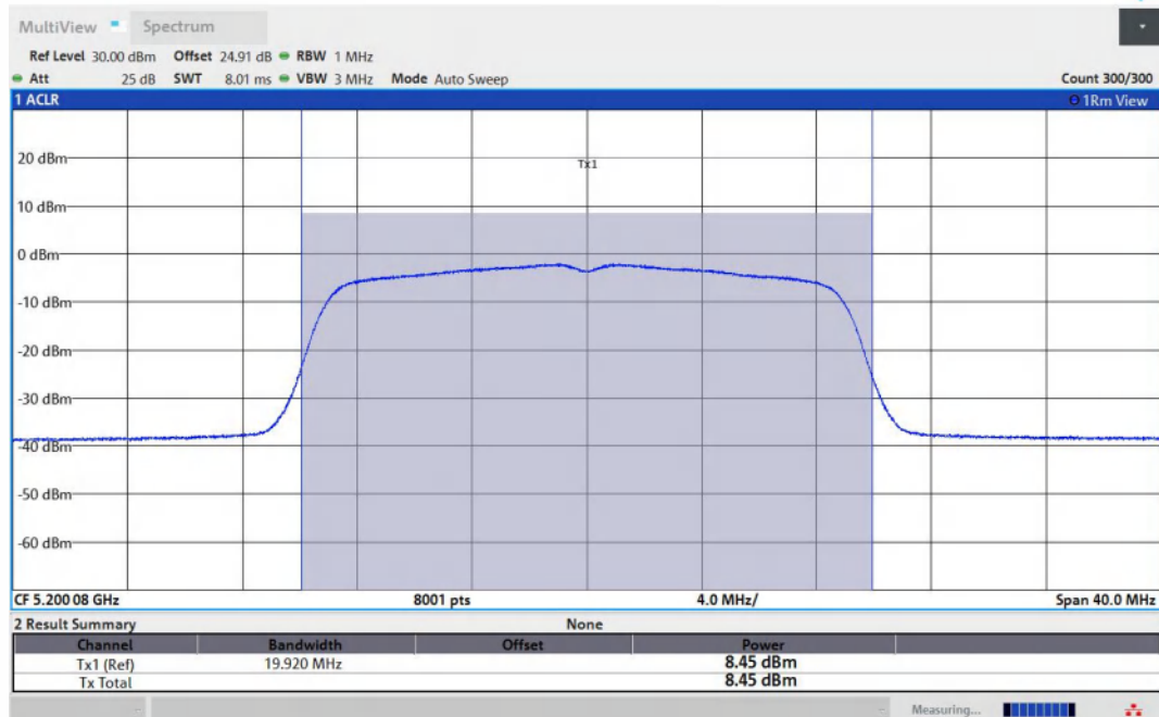
11AC20MIMO-Ant2-5200-PASS
