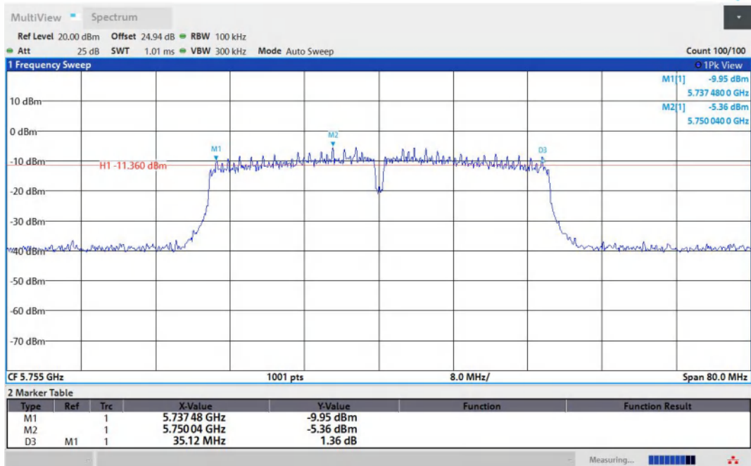
11AC40MIMO-Ant2-5755-PASS
