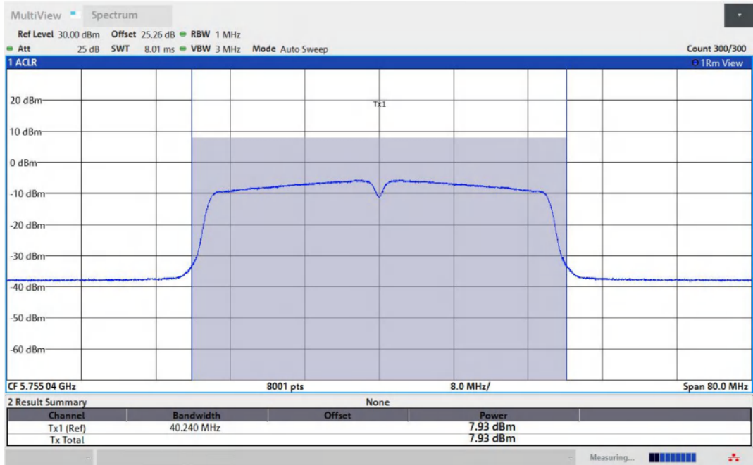
11AC40MIMO-Ant2-5755-PASS
