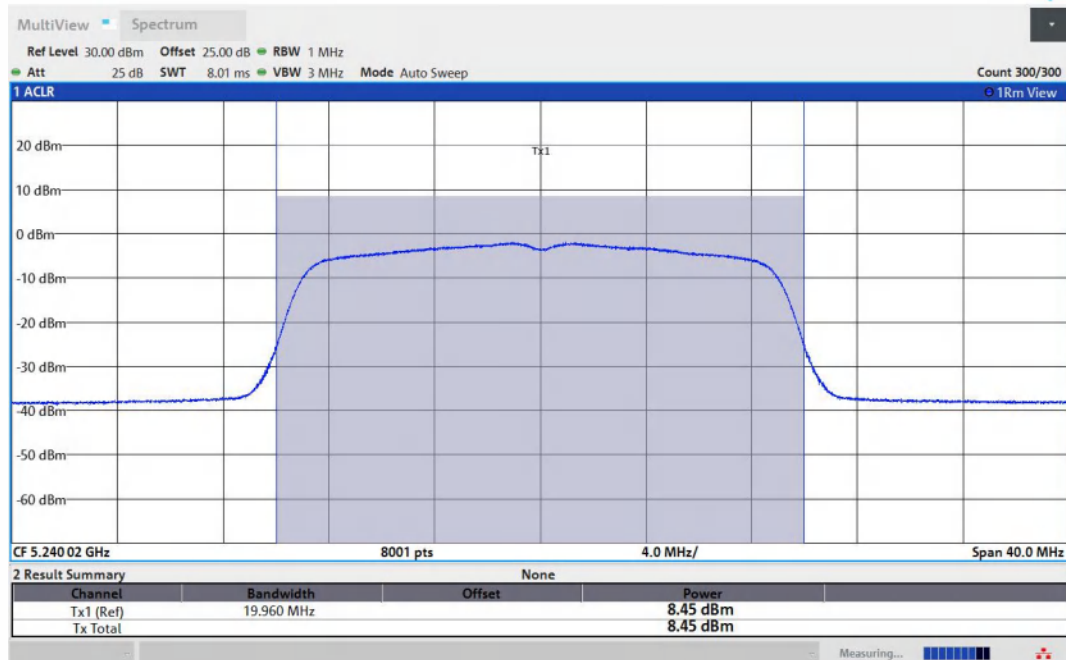
11AC20MIMO-Ant2-5240-PASS
