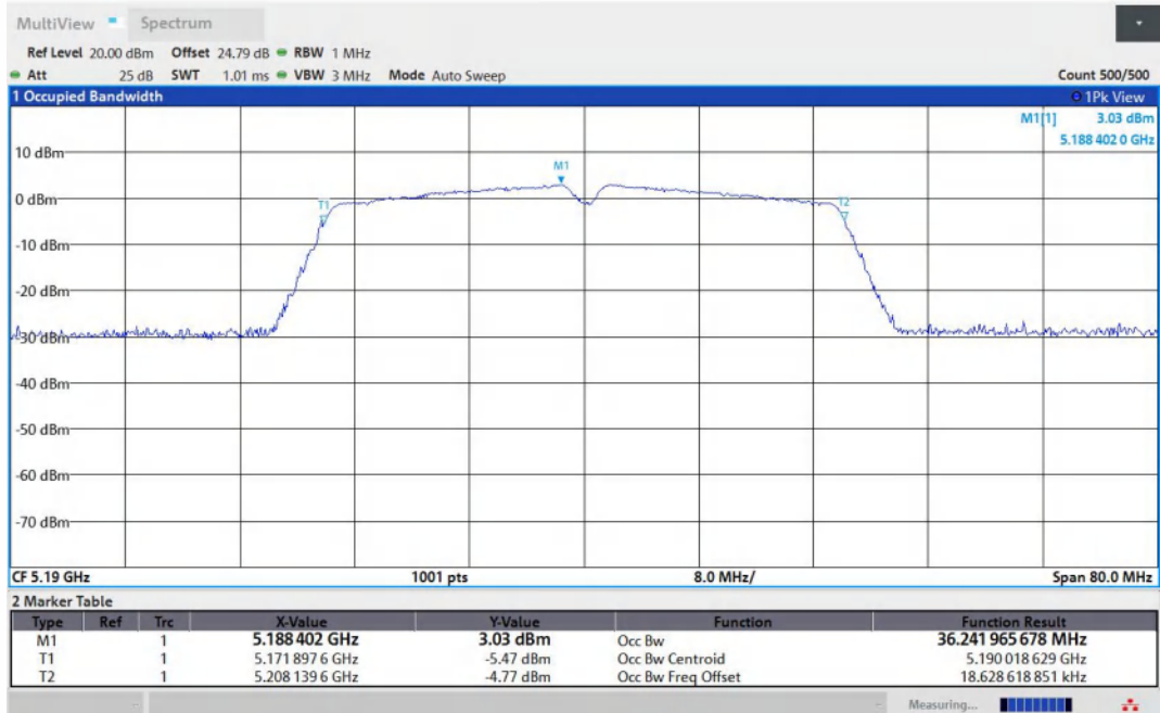
11AC40MIMO-Ant1-5190
