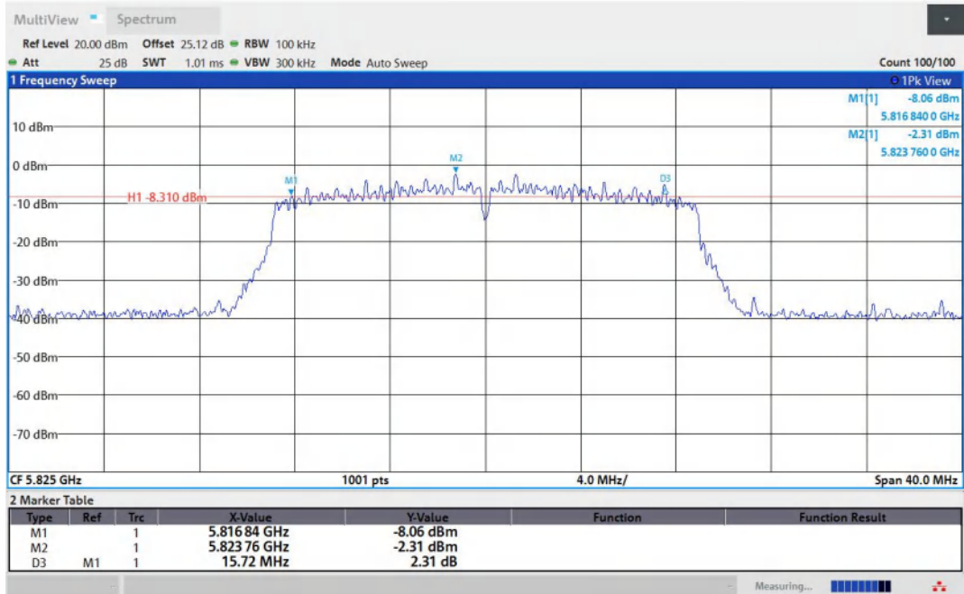
11N20MIMO-Ant2-5825-PASS
