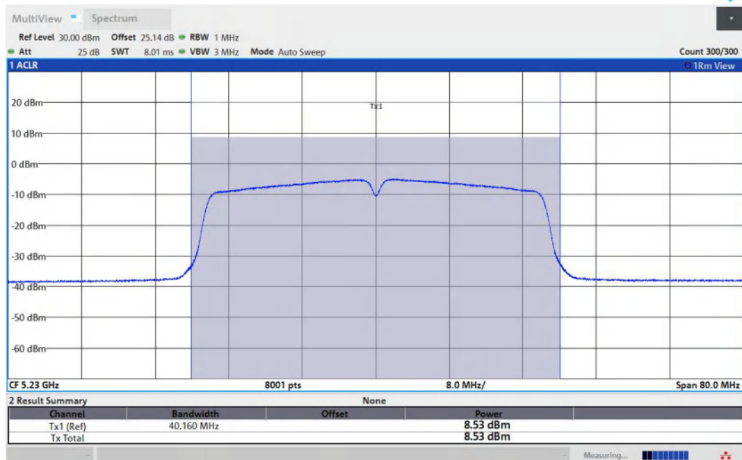
11AC40MIMO-Ant2-5230-PASS
