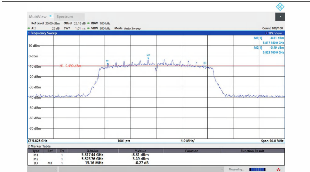
11AC20MIMO-Ant1-5825-PASS
