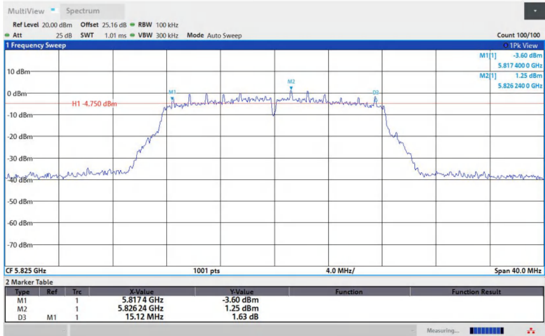
11A-Ant1-5825-PASS
