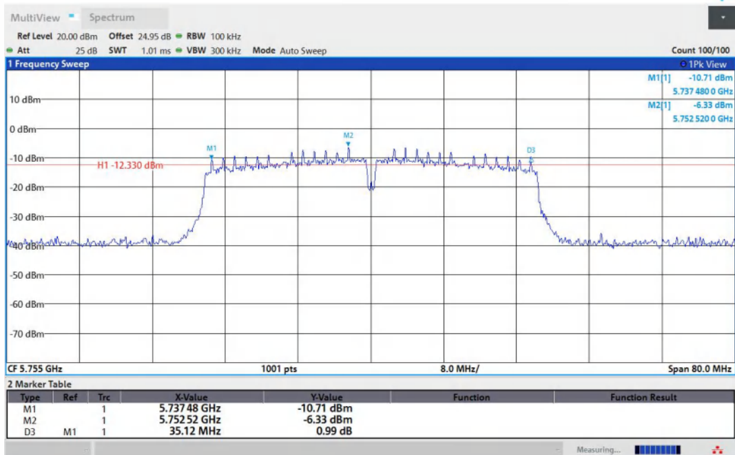
11AC40MIMO-Ant1-5755-PASS
