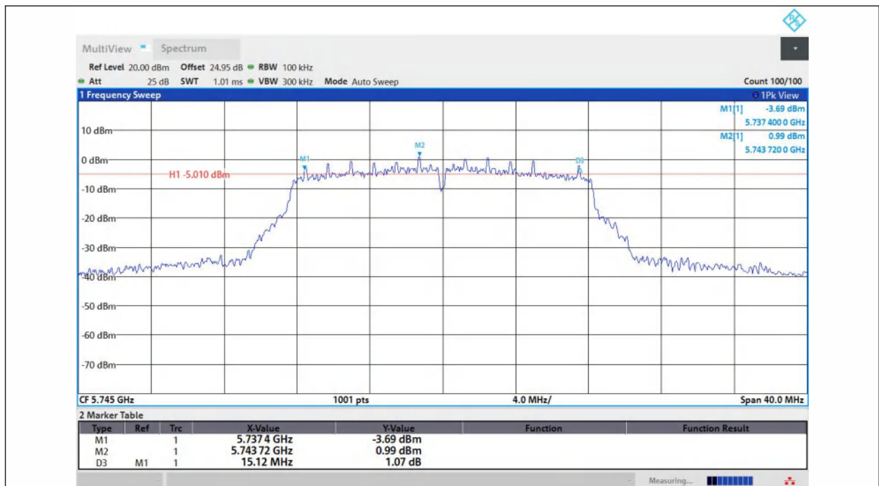
11A-Ant1-5745-PASS
