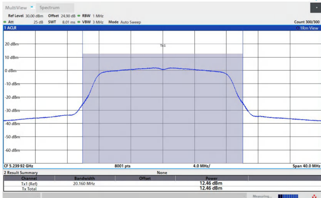
11A-Ant1-5240-PASS
