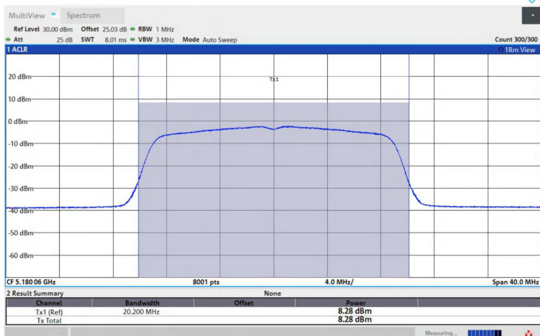
11N20MIMO-Ant1-5180-PASS
