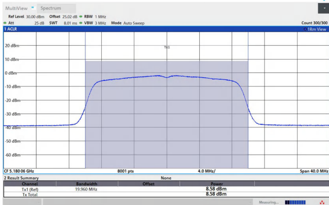
11N20MIMO-Ant2-5180-PASS
