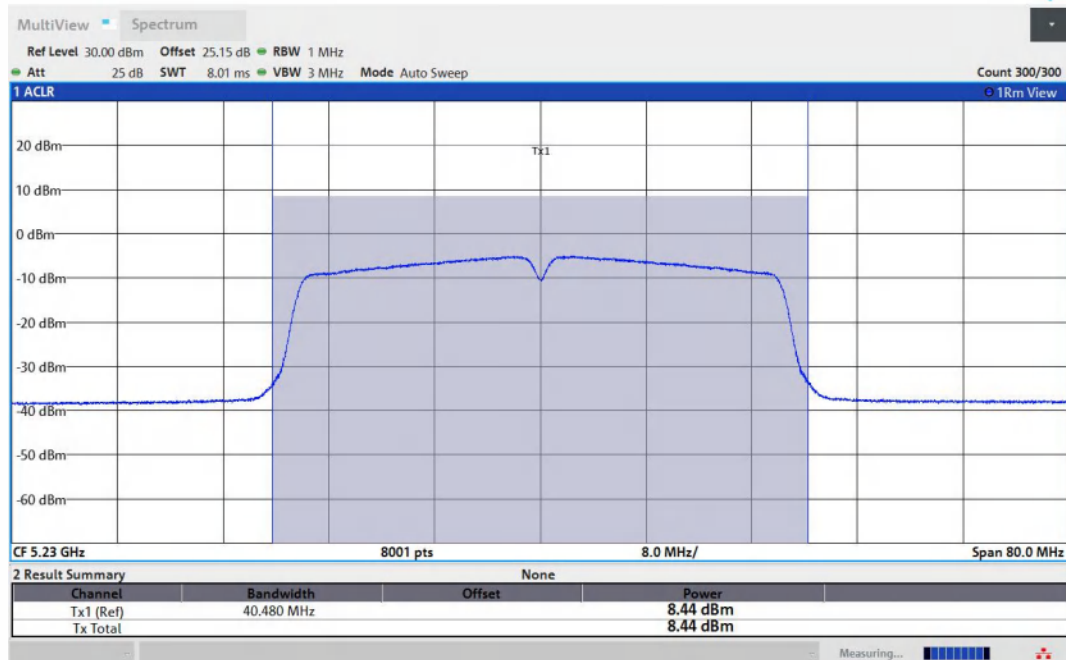
11N40MIMO-Ant2-5230-PASS
