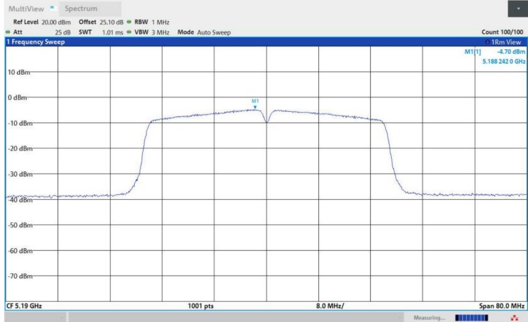
11AC40MIMO-Ant2-5190-PASS
