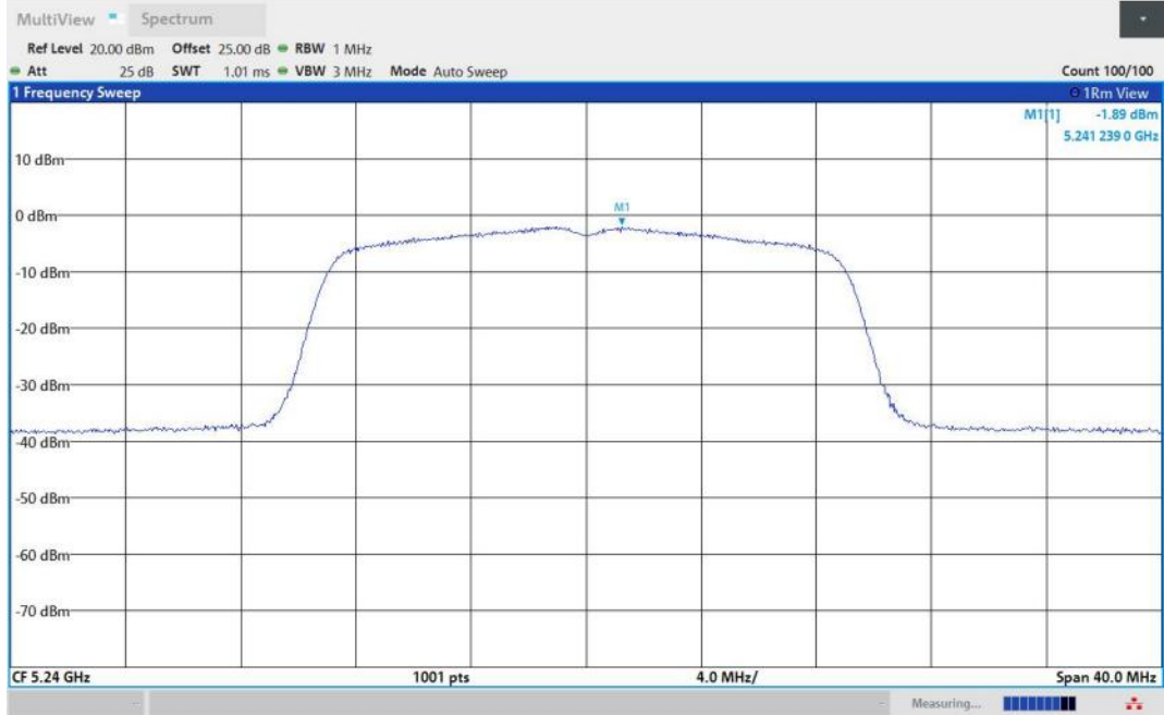
11N20MIMO-Ant2-5240-PASS
