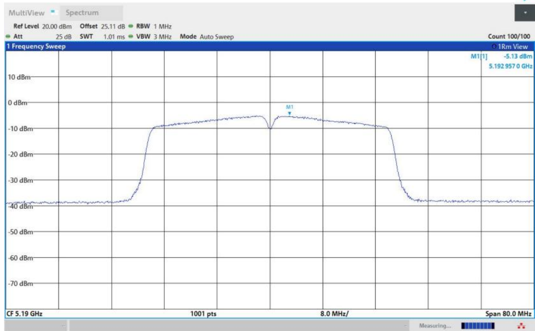
11N40MIMO-Ant1-5190-PASS
