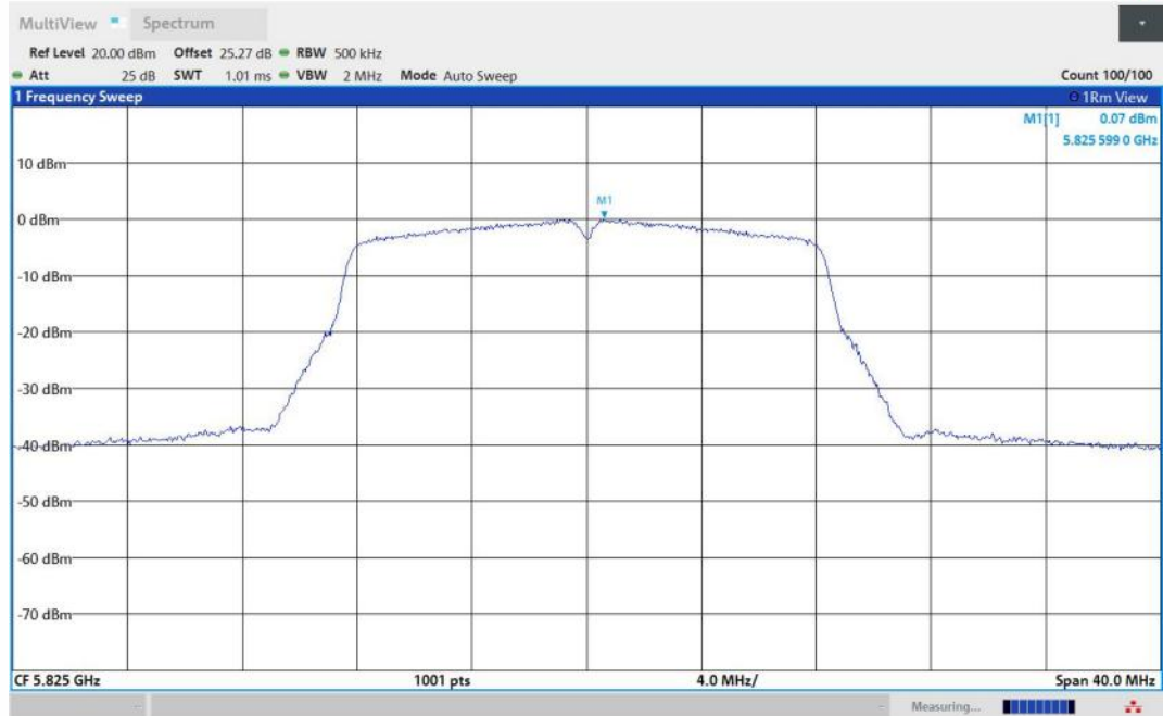
11A-Ant2-5825-PASS
