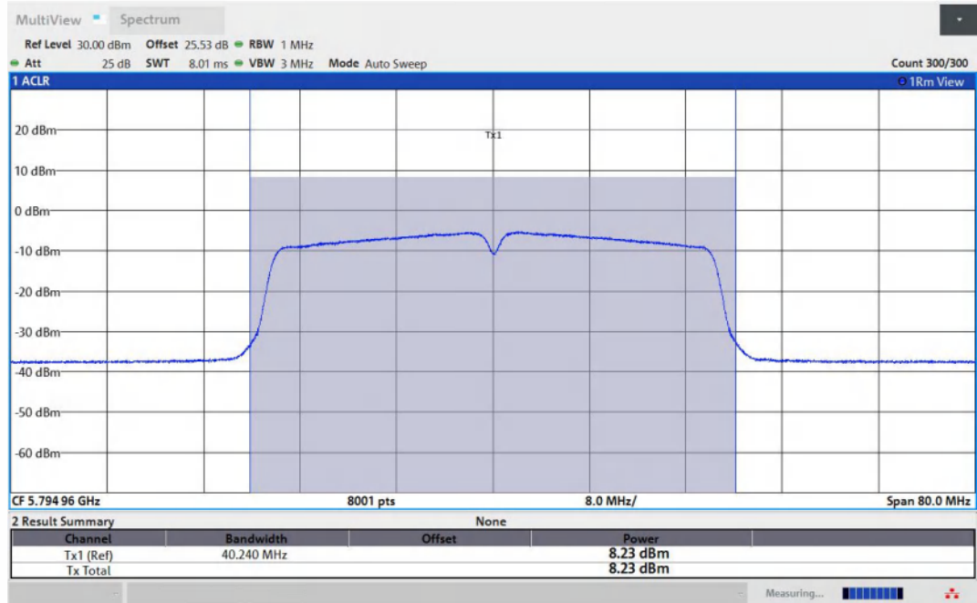
11AC40MIMO-Ant2-5795-PASS
