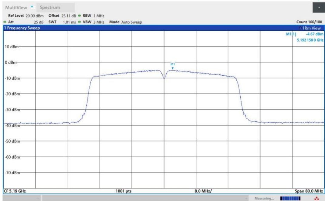
11N40MIMO-Ant2-5190-PASS
