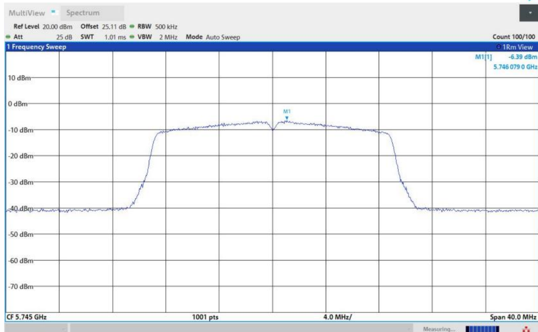
11N20MIMO-Ant1-5745-PASS
