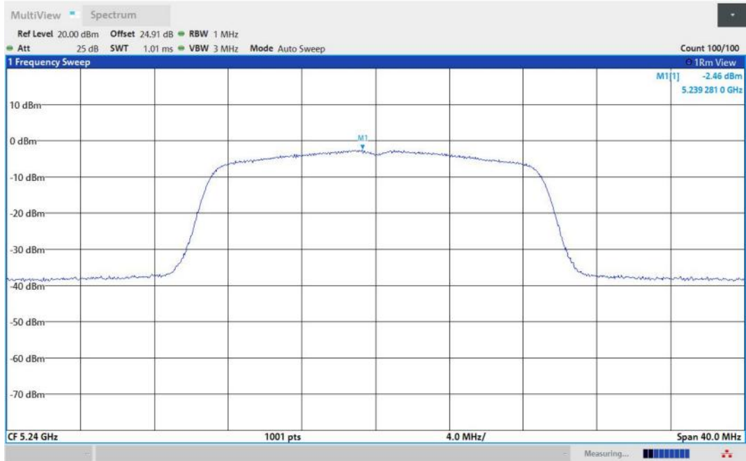
11N20MIMO-Ant1-5240-PASS
