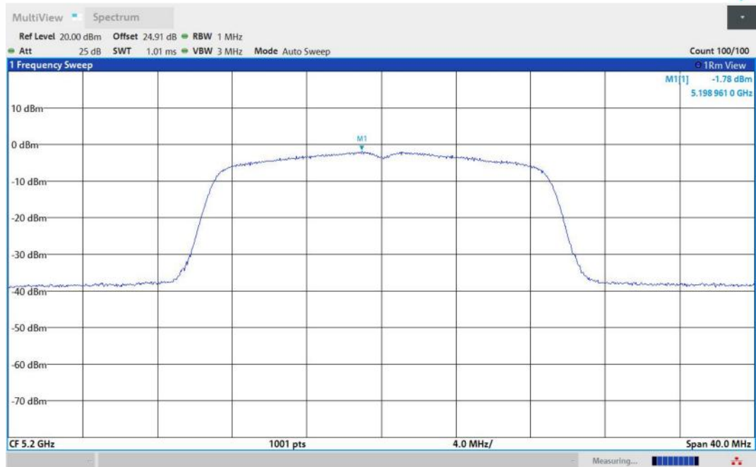
11AC20MIMO-Ant2-5200-PASS
