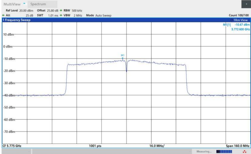
11AC80MIMO-Ant2-5775-PASS
