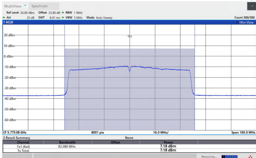
11AC80MIMO-Ant1-5775-PASS
