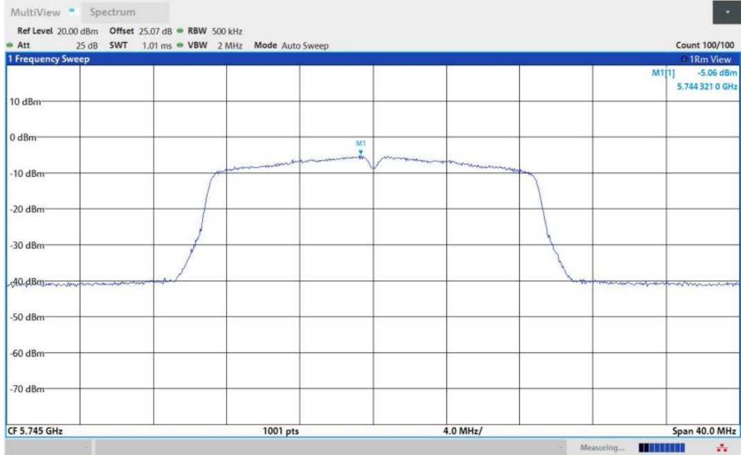
11AC20MIMO-Ant2-5745-PASS
