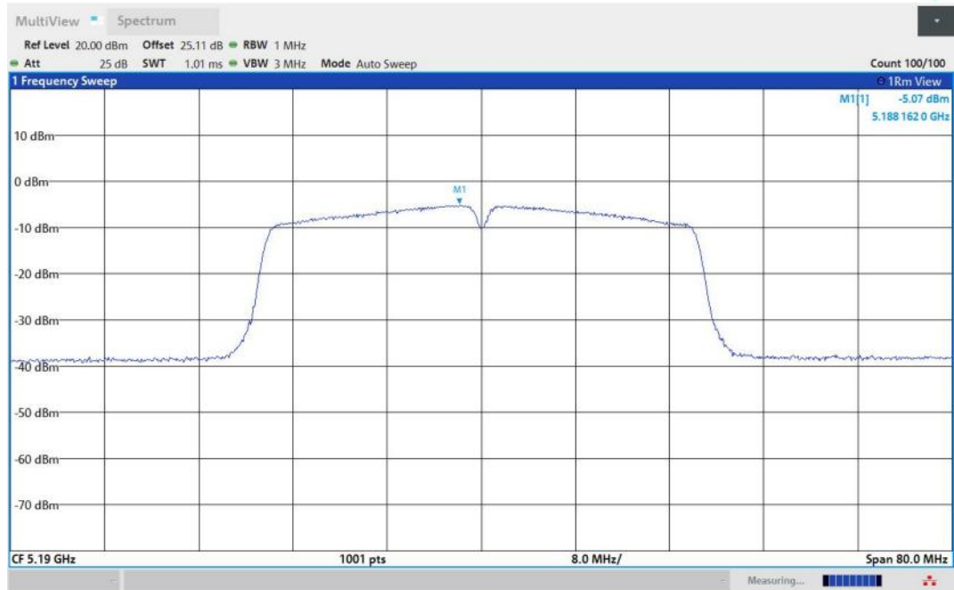
11AC40MIMO-Ant1-5190-PASS
