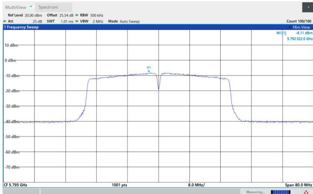
11N40MIMO-Ant2-5795-PASS
