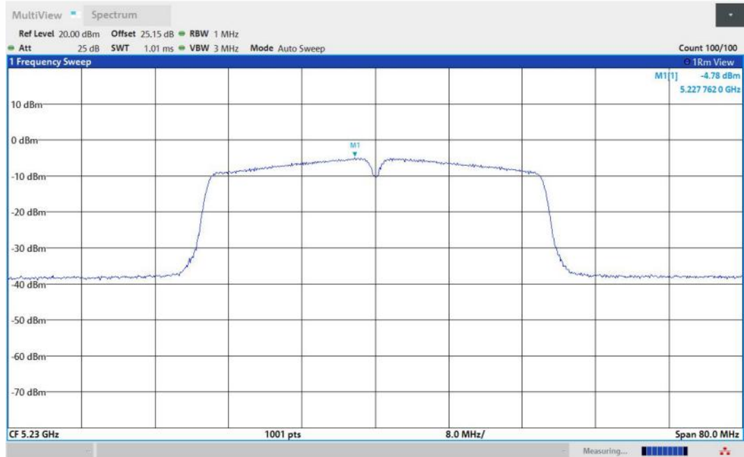
11N40MIMO-Ant2-5230-PASS
