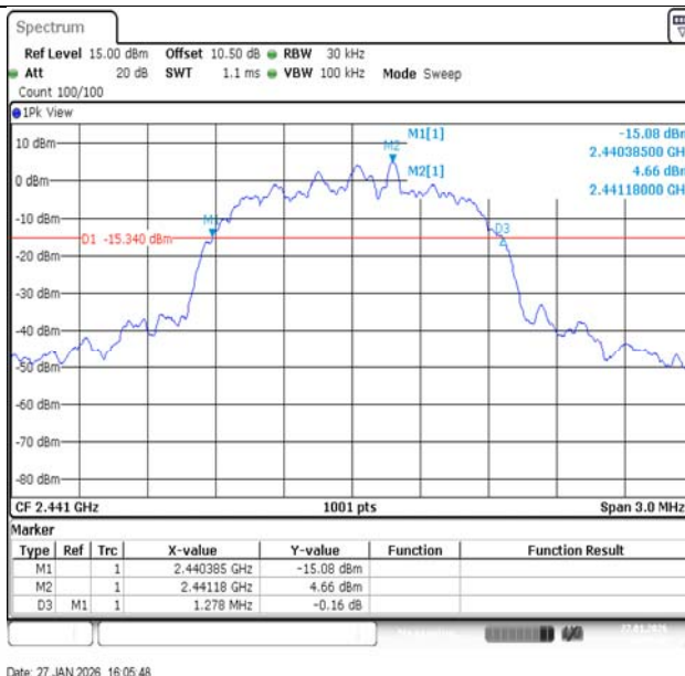
2DH5-Ant1-2441
