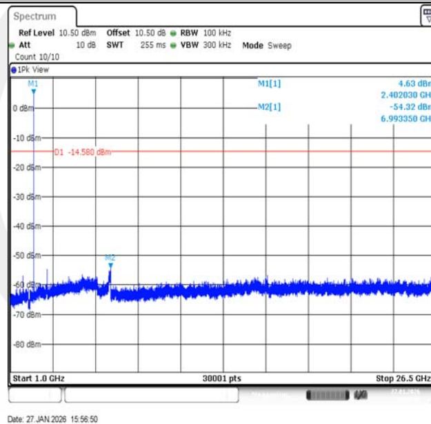
DH5-Ant1-2402-1000~26500-PASS
