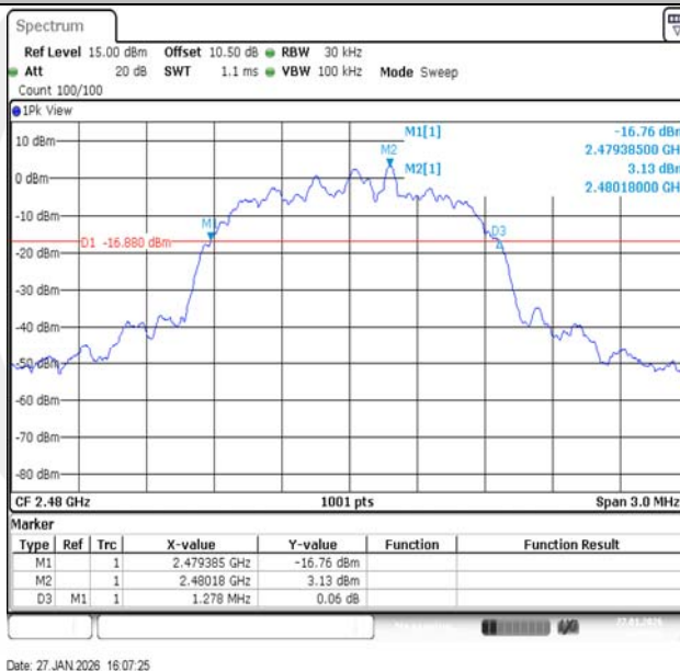
2DH5-Ant1-2480
