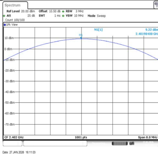
3DH5-Ant1-2402-PASS
