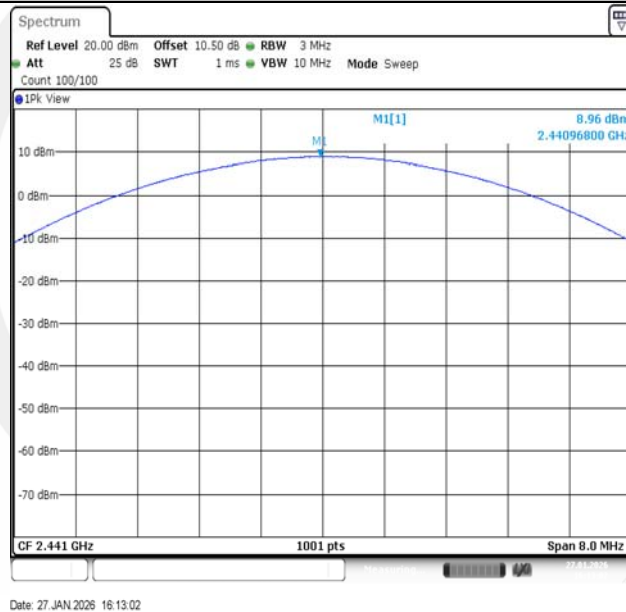
3DH5-Ant1-2441-PASS
