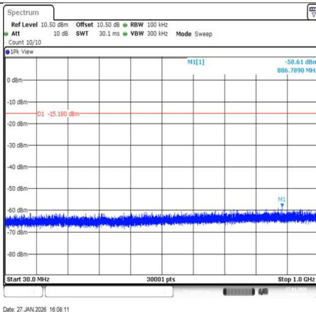
2DH5-Ant1-2480-30~1000-PASS
