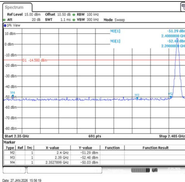
DH5-Ant1-2402-PASS
