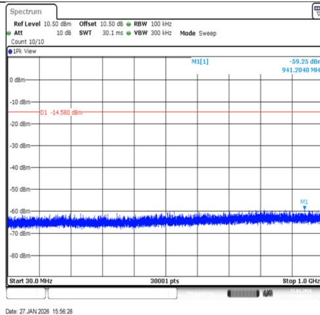
DH5-Ant1-2402-30~1000-PASS
