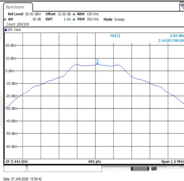
DH5-Ant1-2441-PASS
