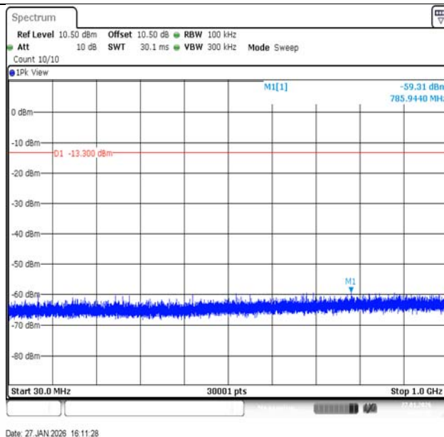
3DH5-Ant1-2402-30~1000-PASS
