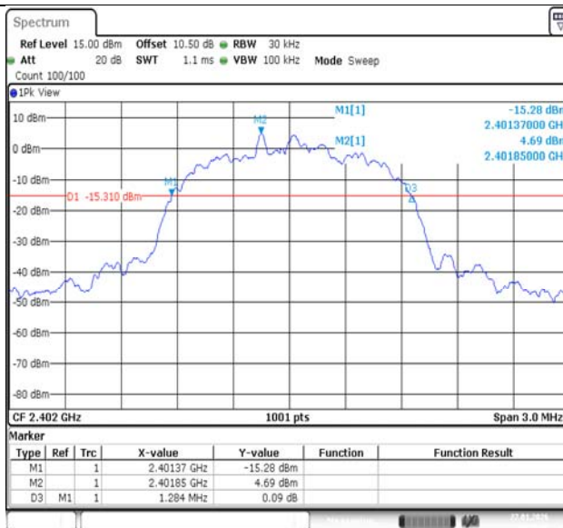
3DH5-Ant1-2402
