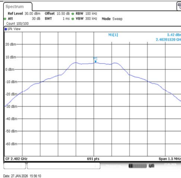
DH5-Ant1-2402-PASS
