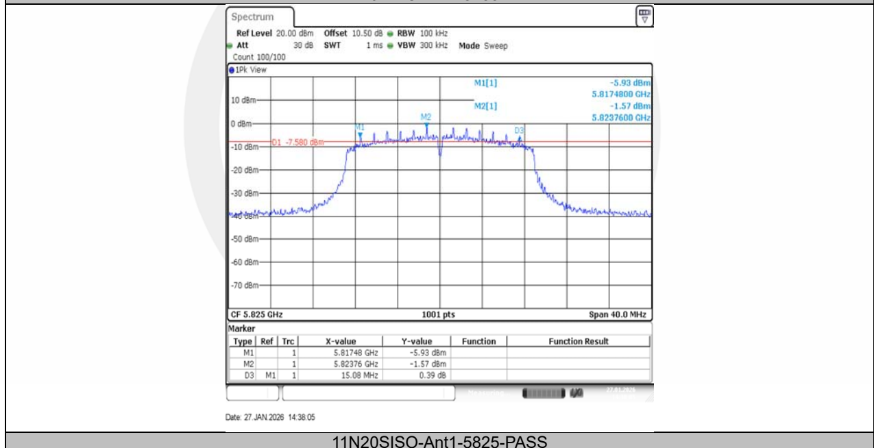
11N20SISO-Ant1-5825-PASS
