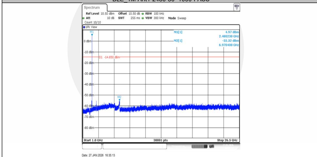
BLE_1M-Ant1-2480-1000~26500-PASS
