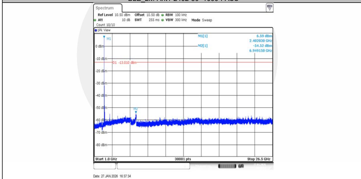
BLE_2M-Ant1-2402-1000~26500-PASS
