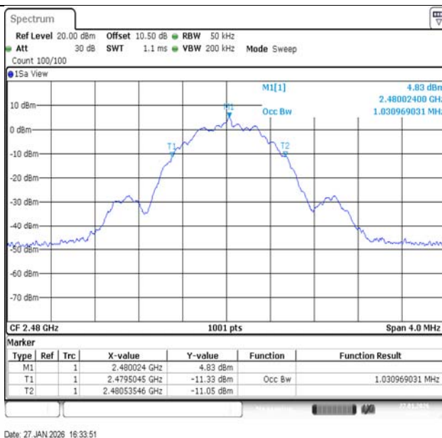
BLE_1M-Ant1-2480
