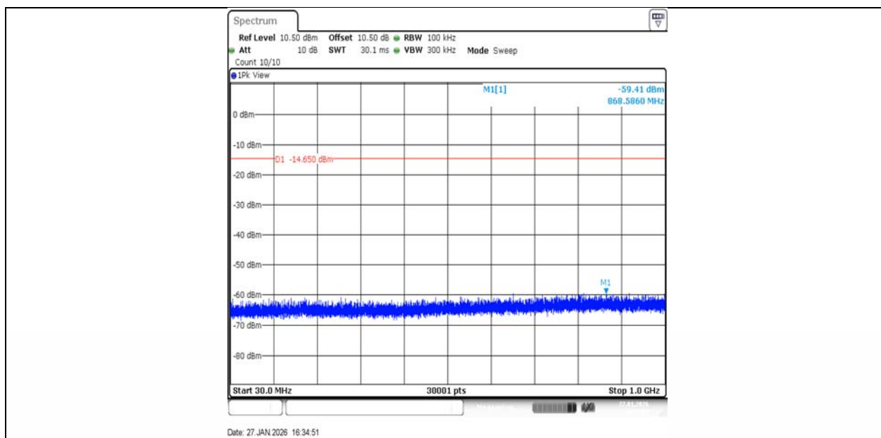
BLE_1M-Ant1-2480-30~1000-PASS
