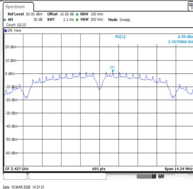
11B-Ant1-2437-PASS
