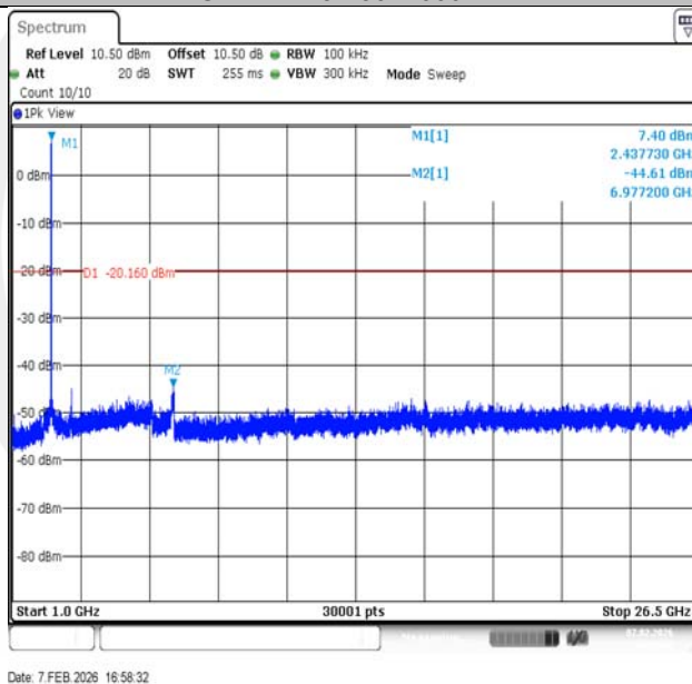
11G-Ant1-2437-1000~26500-PASS
