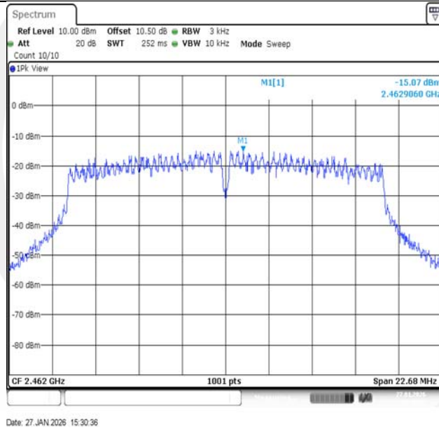
11G-Ant1-2462-PASS
