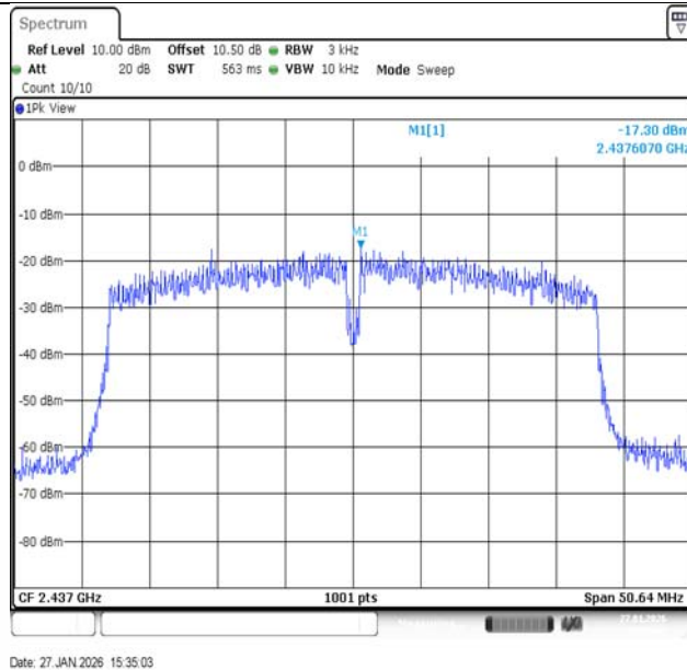
11N40SISO-Ant1-2437-PASS
