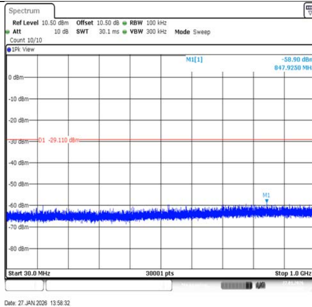
11B-Ant1-2462-30~1000-PASS
