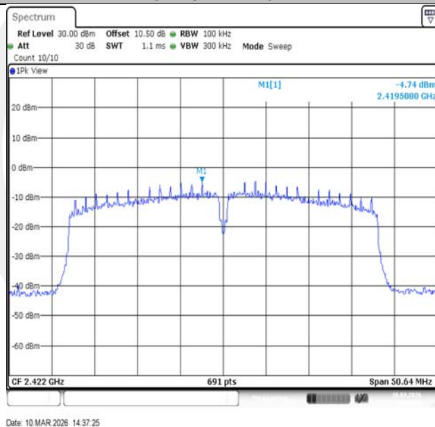
11N40SISO-Ant1-2422-PASS
