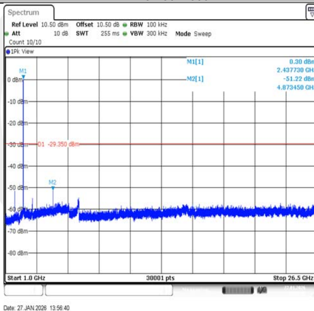
11B-Ant1-2437-1000~26500-PASS
