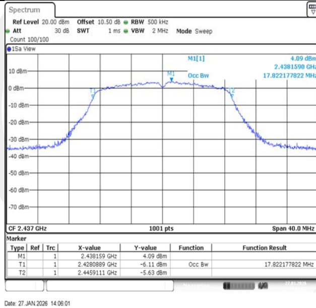
11N20SISO-Ant1-2437
