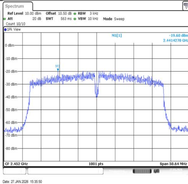
11N40SISO-Ant1-2452-PASS
