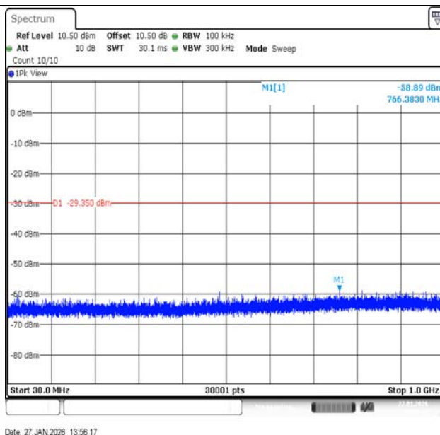
11B-Ant1-2437-30~1000-PASS
