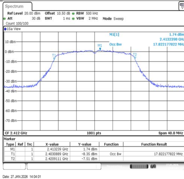
11N20SISO-Ant1-2412
