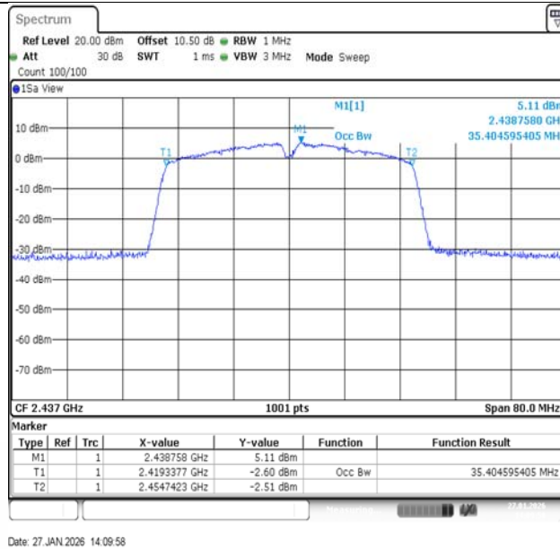
11N40SISO-Ant1-2437
