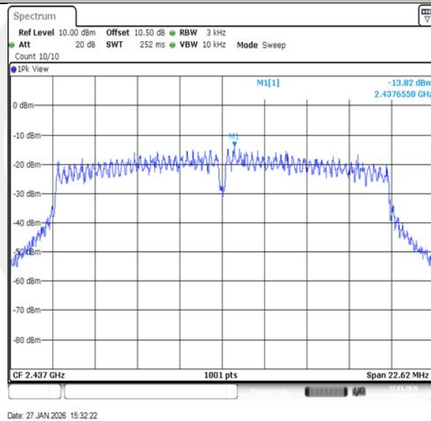
11N20SISO-Ant1-2437-PASS
