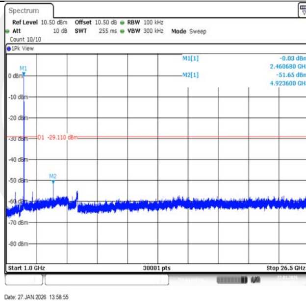
11B-Ant1-2462-1000~26500-PASS
