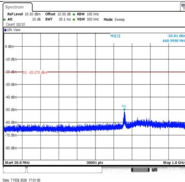
11N20SISO-Ant1-2437-30~1000-PASS
