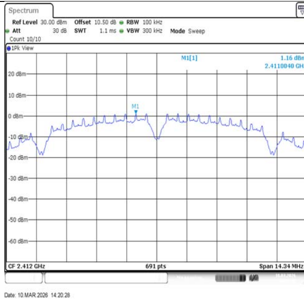
11B-Ant1-2412-PASS
