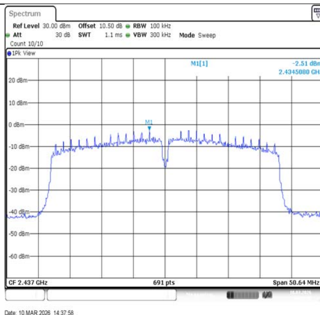
11N40SISO-Ant1-2437-PASS
