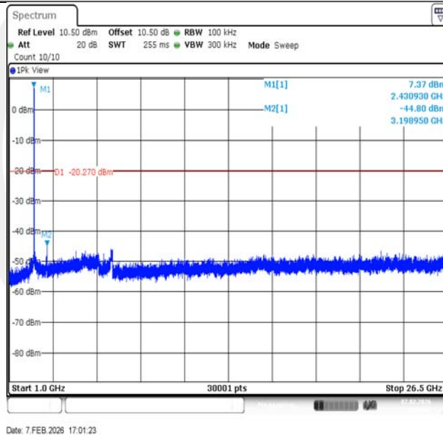
11N20SISO-Ant1-2437-1000~26500-PASS
