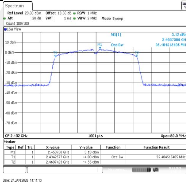
11N40SISO-Ant1-2452
