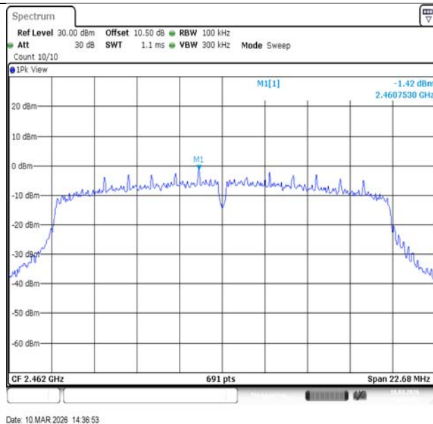
11N20SISO-Ant1-2462-PASS
