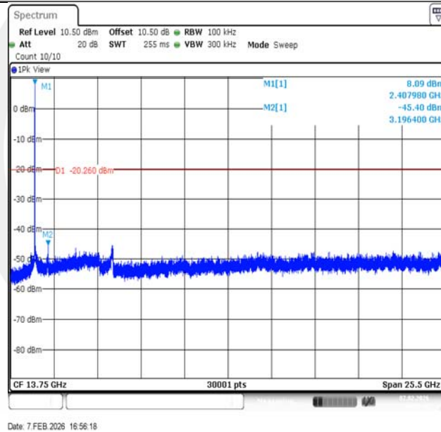
11G-Ant1-2412-1000~26500-PASS
