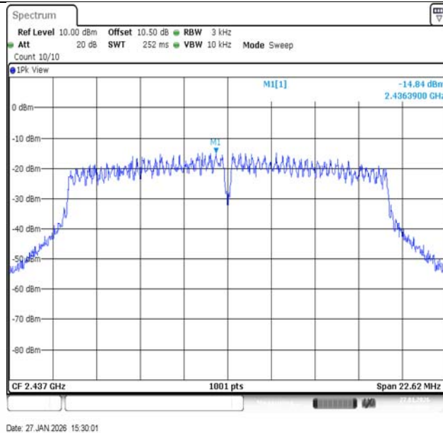
11G-Ant1-2437-PASS
