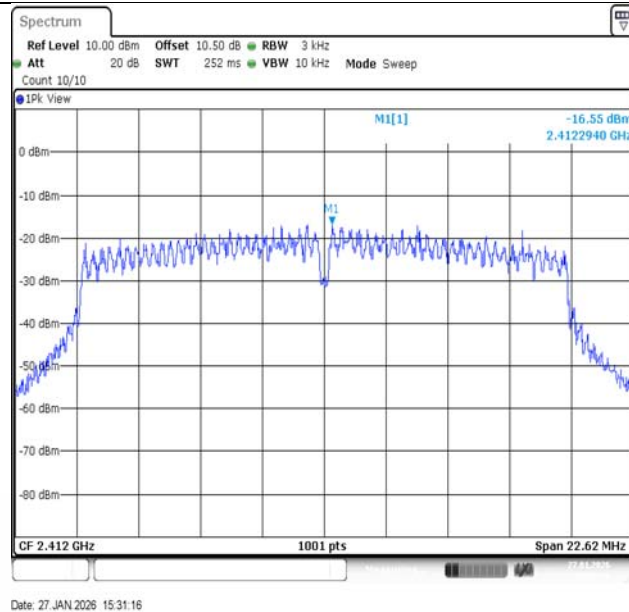
11N20SISO-Ant1-2412-PASS
