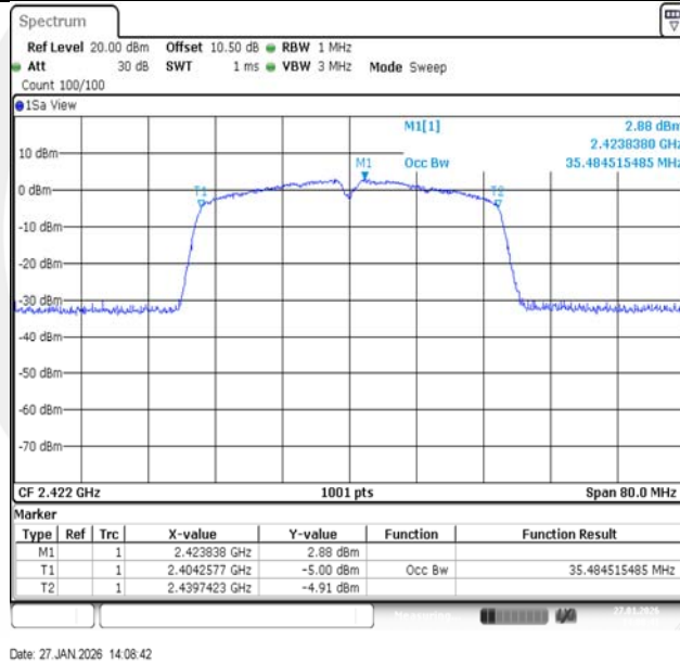
11N40SISO-Ant1-2422
