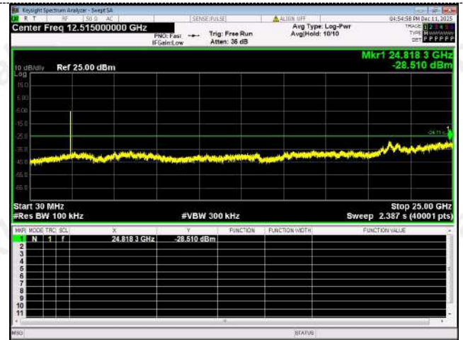
30.0 MHz - 25000.0 MHz
