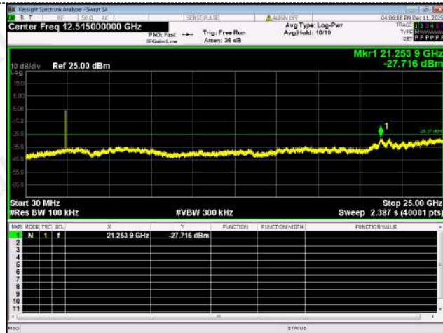
30.0 MHz - 25000.0 MHz
