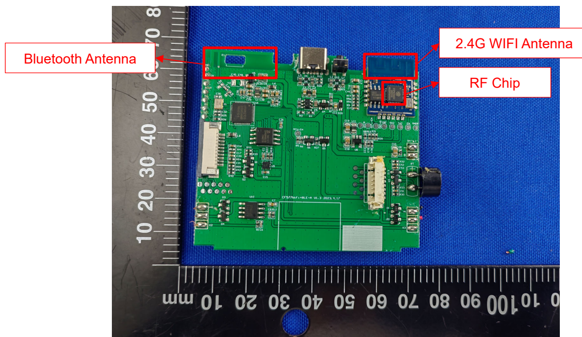
MAIN BOARD TOP VIEW (WITHOUT SHIELDING)
