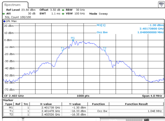
BLE_1M_Low_Channel
