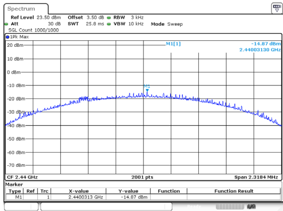
BLE_2M_Middle_Channel
