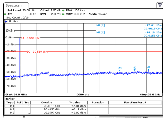
BLE_2M_Low_Channel
