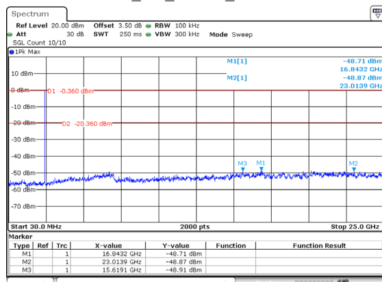
BLE_2M_Middle_Channel
