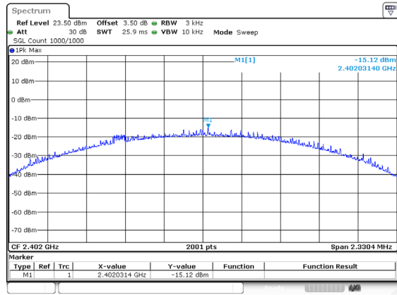
BLE_2M_Low_Channel
