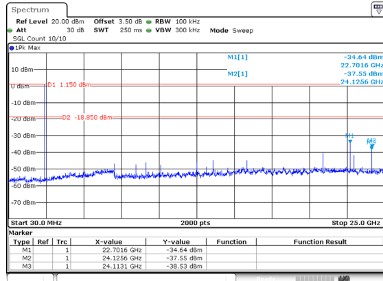
BLE_1M_Low_Channel
