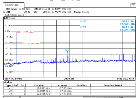
BLE_2M_High_Channel
