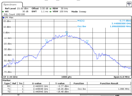
BLE_2M_Middle_Channel
