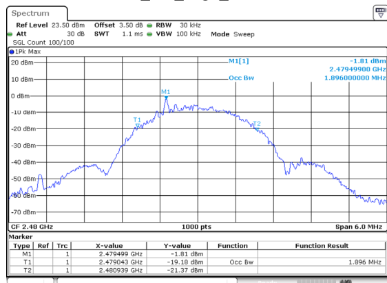
BLE_2M_High_Channel
