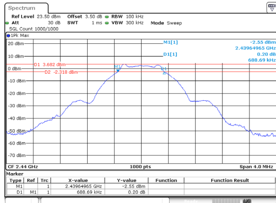
BLE_1M_Middle_Channel
