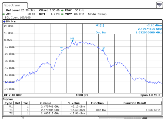
BLE_1M_High_Channel
