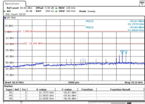
BLE_1M_Middle_Channel
