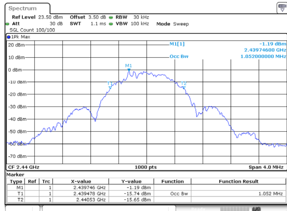
BLE_1M_Middle_Channel
