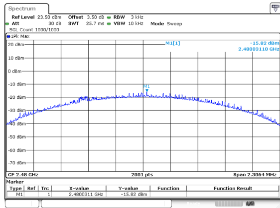
BLE_2M_High_Channel
