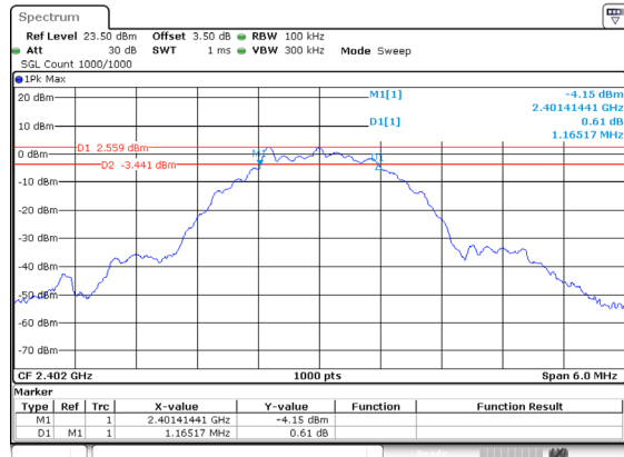
BLE_2M_Low_Channel
