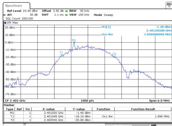
BLE_2M_Low_Channel
