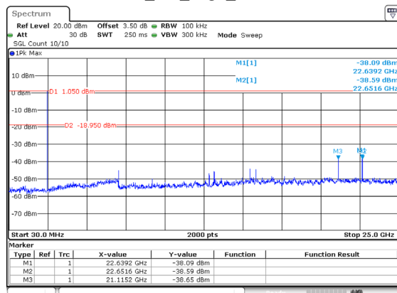
BLE_1M_High_Channel
