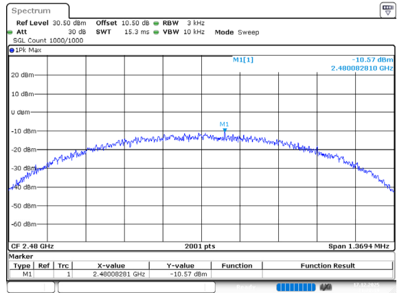
BLE_1M_High_Channel
