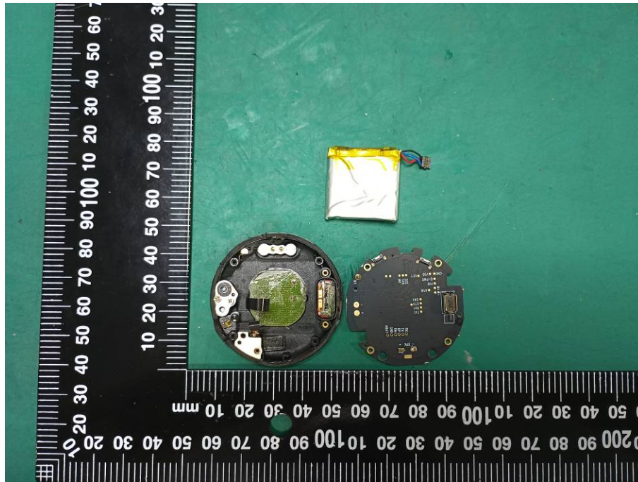
Ant-BT&BLE
