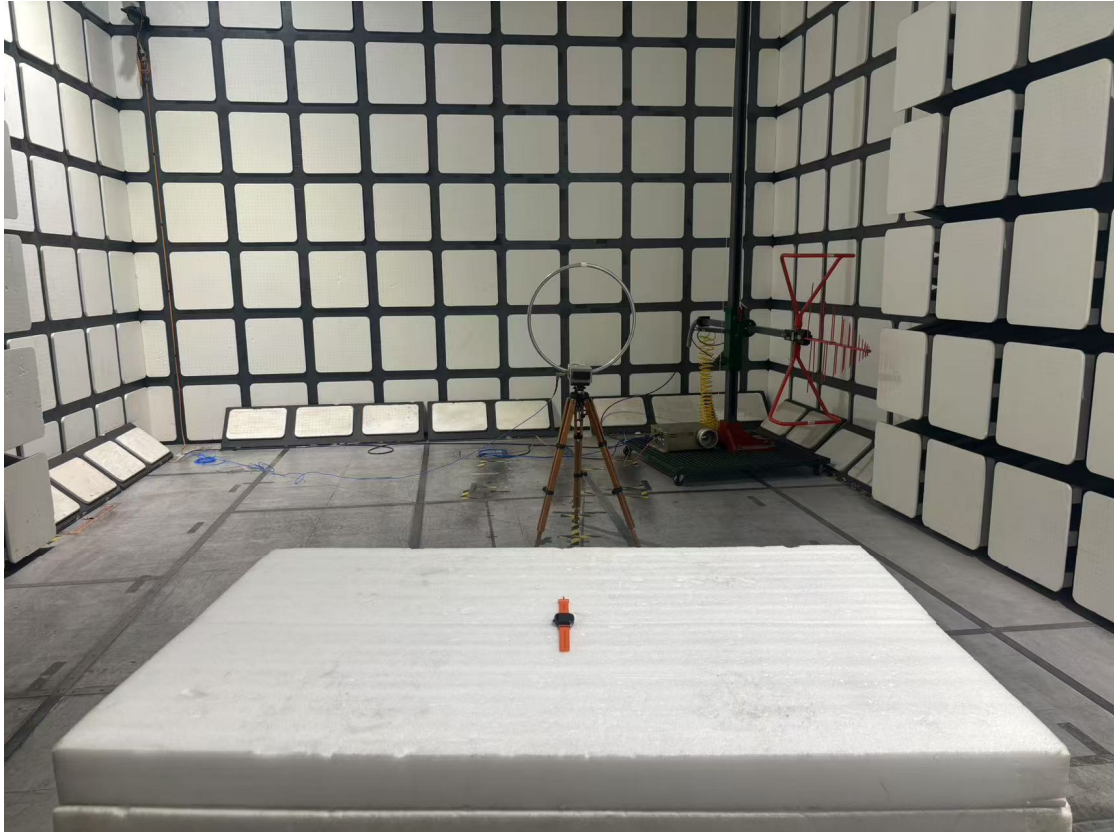
Radiated Emissions View (9 kHz- 30MHz)
