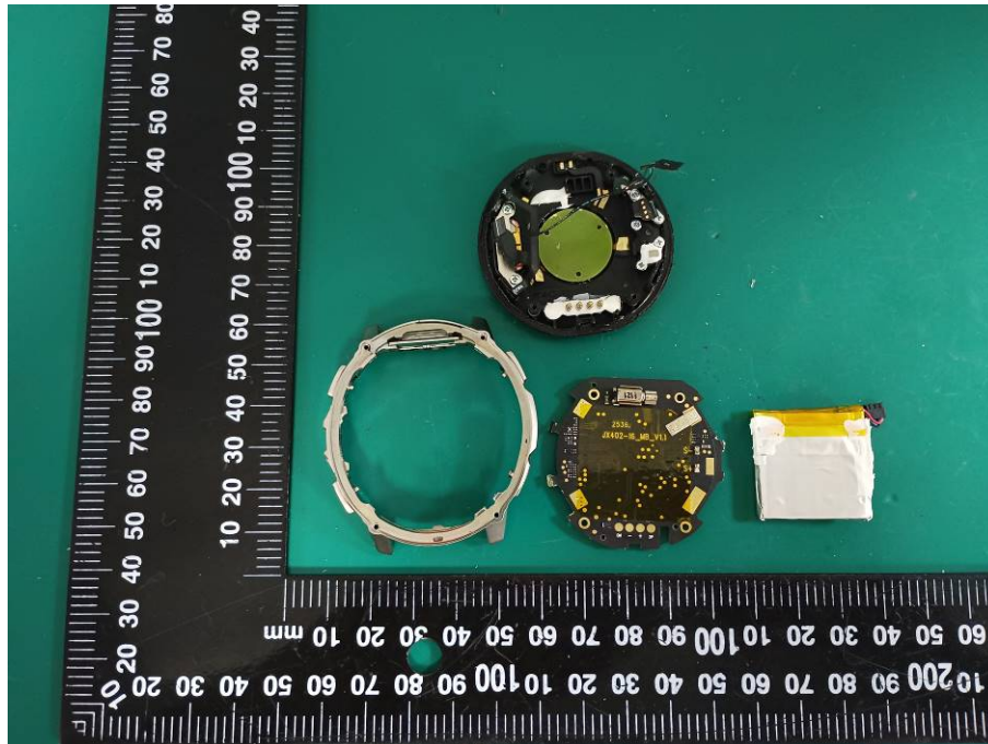
BT/BLE Antenna
