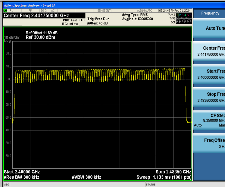
DH5-Ant2-Hop-PASS
