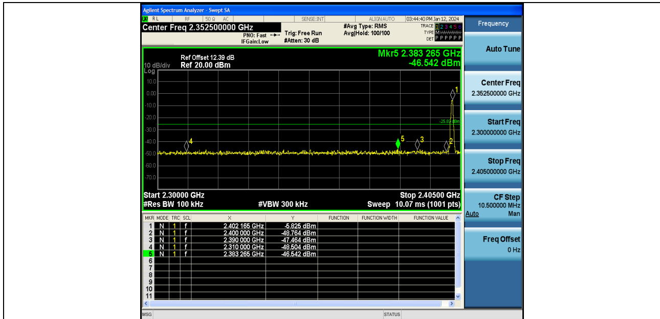
DH5-Ant1-2402-PASS
