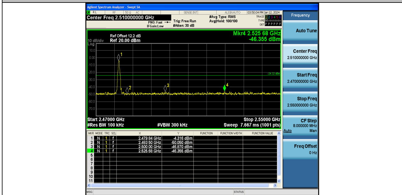
DH5-Ant1-2480-PASS
