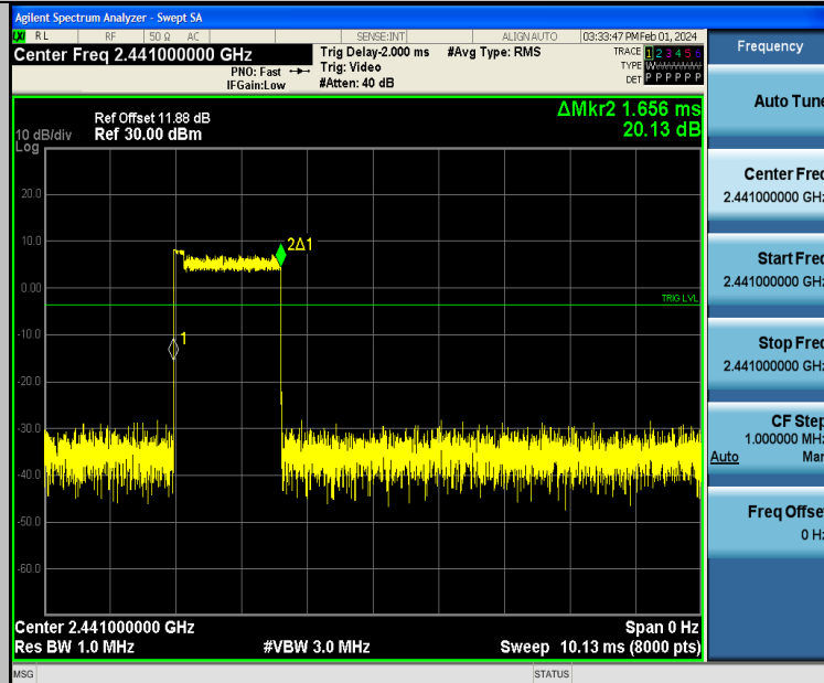
3DH3-Ant2-Hop-PASS
