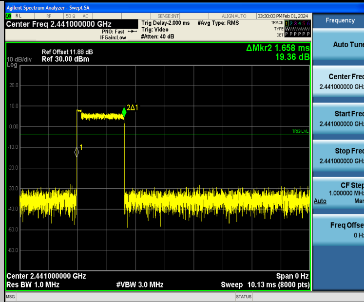
2DH3-Ant2-Hop-PASS
