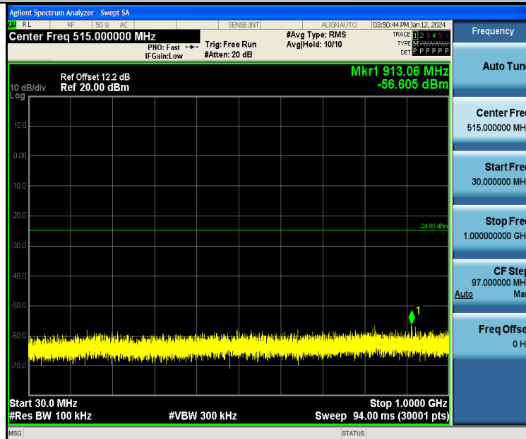
DH5-Ant1-2480-30~1000-PASS
