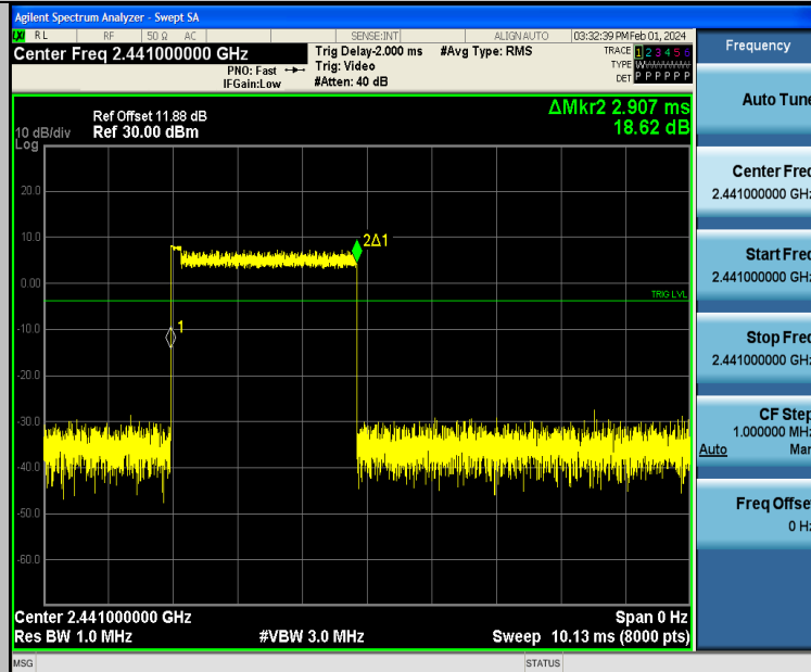
3DH5-Ant2-Hop-PASS
