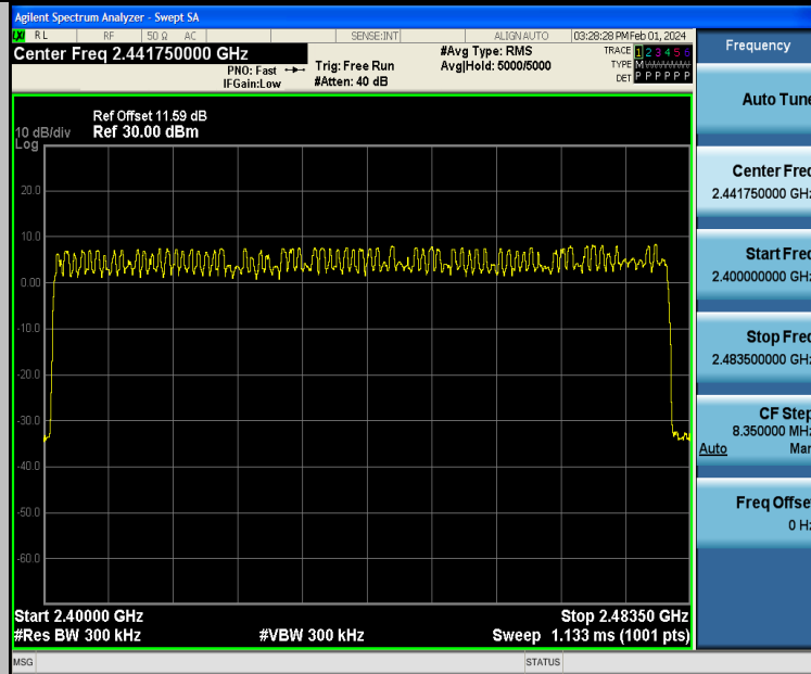
2DH5-Ant2-Hop-PASS
