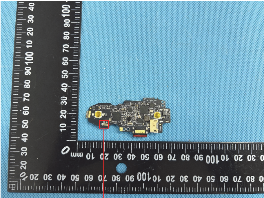
BT(BR/EDR/BLE)_A Ant.
