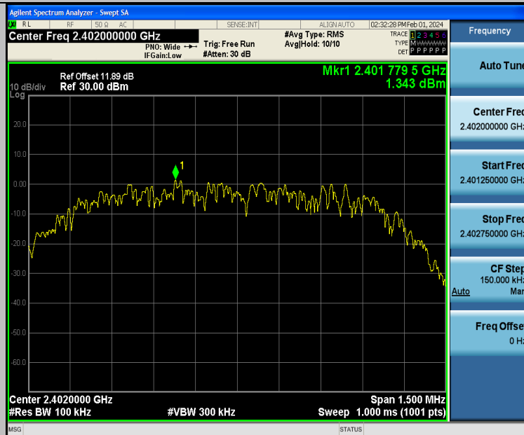
3DH5-Ant2-2402-0~Reference-PASS
