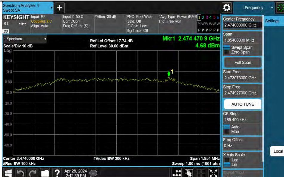
GFSK-Ant1-2474-PASS
