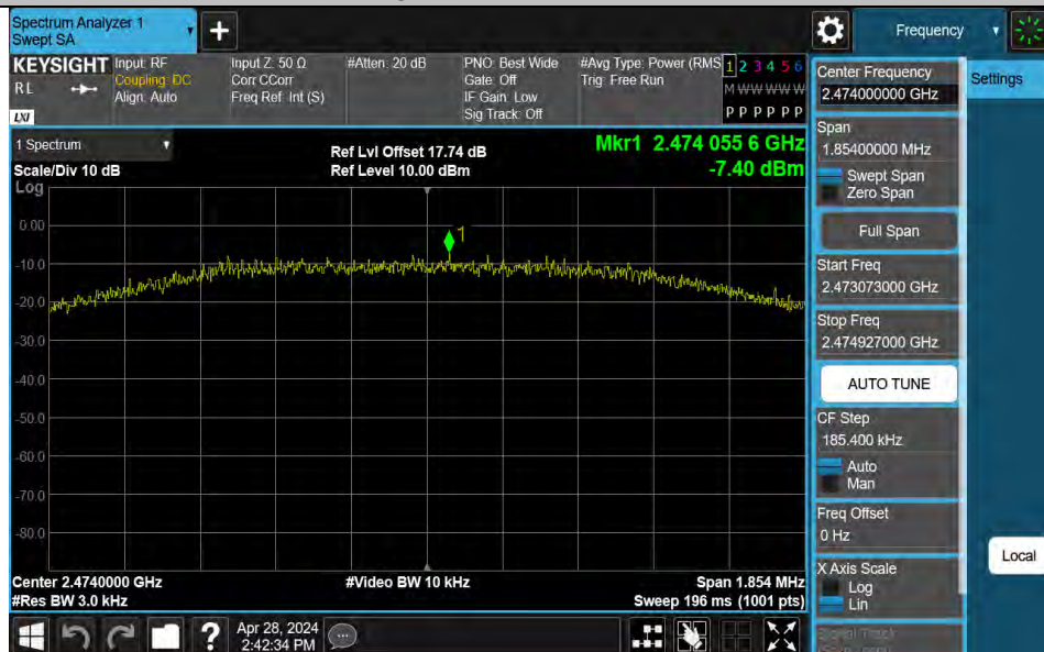
GFSK-Ant1-2474-PASS
