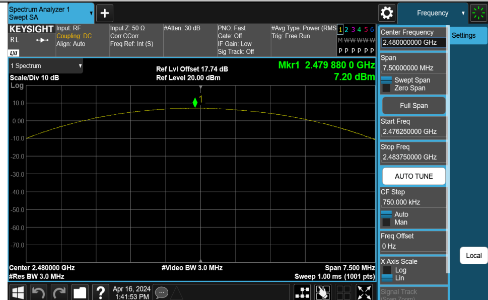
DH5-Ant1-2480-PASS
