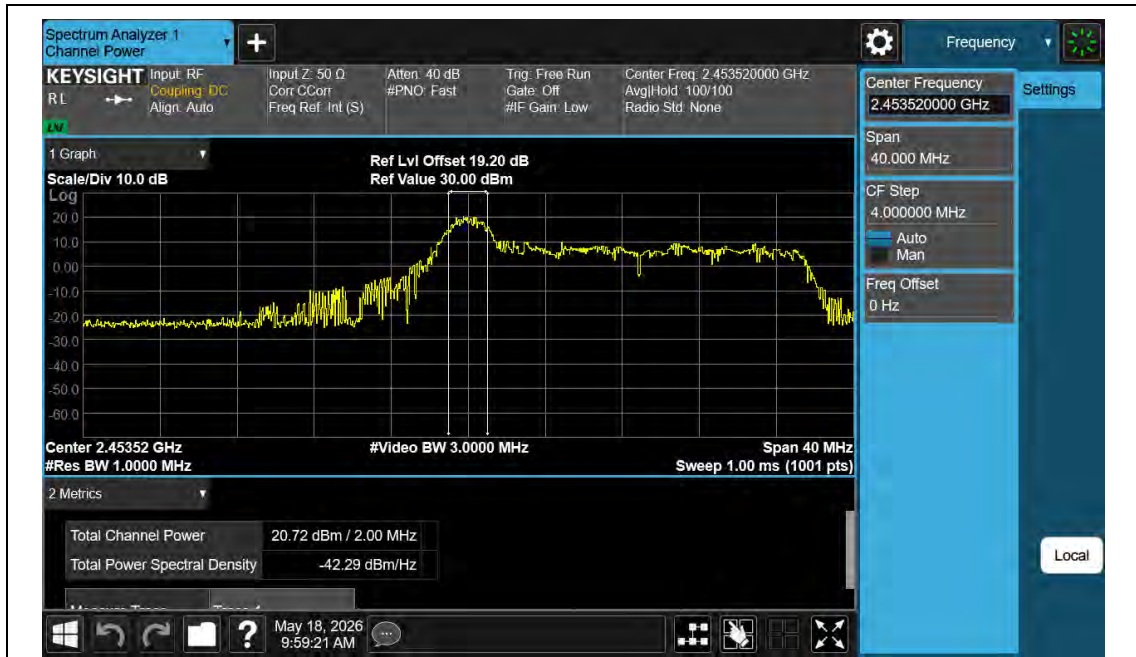
11AX20MIMO-Ant1-2462-26Tone-RU0-PASS
