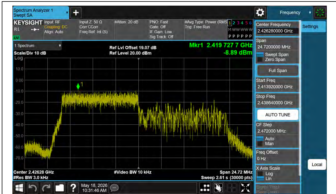
11AX40MIMO-Ant1-2437-106Tone-RU53-PASS
