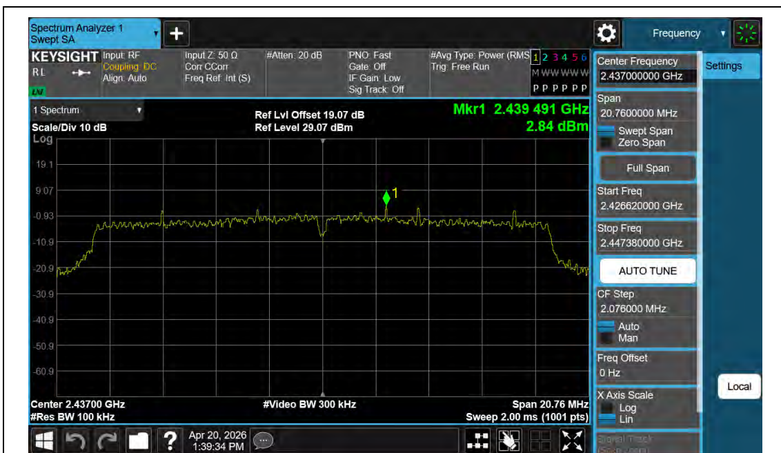
11N20MIMO-Ant1-2437-PASS
