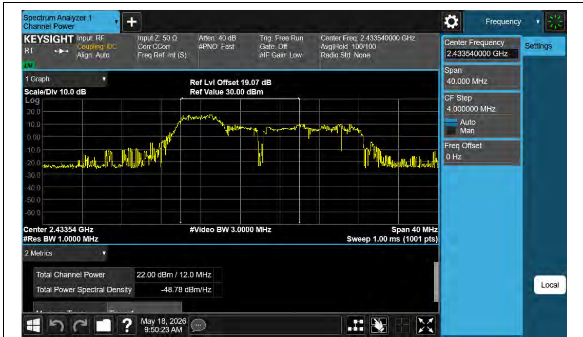
11AX20MIMO-Ant1-2437-52Tone-RU37-PASS
