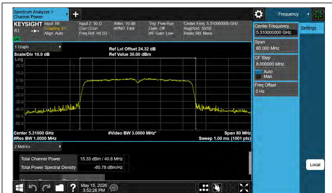
11AX40MIMO-Ant1-5310-PASS
