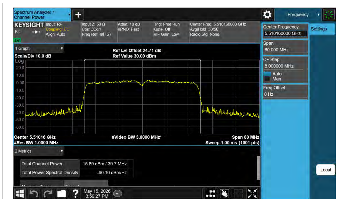
11AX40MIMO-Ant1-5510-PASS
