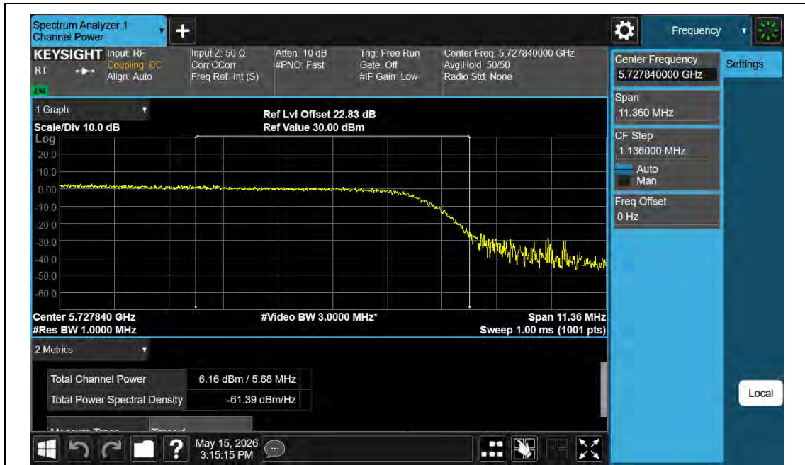
11AX20MIMO-Ant1-5720_UNII-3-PASS
