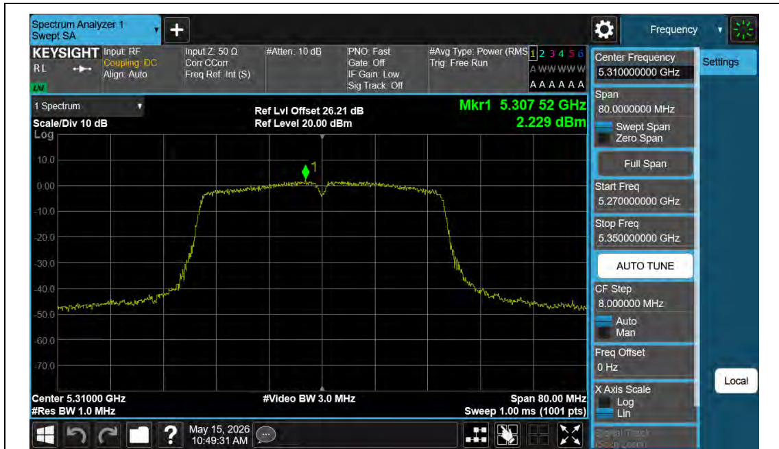
11N40MIMO-Ant1-5310-PASS
