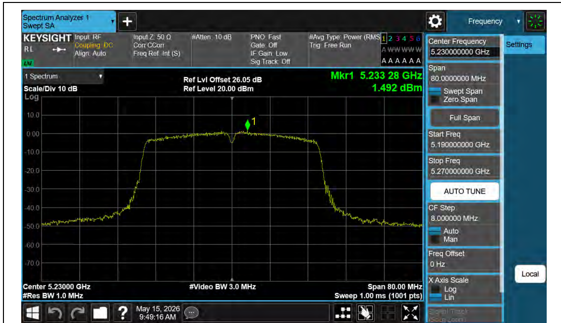
11AC40MIMO-Ant1-5230-PASS
