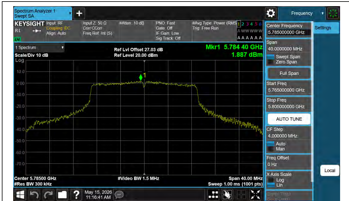
11AC20MIMO-Ant1-5785-PASS
