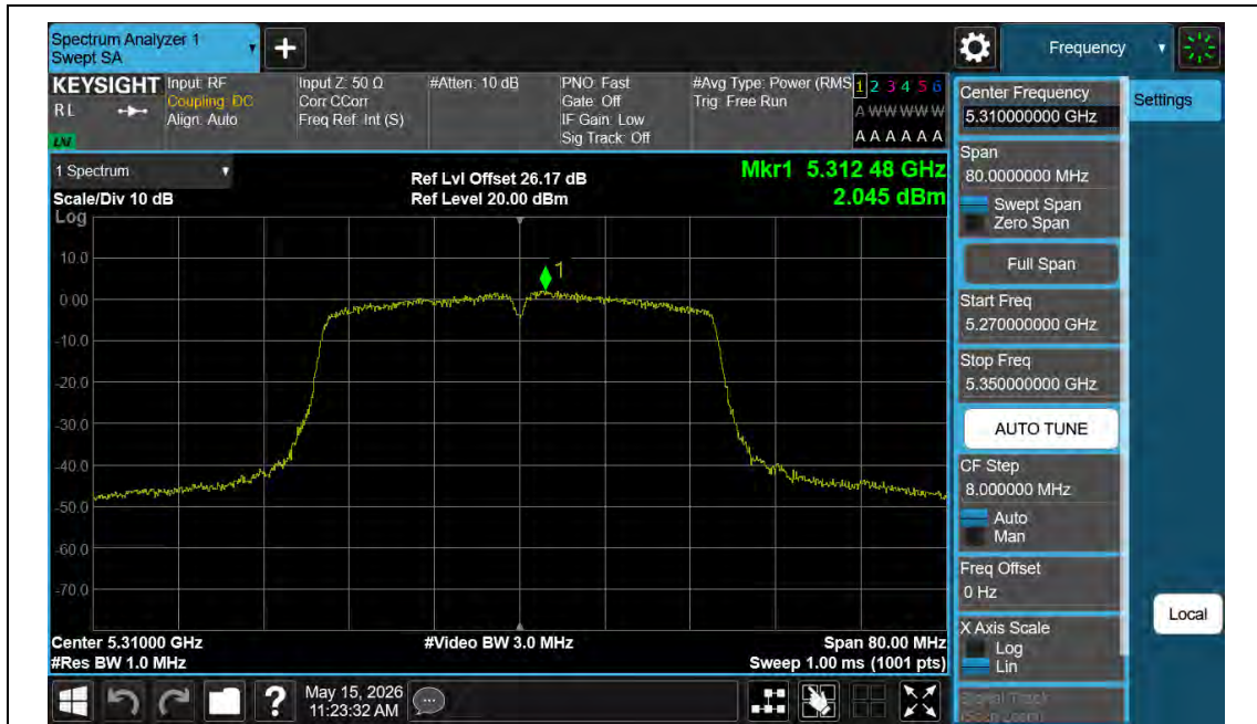
11AC40MIMO-Ant1-5310-PASS
