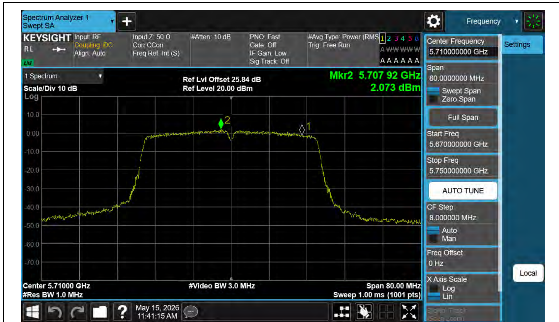
11AC40MIMO-Ant1-5710_UNII-2C-PASS
