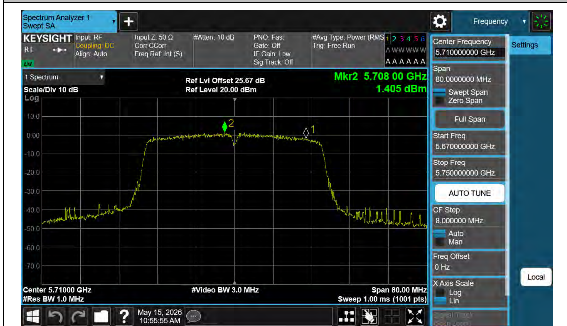
11N40MIMO-Ant0-5710_UNII-3-PASS
