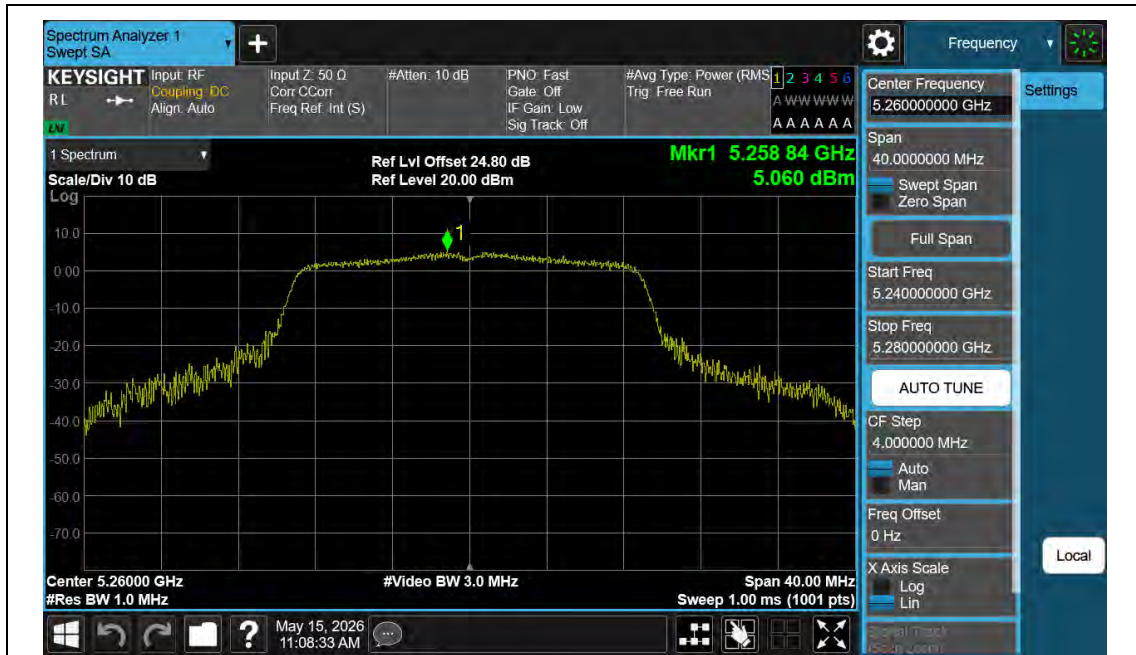
11AC20MIMO-Ant1-5260-PASS
