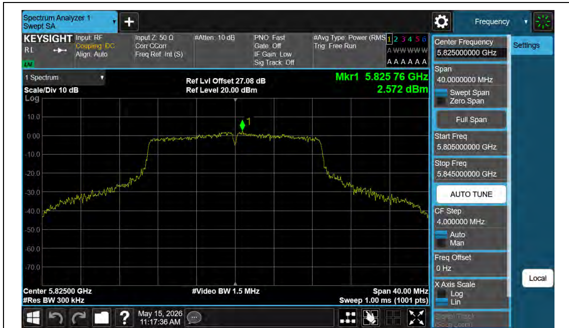
11AC20MIMO-Ant1-5825-PASS
