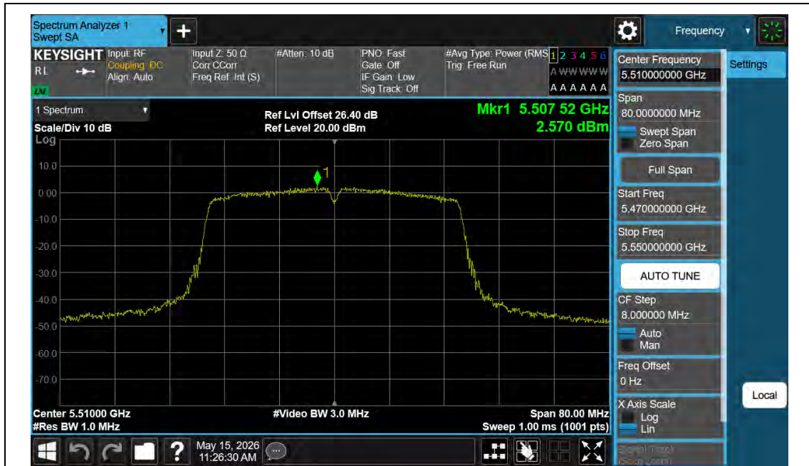
11AC40MIMO-Ant1-5510-PASS
