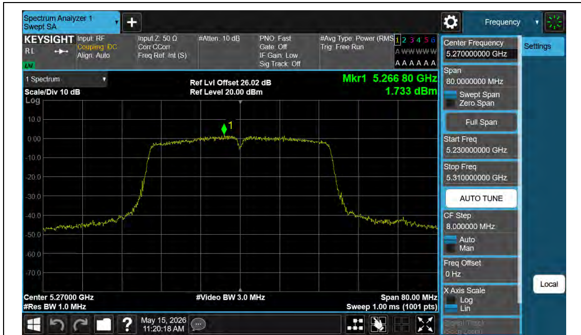
11AC40MIMO-Ant1-5270-PASS
