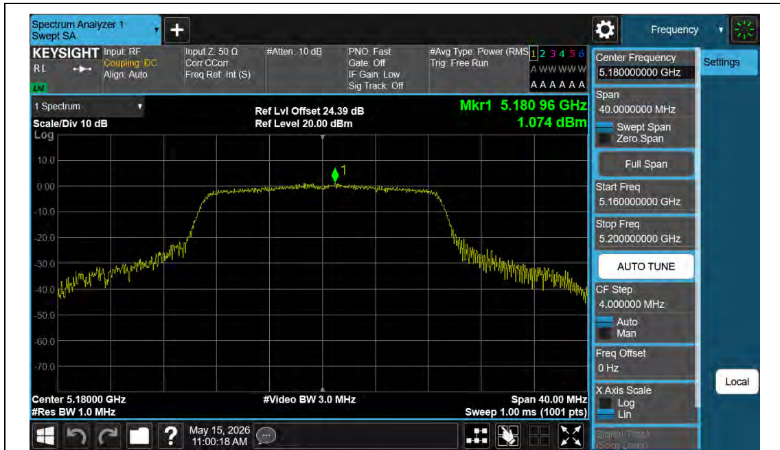
11AC20MIMO-Ant1-5180-PASS
