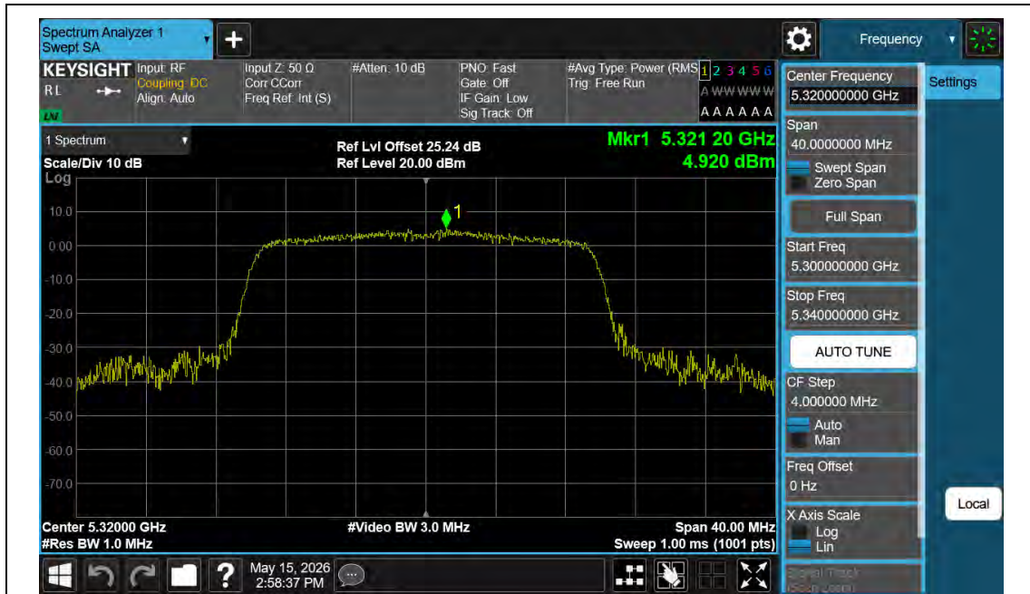
11AX20MIMO-Ant1-5320-PASS
