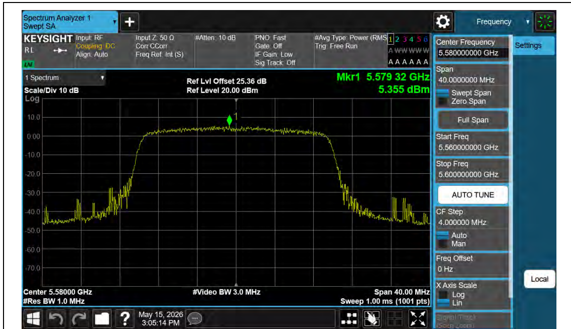
11AX20MIMO-Ant1-5580-PASS
