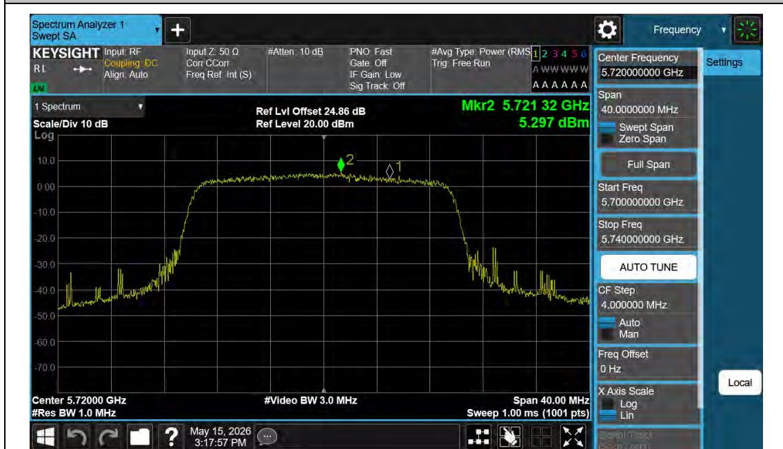
11AX20MIMO-Ant0-5720_UNII-3-PASS
