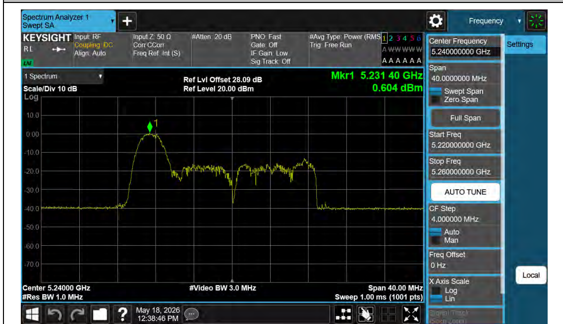
11AX20MIMO-Ant0-5240-52Tone-RU37-PASS
