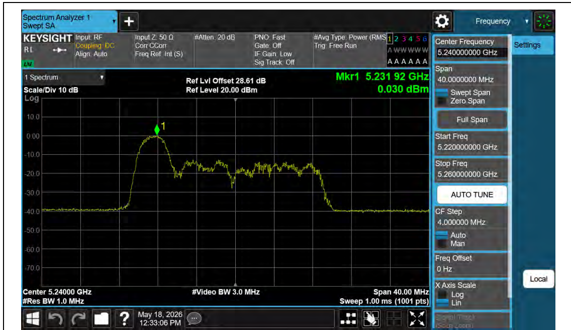
11AX20MIMO-Ant1-5240-26Tone-RU0-PASS
