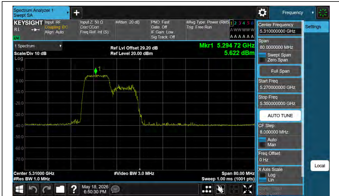
11AX40MIMO-Ant1-5310-106Tone-RU53-PASS
