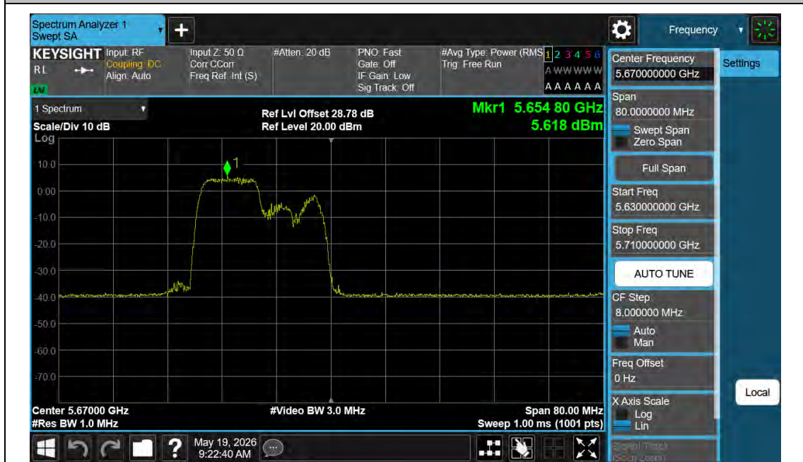
11AX40MIMO-Ant0-5710_UNII-2C-106Tone-RU53-PASS
