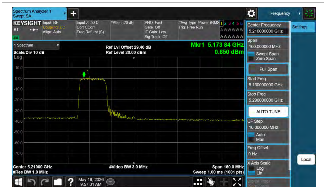
11AX80MIMO-Ant1-5210-242Tone-RU61-PASS
