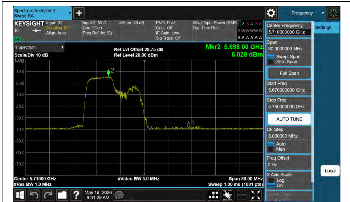
11AX40MIMO-Ant1-5710_UNII-2C-106Tone-RU53-PASS
