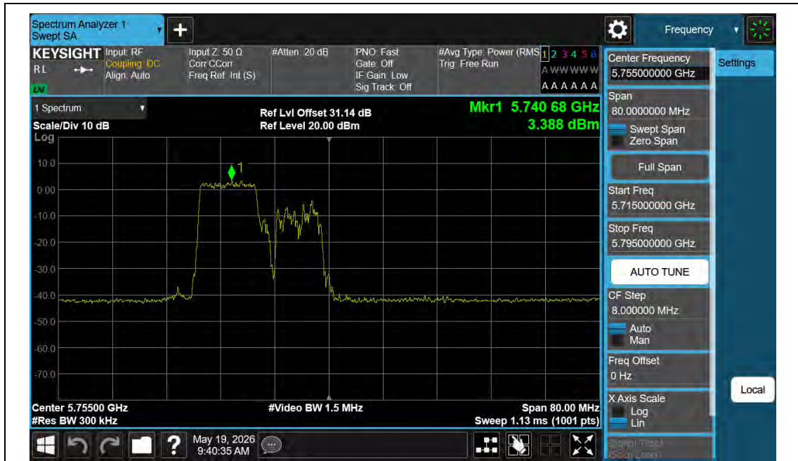
11AX40MIMO-Ant1-5755-106Tone-RU53-PASS
