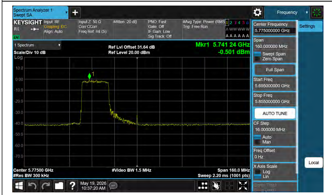
11AX80MIMO-Ant1-5775-242Tone-RU61-PASS
