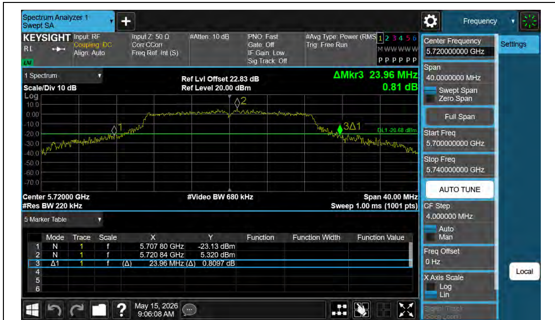
11AC20MIMO-Ant1-5720
