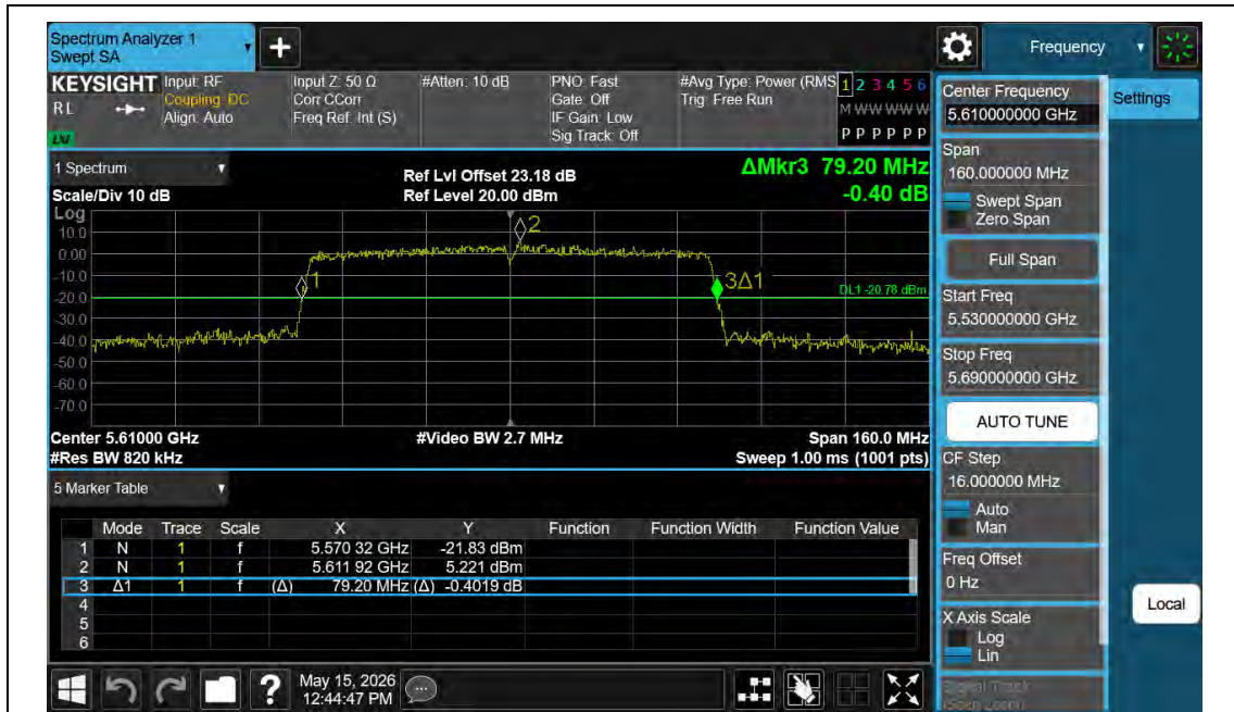
11AC80MIMO-Ant1-5610
