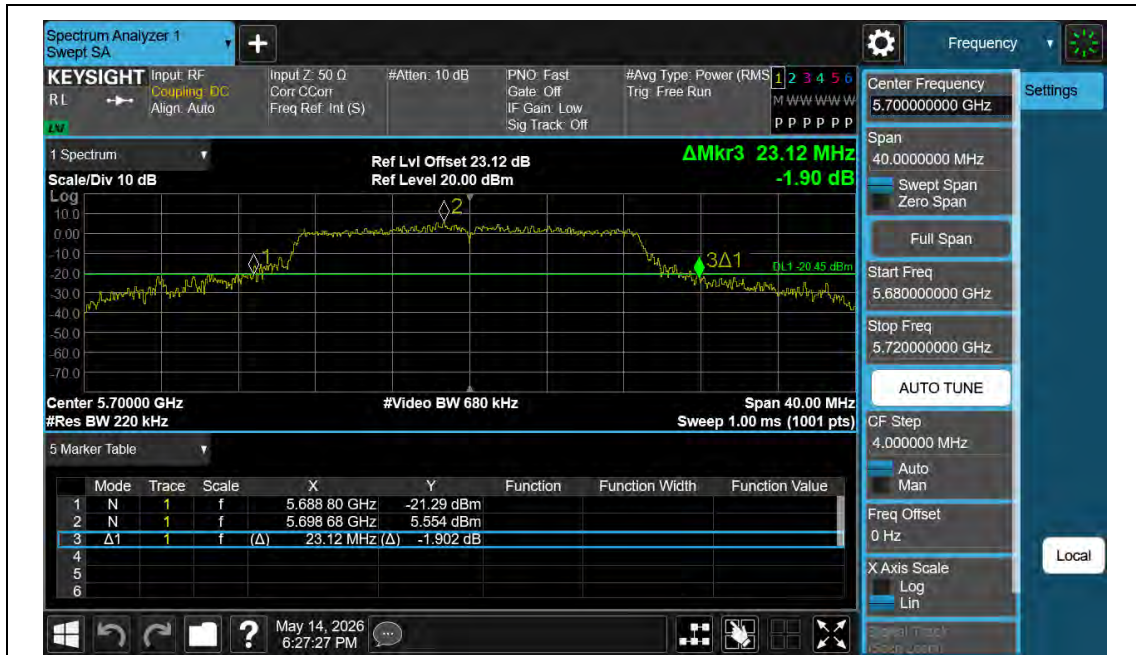
11AC20MIMO-Ant1-5700
