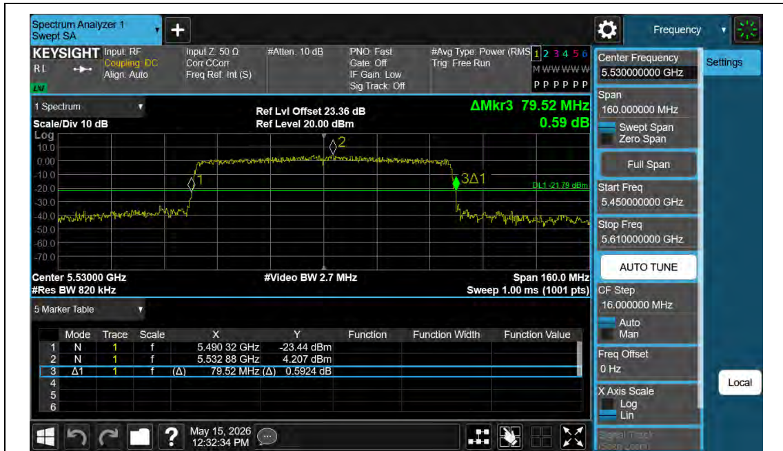
11AC80MIMO-Ant1-5530
