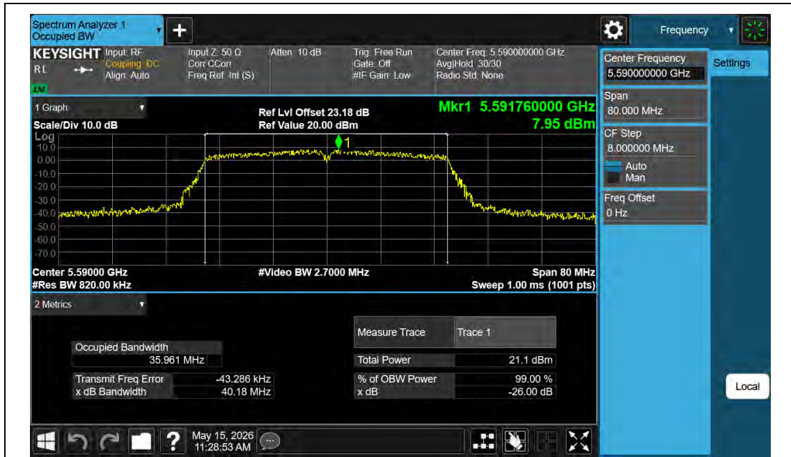
11AC40MIMO-Ant1-5590
