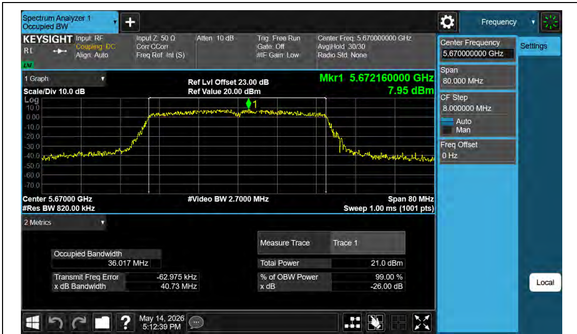
11N40MIMO-Ant1-5670
