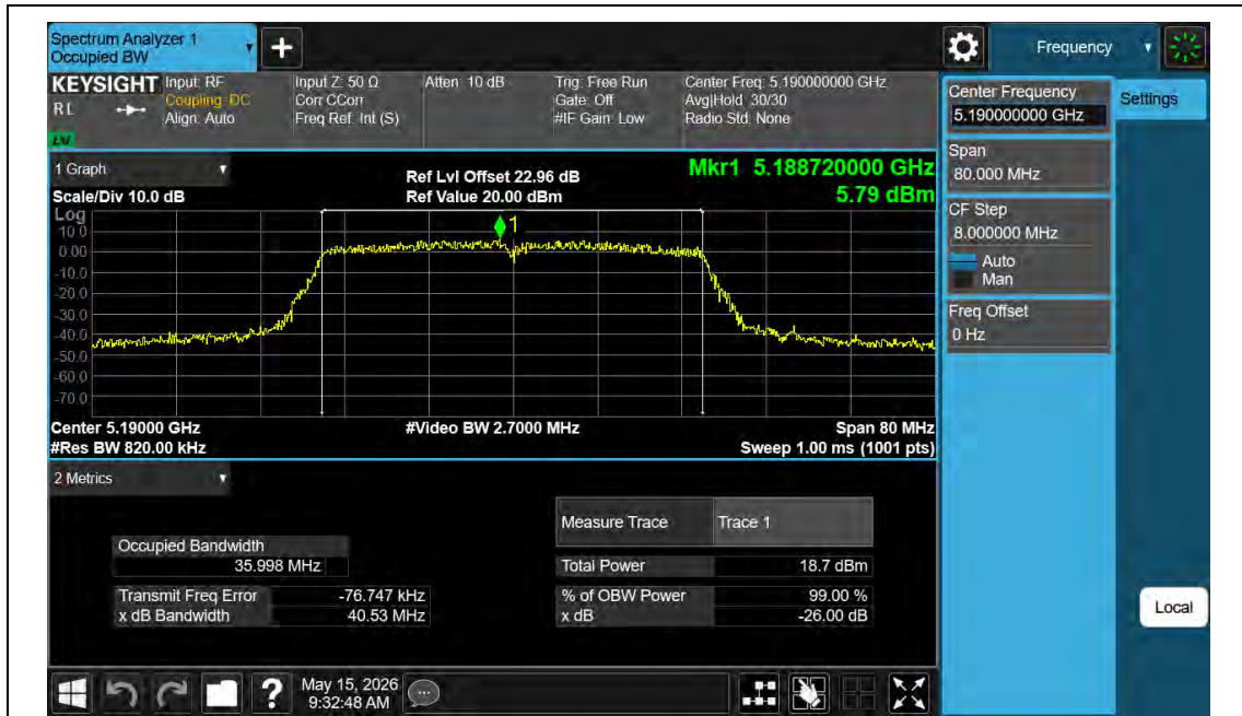
11AC40MIMO-Ant1-5190
