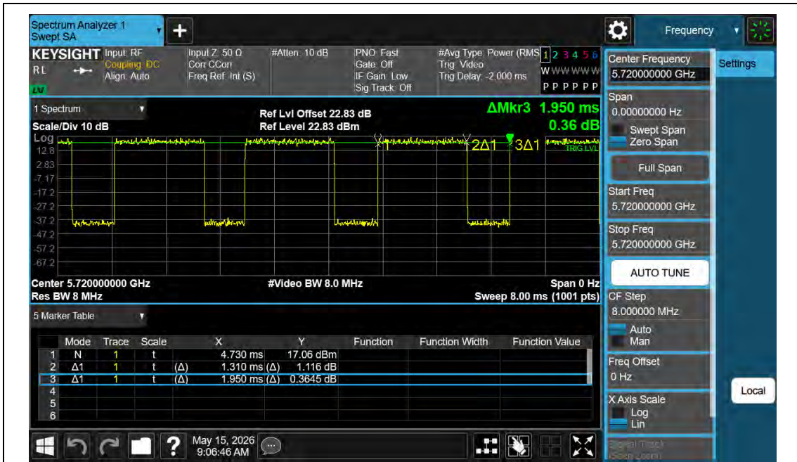
NTNV-11AC20MIMO-Ant1-5720
