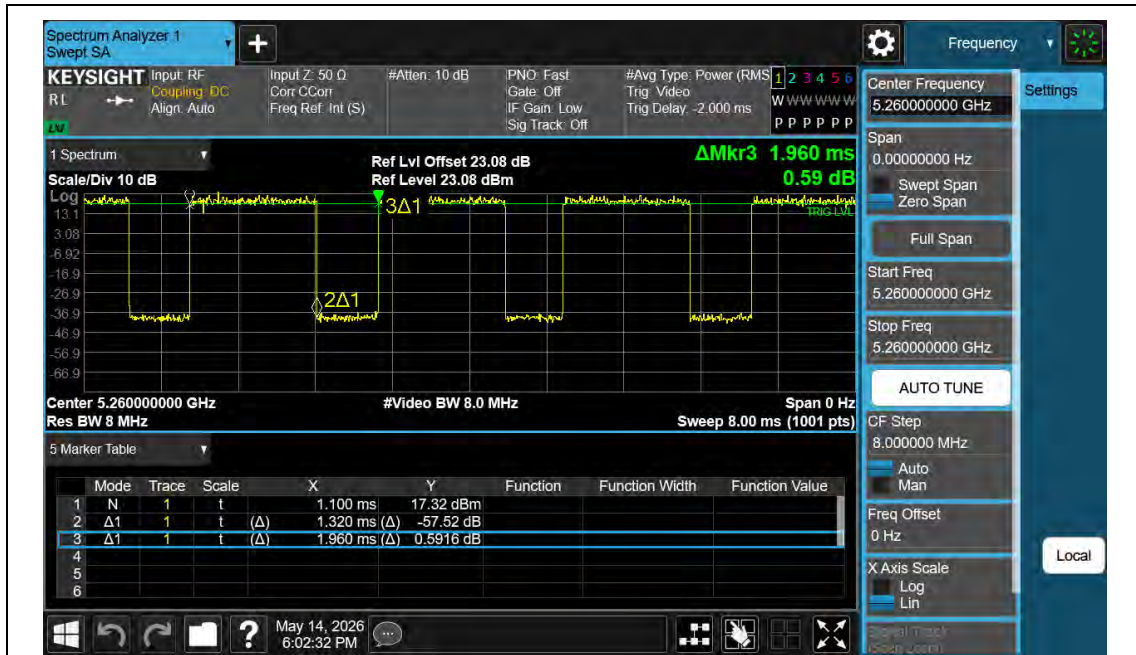
NTNV-11AC20MIMO-Ant1-5260
