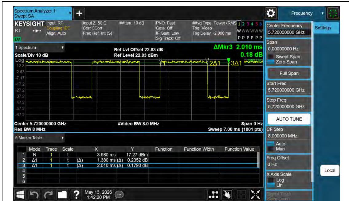
NTNV-11A-Ant1-5720
