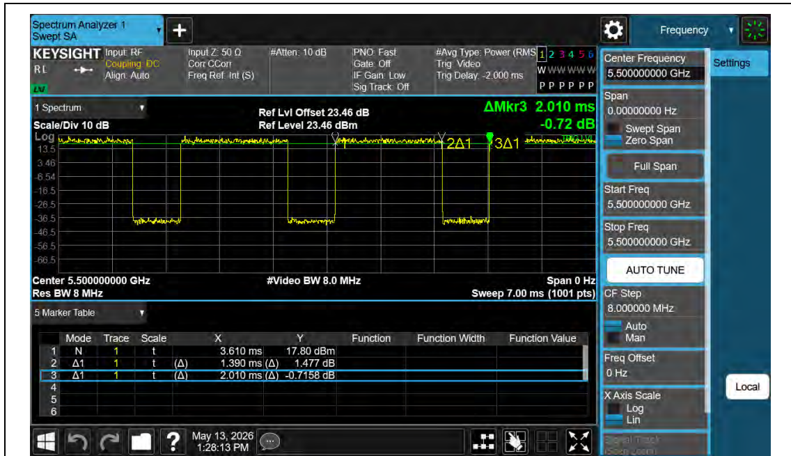
NTNV-11A-Ant1-5500
