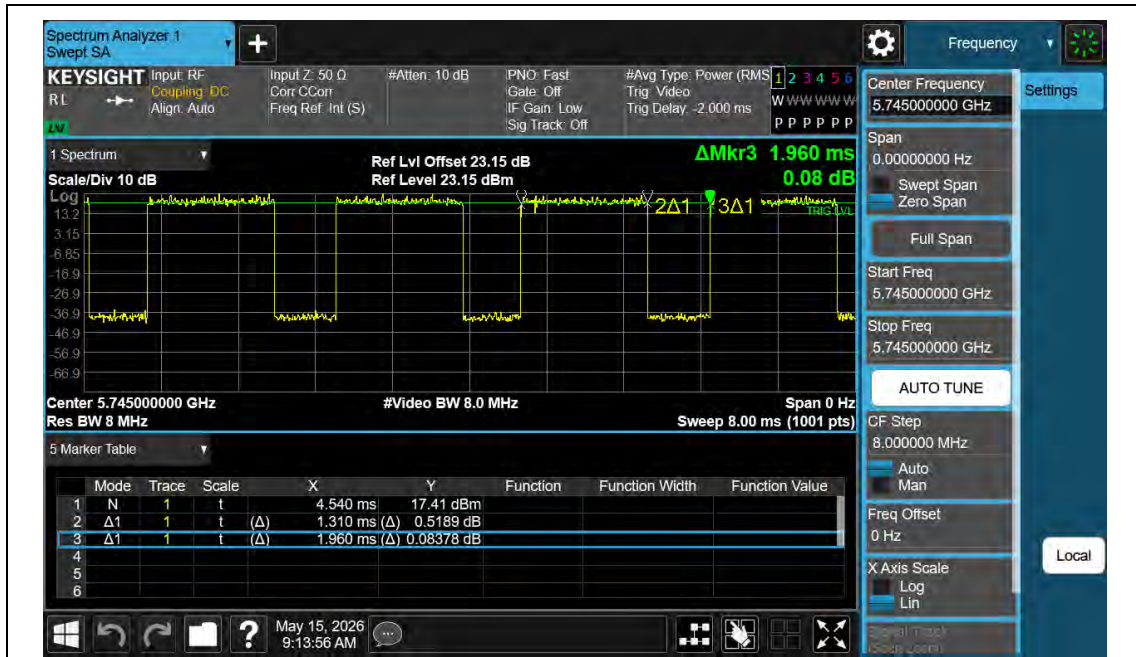
NTNV-11AC20MIMO-Ant1-5745
