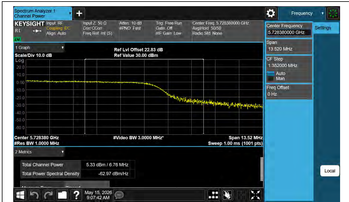
11AC20MIMO-Ant1-5720_UNII-3-PASS
