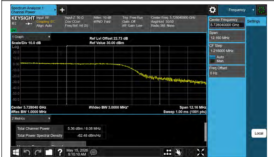
11AC20MIMO-Ant0-5745-PASS
