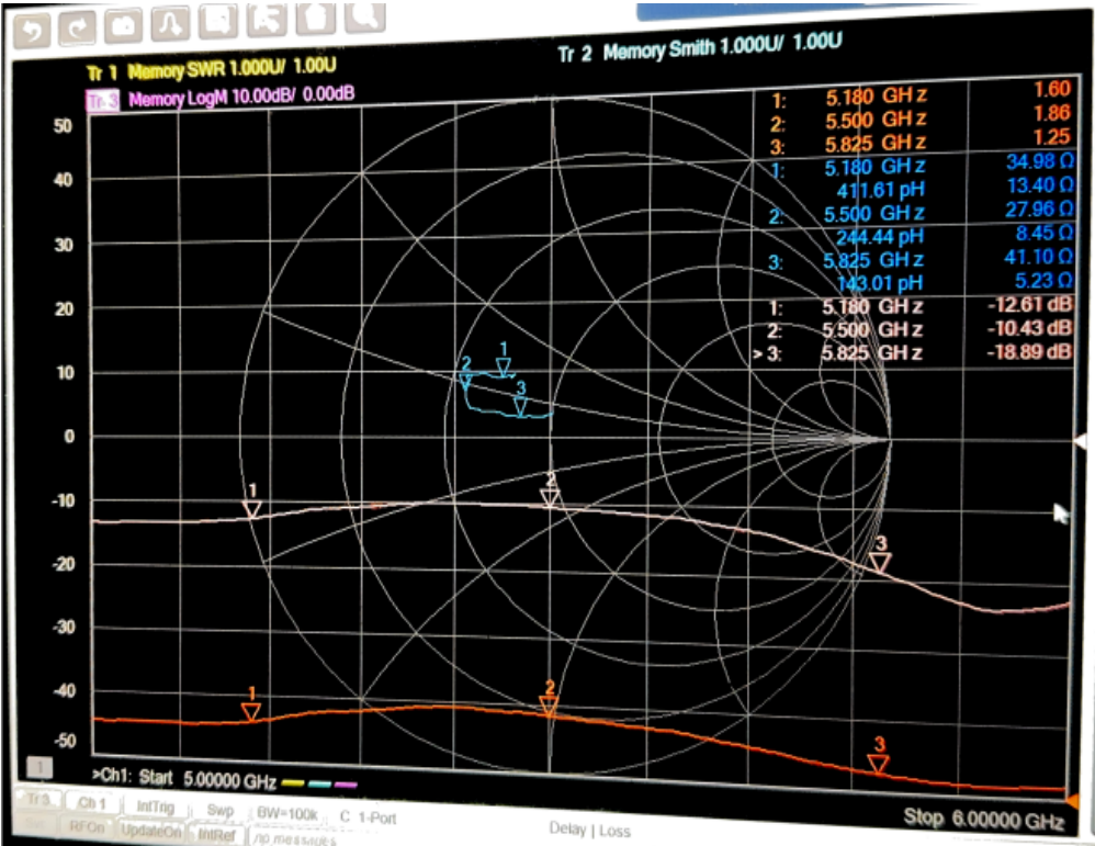
Wireless模组天线S11和VSWR
