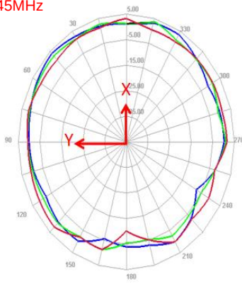
Horizontal 5745MHz
