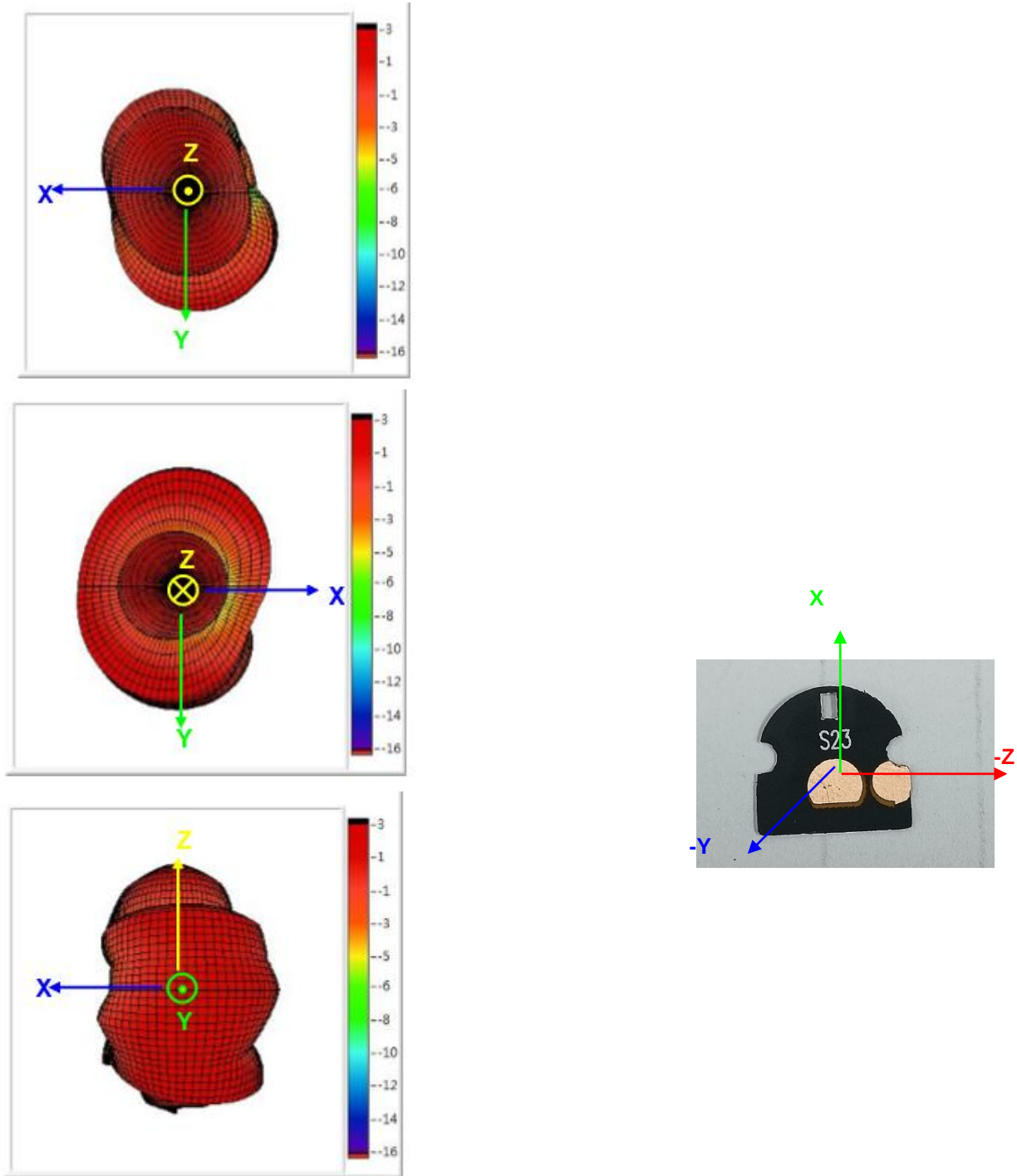
9-1.3D Gain Pattern (Radiation Pattern at 2450 MHz)
