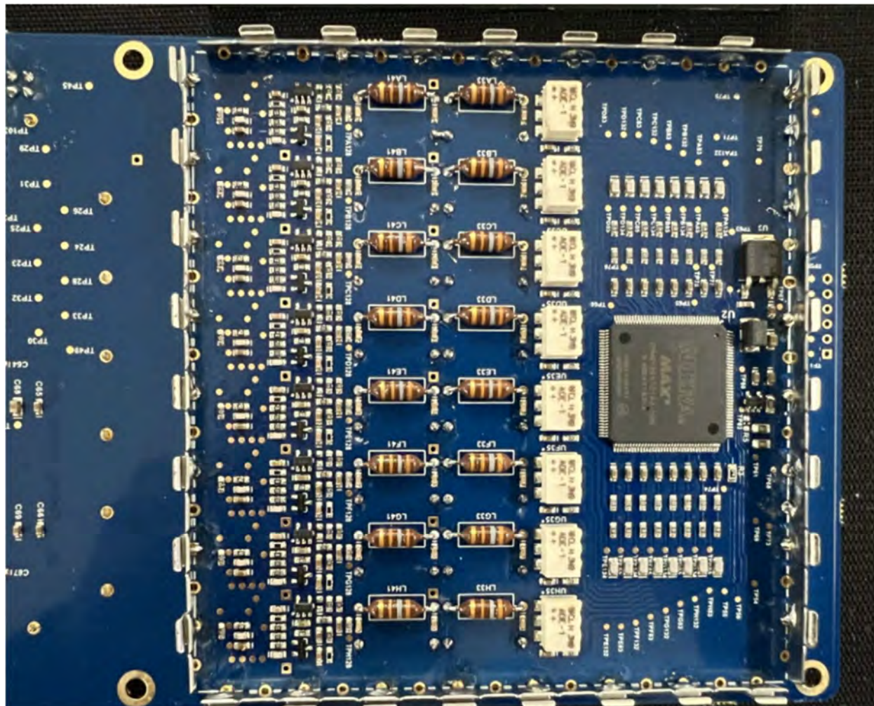
DSBR board (bottom zoom view)
