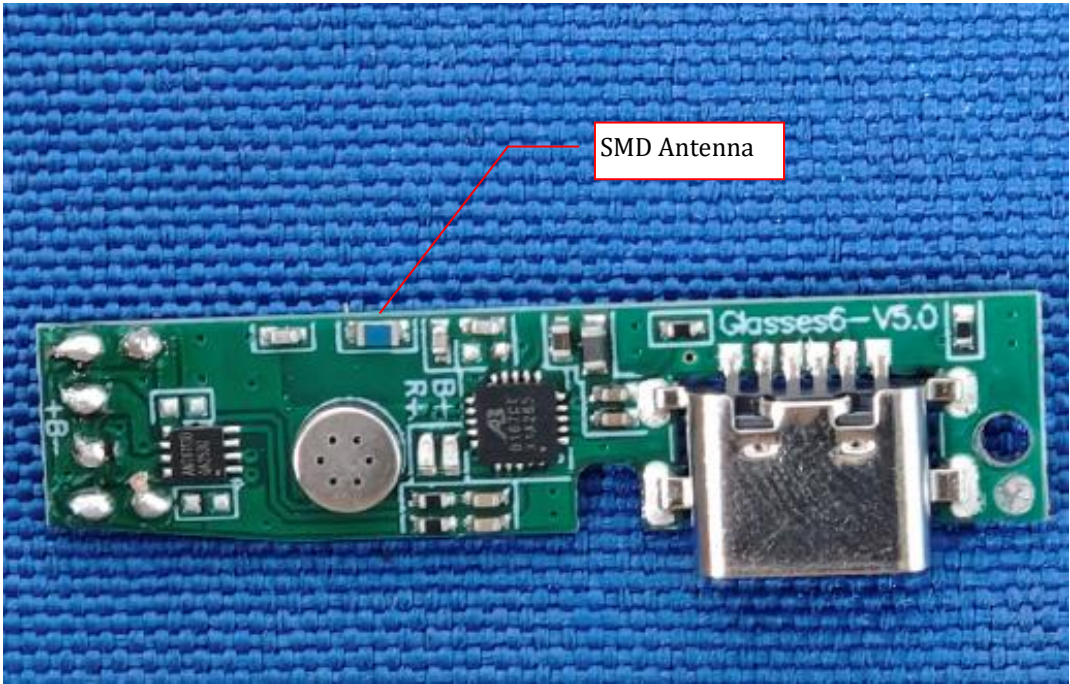
EUT Internal View 4
