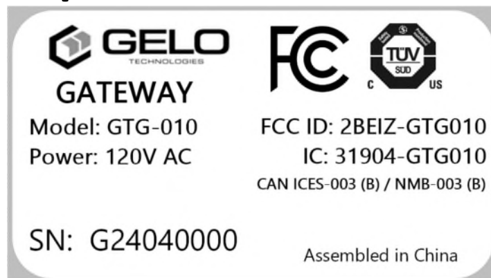
Figure 1 - Label – Gateway
