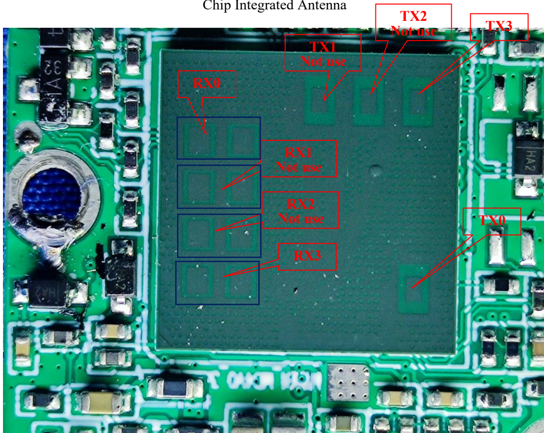
Chip Integrated Antenna
