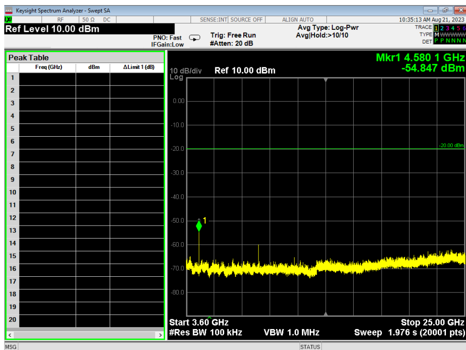
Figure 13 - Radiated Emissions Plot, Mid Channel, 3.6G – 25G
