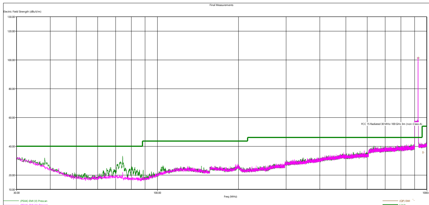
Figure 7 - Radiated Emissions Plot, High Channel
