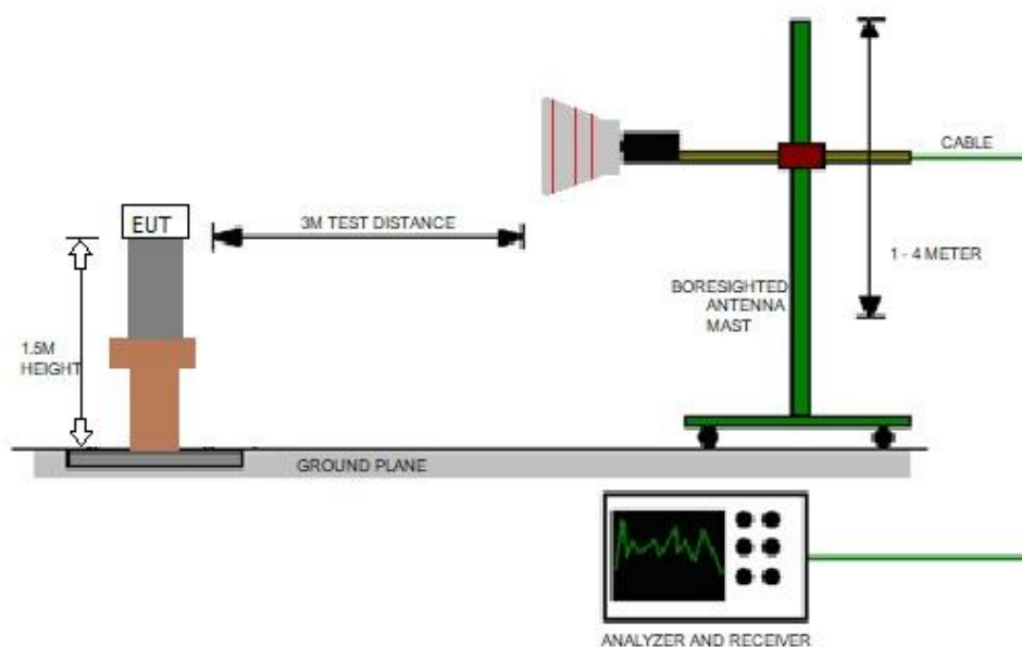
Figure 3 - Radiated Emissions Test Setup, >1GHz
