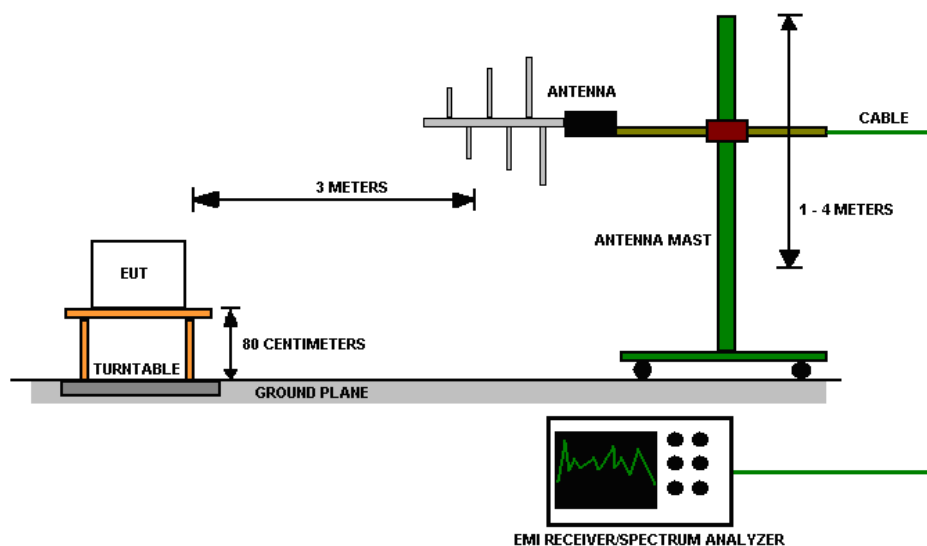
Figure 2 - Radiated Emissions Test Setup, 30MHz – 1GHz
