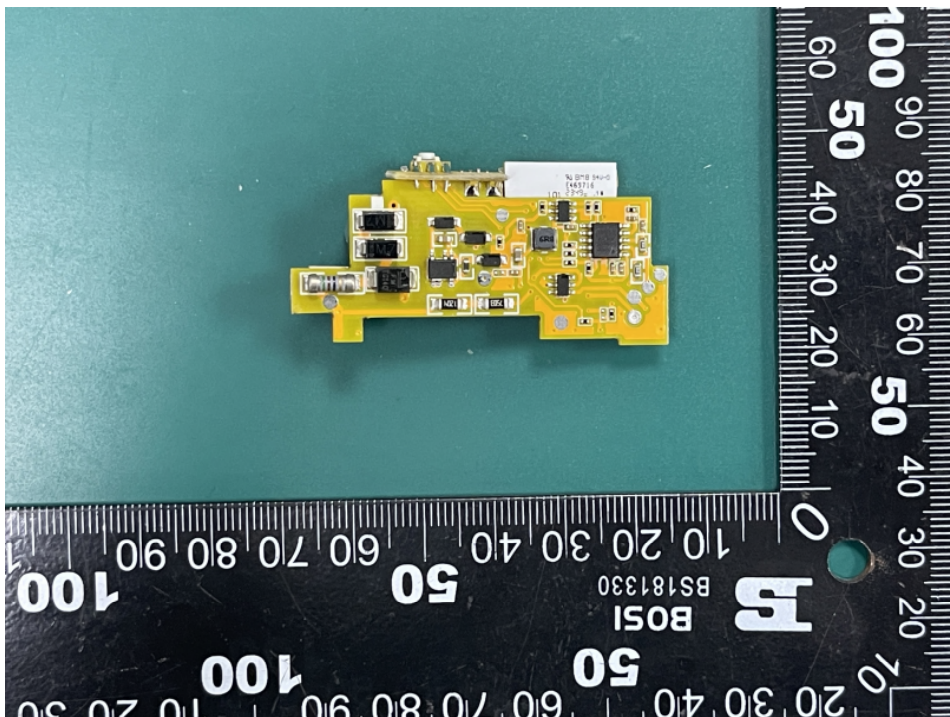
TO-Q-SY2-JWT Internal view: PCB
