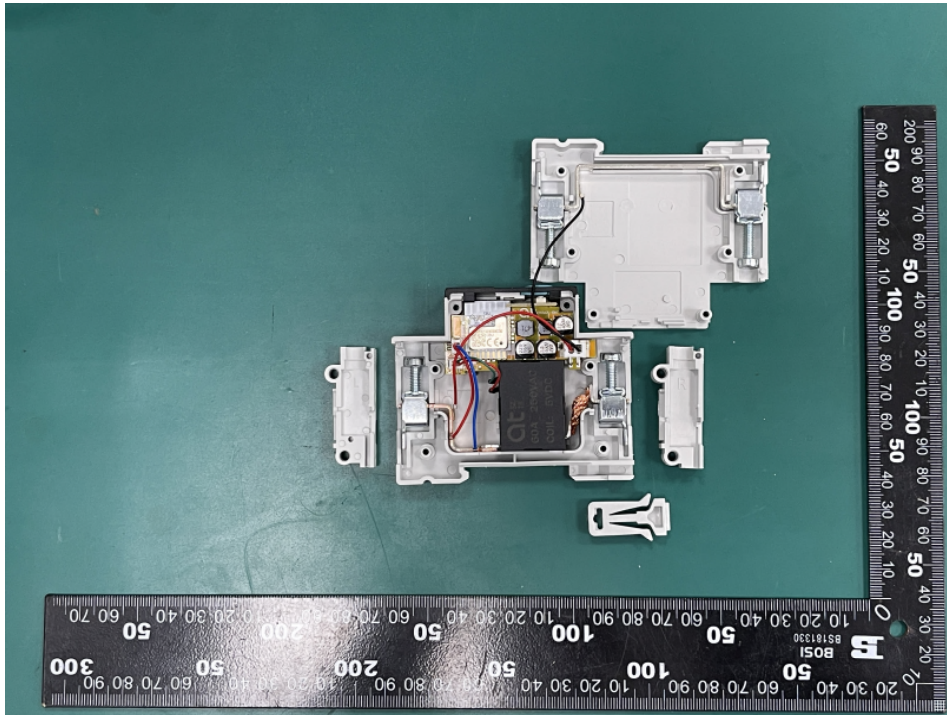
TO-Q-SY1-JWT Internal view
