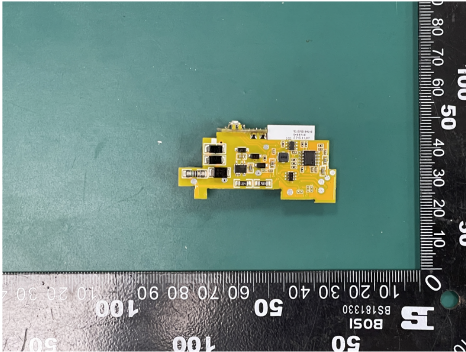
TO-Q-SY1-JWT Internal view: PCB
