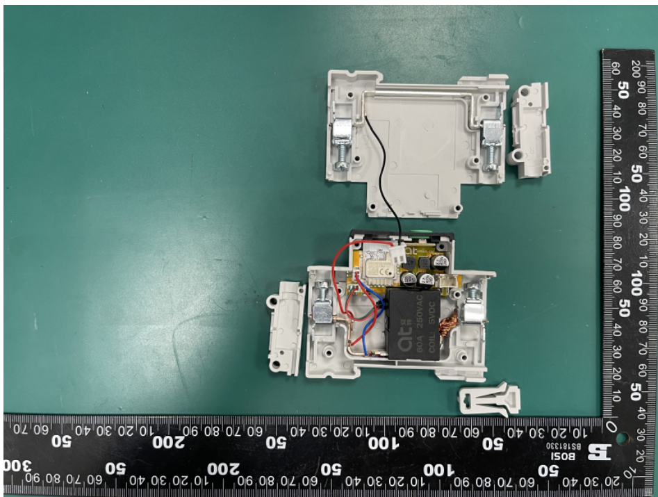
TO-Q-SY2-JWT Internal view
