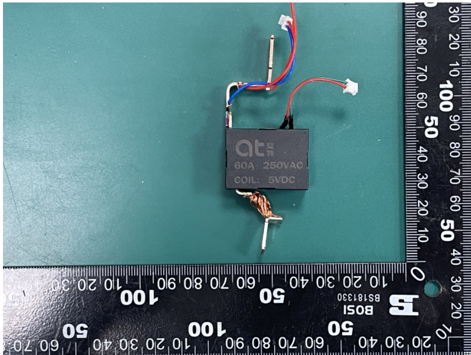
TO-Q-SY1-JWT& TO-Q-SY2-JWT Internal view: Latching Relay
