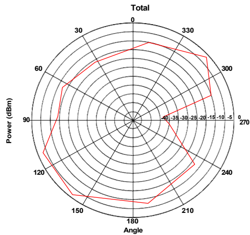
XY Plane at f = 2.400GHz
