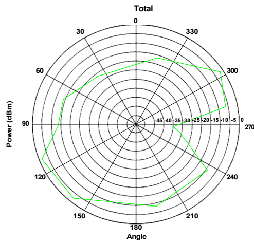
XY Plane at Freq = 2.450GHz
