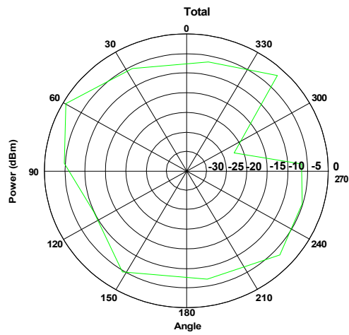
YZ Plane at Freq = 2.450GHz
