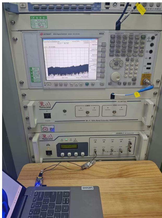
Test Setup Photo(s) of RF Conducted
