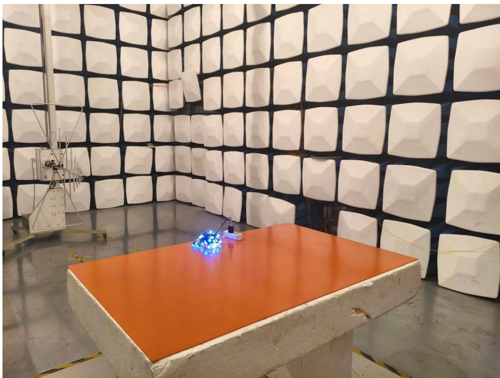
Test Setup Photo(s) of Radiated Emissions Measurement
