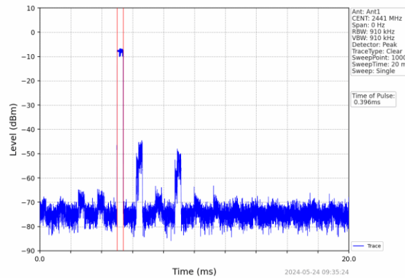
2DH1
