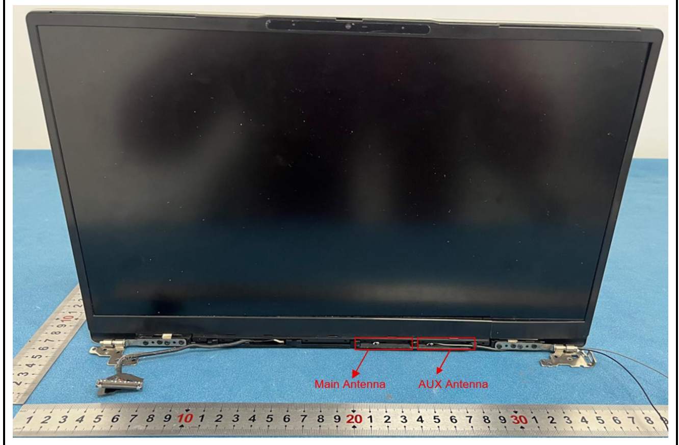
Photo 5: Antenna Locations
