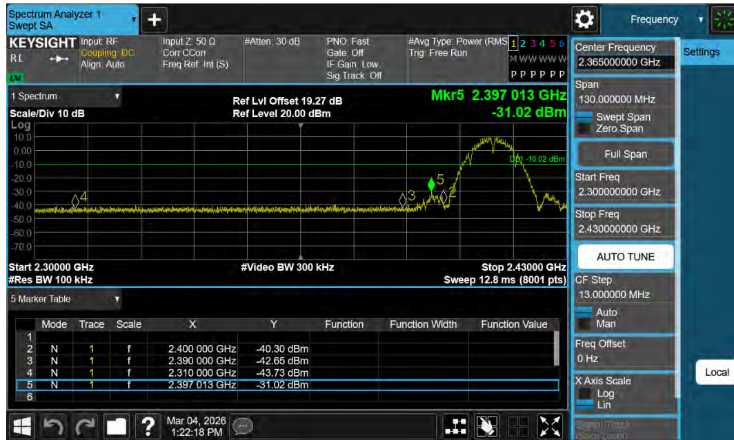
11B-Ant2-2412-PASS
