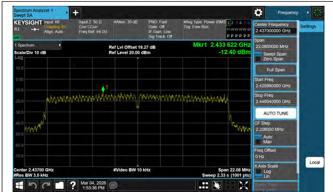
11N20MIMO-Ant2-2437-PASS
