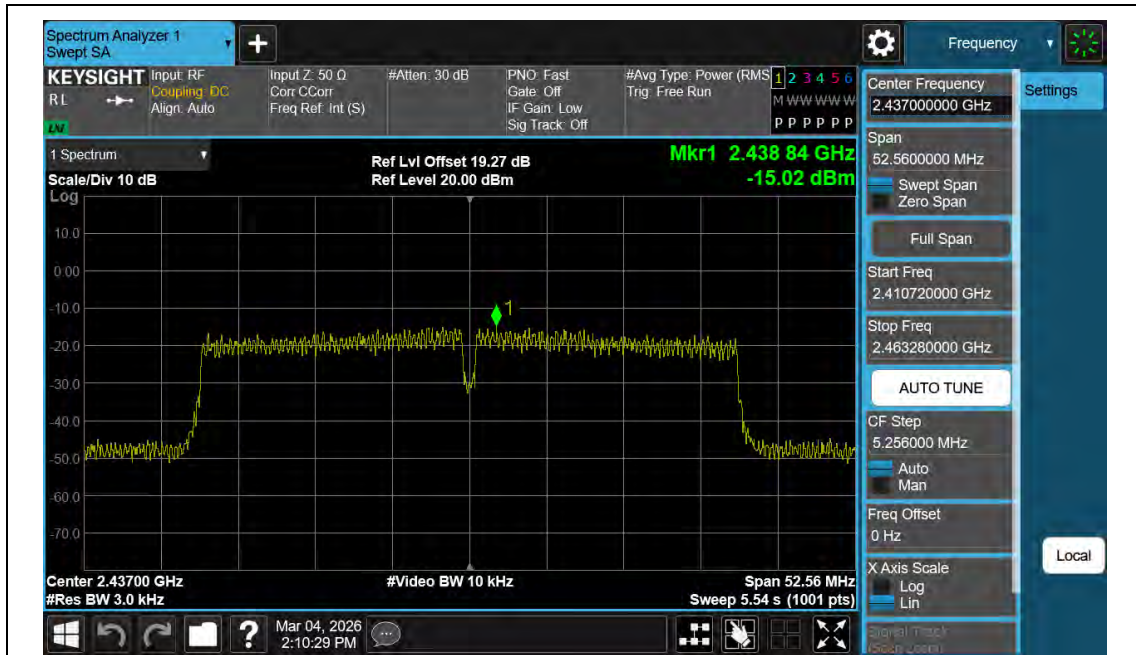
11N40MIMO-Ant2-2437-PASS
