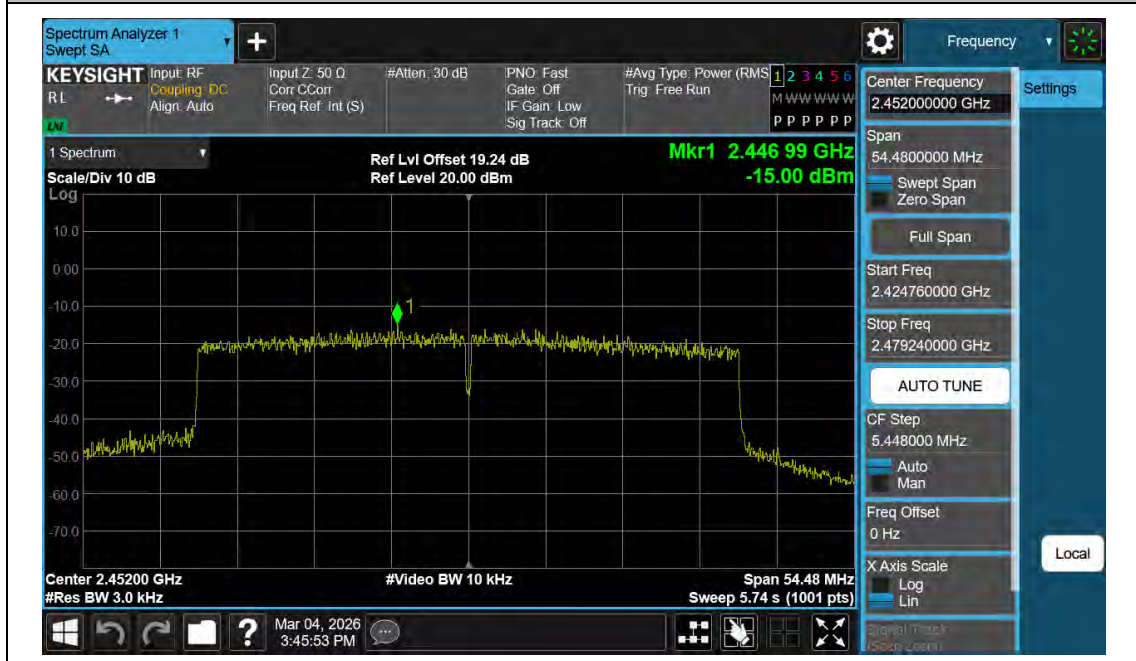
11BE40MIMO-Ant2-2452-PASS
