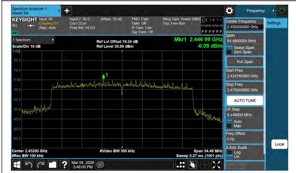
11BE40MIMO-Ant2-2452-PASS
