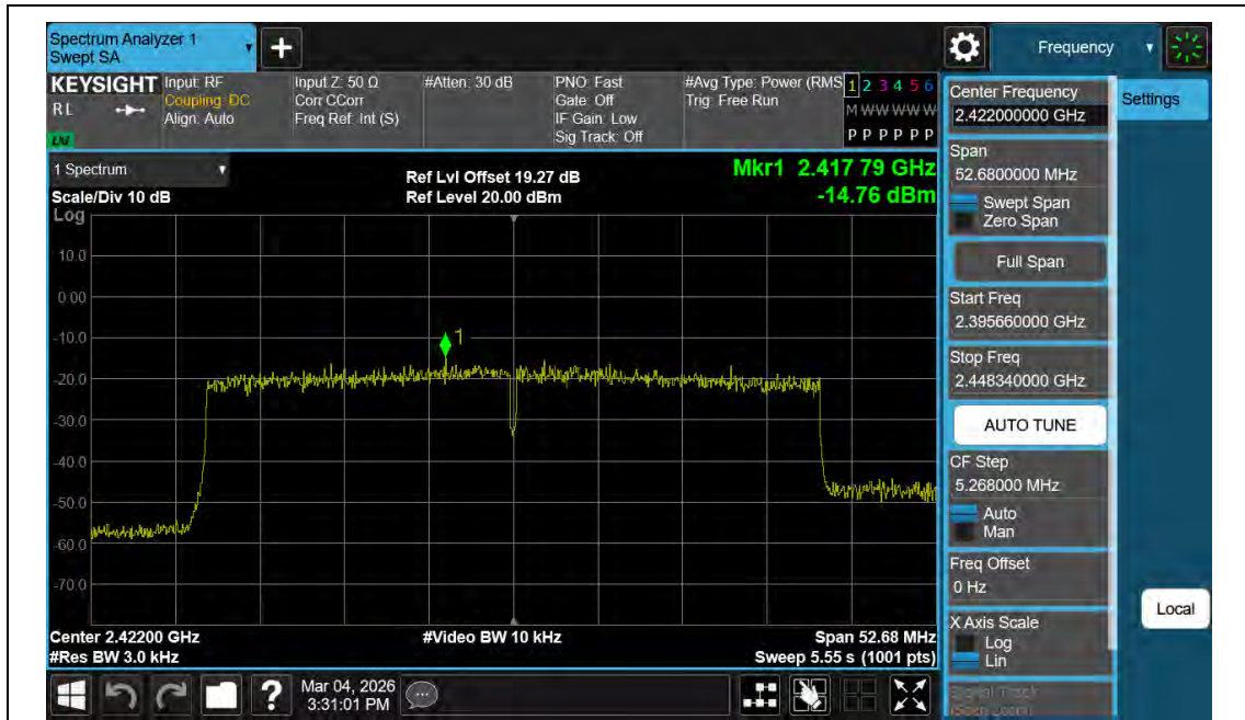
11BE40MIMO-Ant2-2422-PASS
