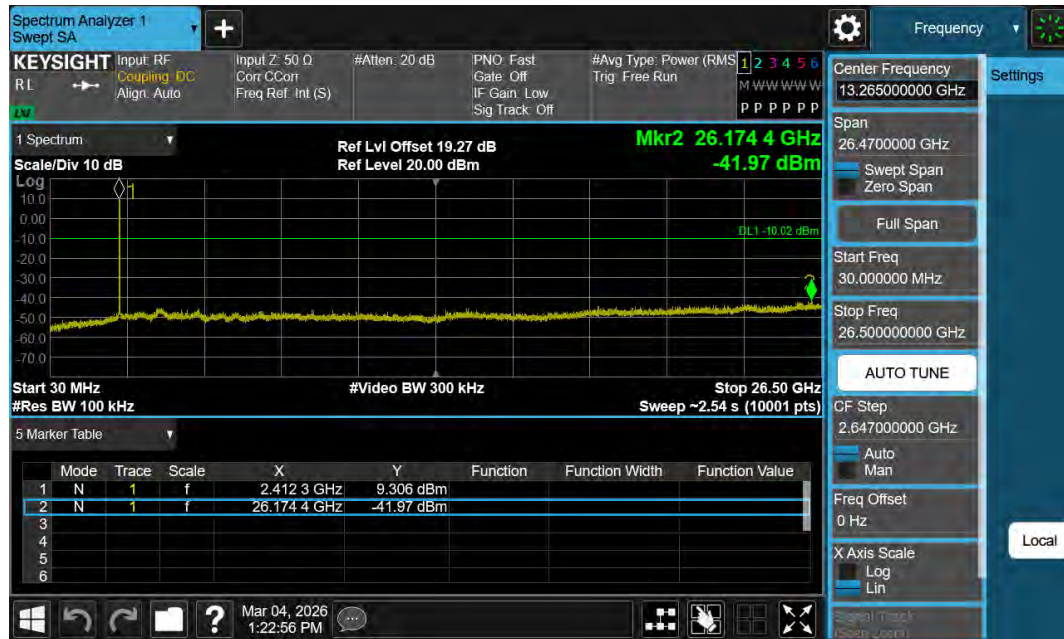
11B-Ant2-2412-30~26500-PASS
