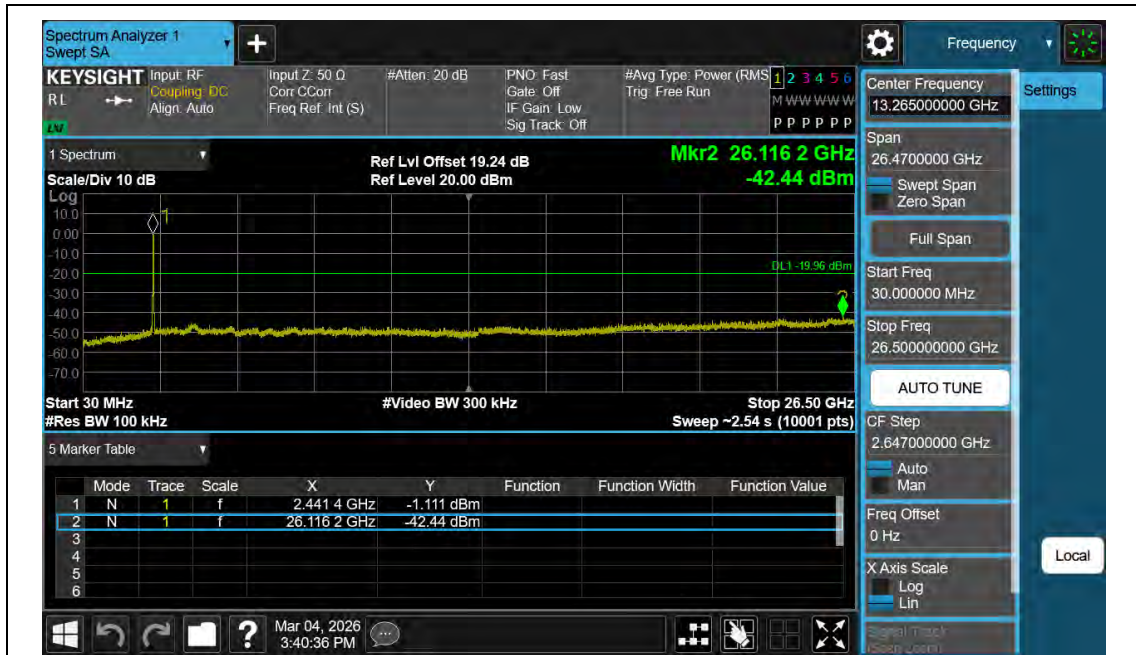
11BE40MIMO-Ant1-2452-30~26500-PASS
