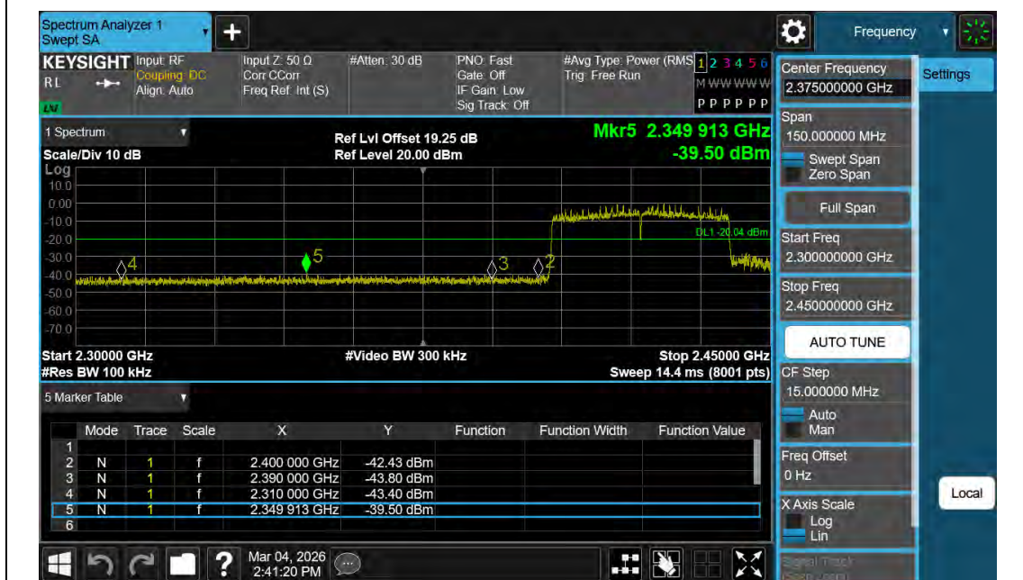
11AX40MIMO-Ant1-2452-PASS
