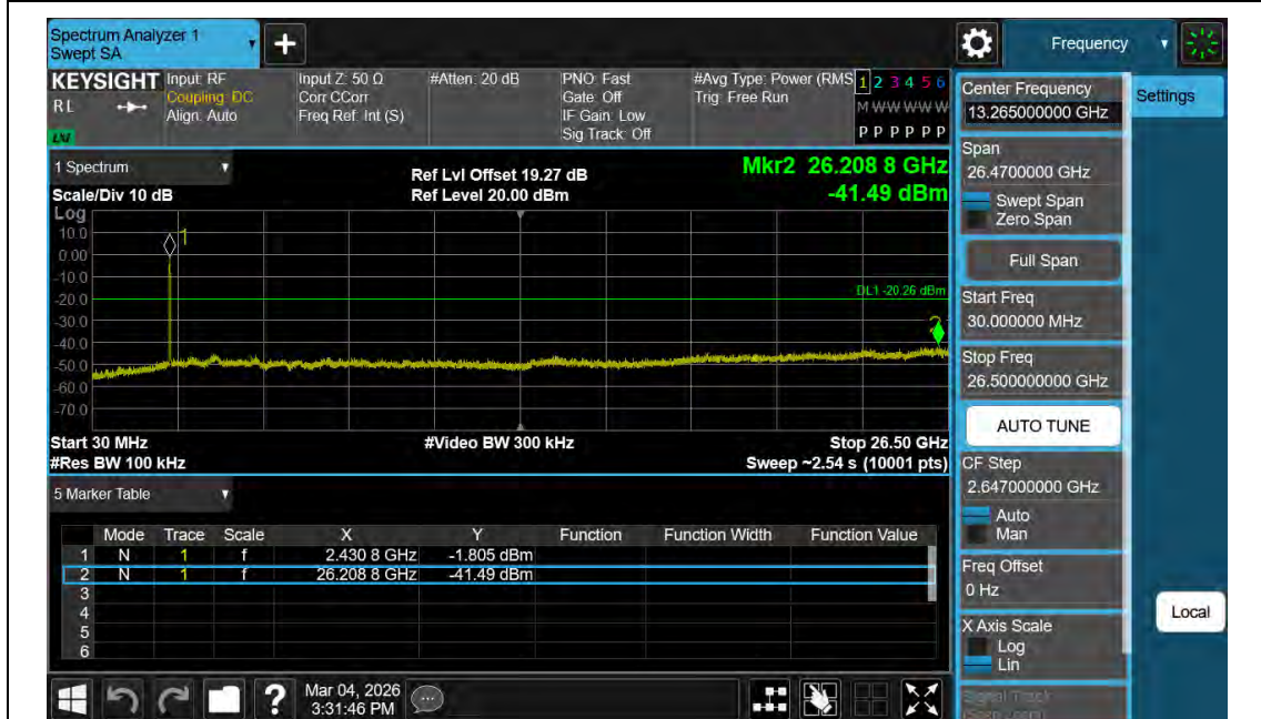
11BE40MIMO-Ant2-2422-30~26500-PASS
