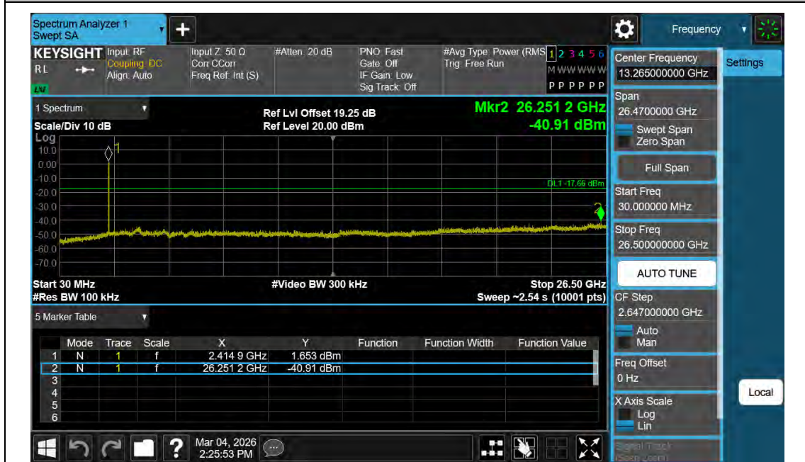
11AX20MIMO-Ant1-2437-30~26500-PASS
