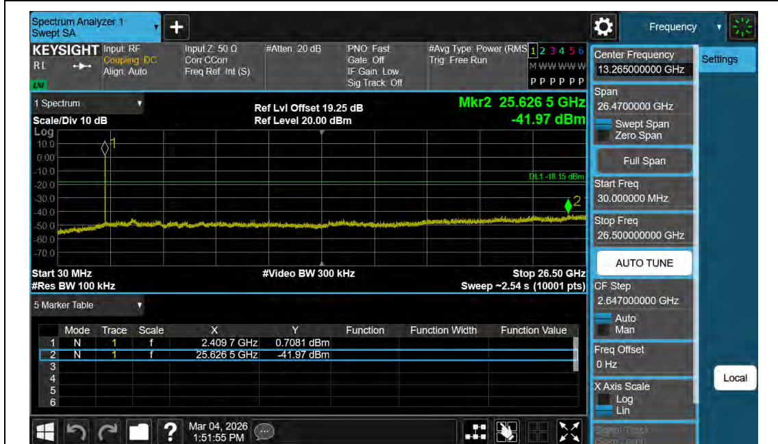
11N20MIMO-Ant1-2437-30~26500-PASS
