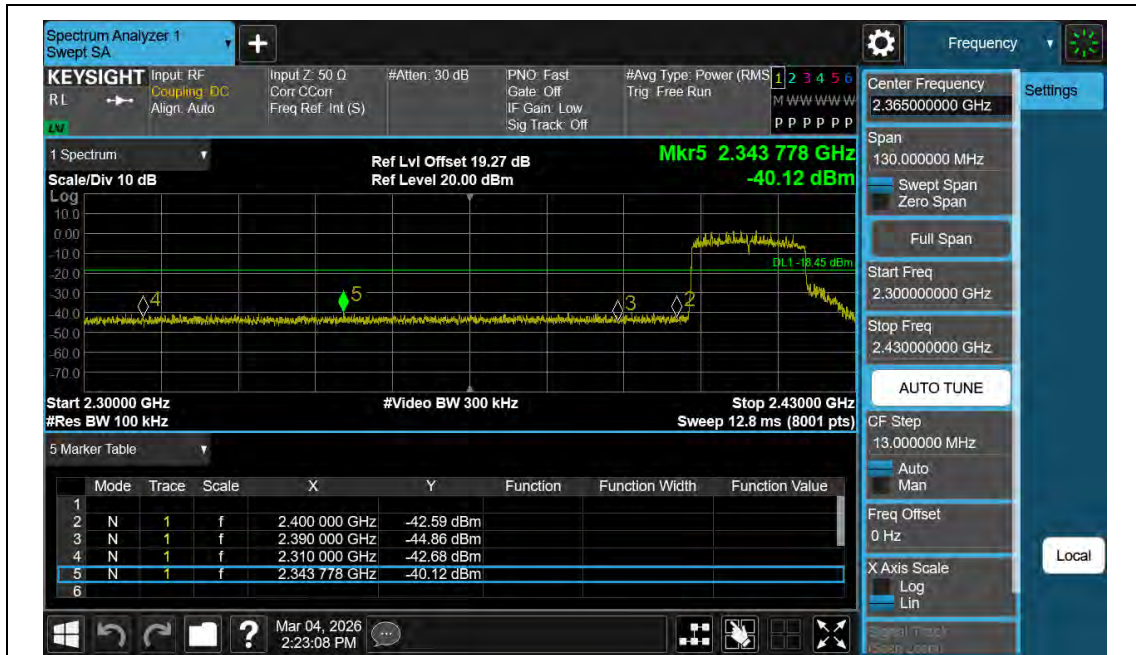
11AX20MIMO-Ant2-2412-PASS
