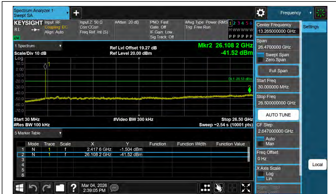
11AX40MIMO-Ant2-2422-30~26500-PASS
