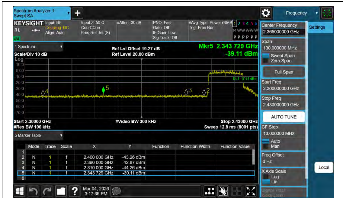
11BE20MIMO-Ant2-2412-PASS
