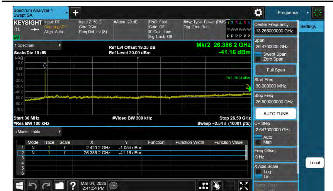
11AX40MIMO-Ant1-2437-30~26500-PASS
