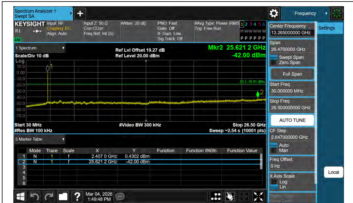
11N20MIMO-Ant2-2412-30~26500-PASS
