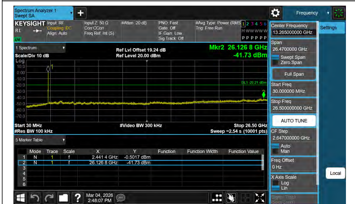
11AX40MIMO-Ant1-2452-30~26500-PASS
