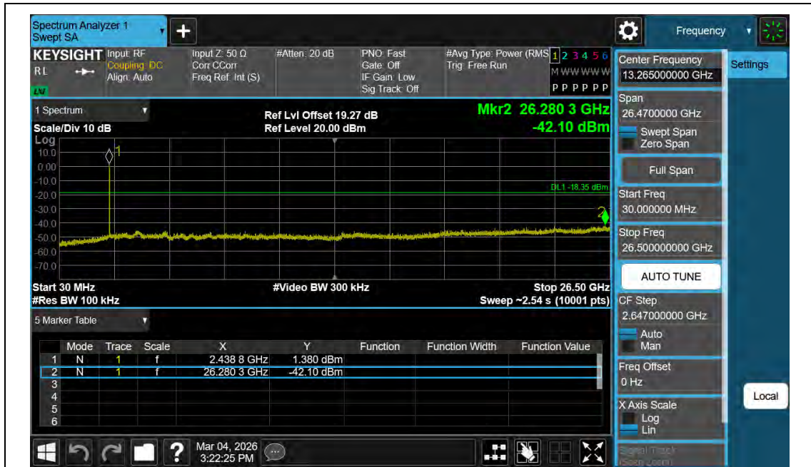
11BE20MIMO-Ant2-2437-30~26500-PASS
