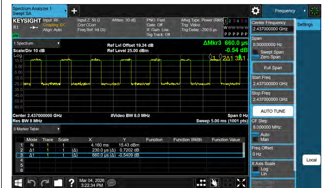
NTNV-11BE40MIMO-Ant1-2437
