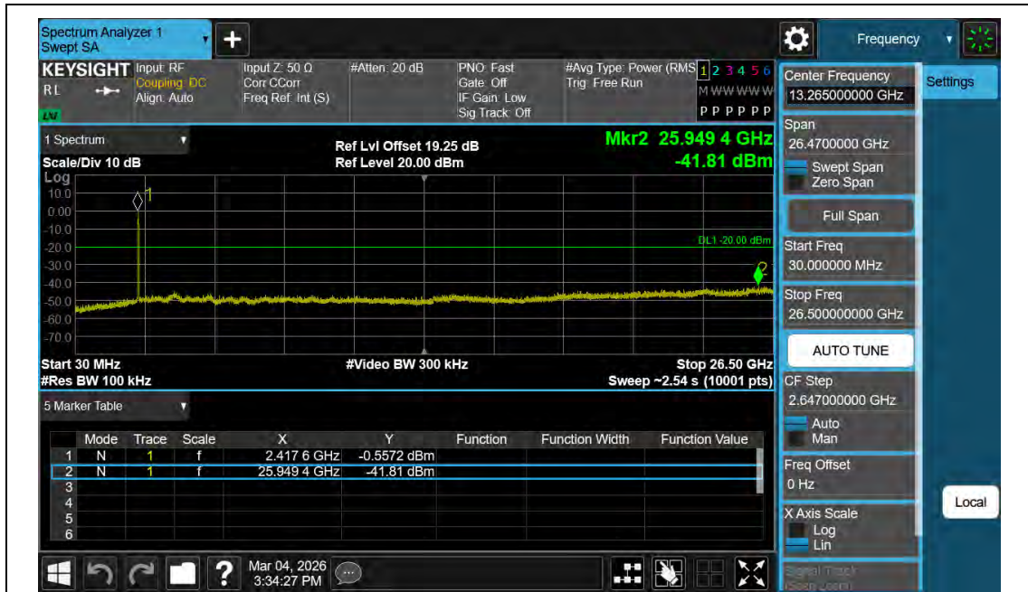
11BE40MIMO-Ant1-2437-30~26500-PASS
