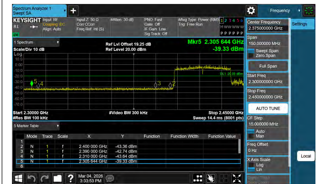
11BE40MIMO-Ant1-2452-PASS
