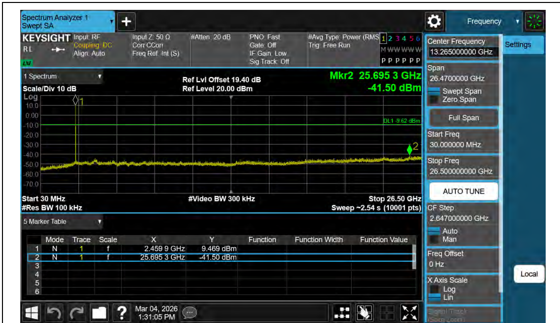
11B-Ant2-2462-30~26500-PASS
