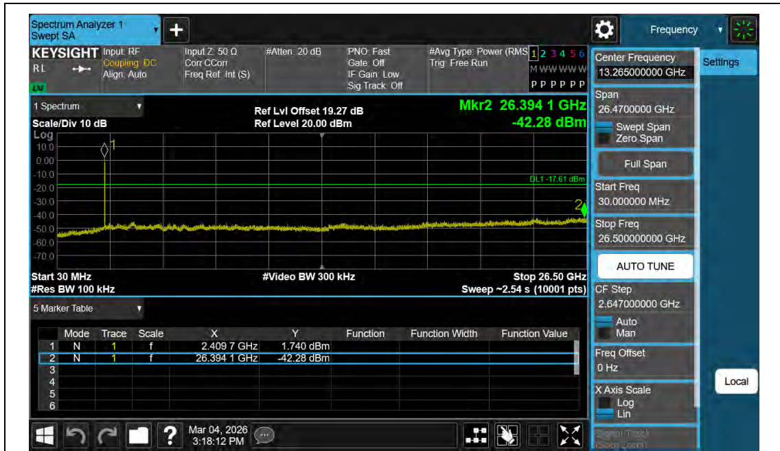
11BE20MIMO-Ant2-2412-30~26500-PASS
