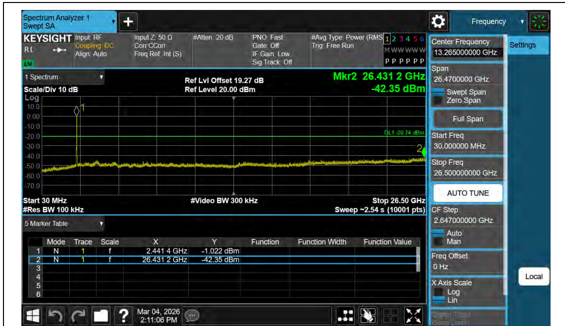
11N40MIMO-Ant2-2437-30~26500-PASS
