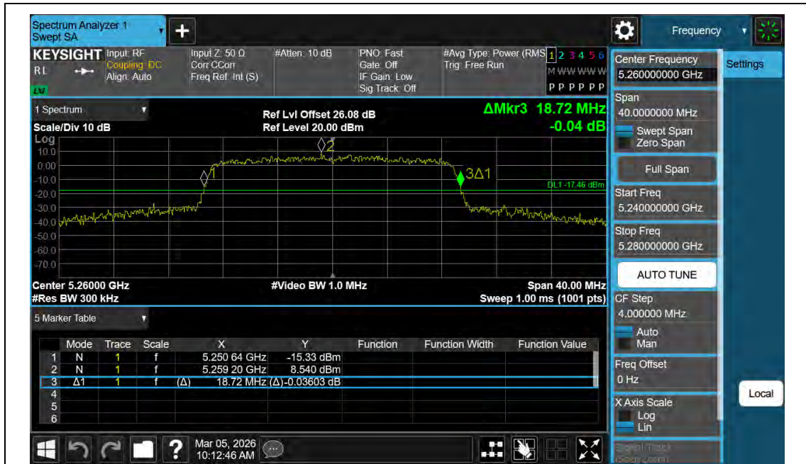
11AC20MIMO-Ant2-5260
