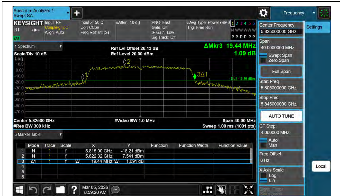
11N20MIMO-Ant2-5825
