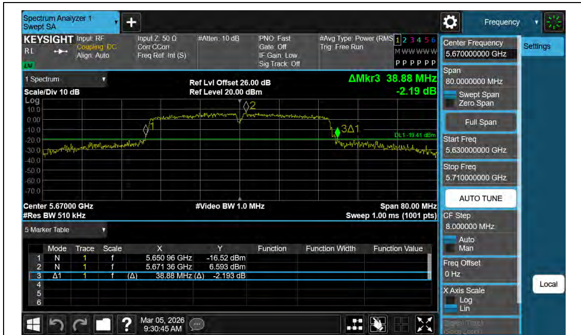
11N40MIMO-Ant2-5670
