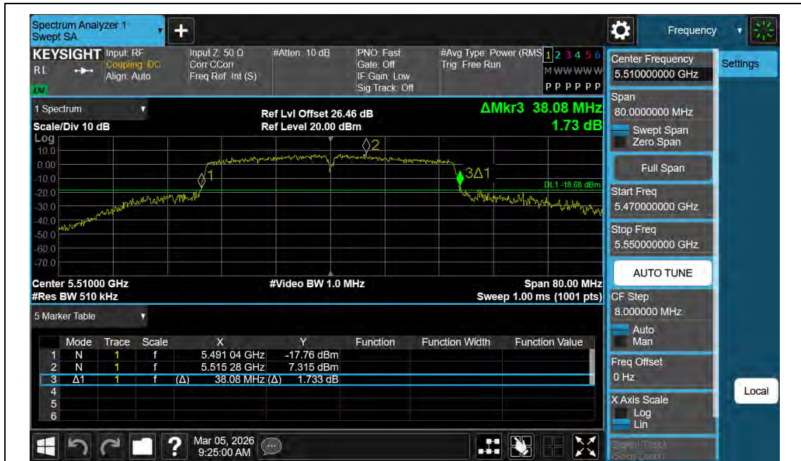
11N40MIMO-Ant2-5510
