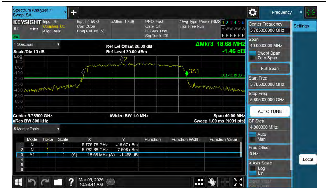
11AC20MIMO-Ant2-5785
