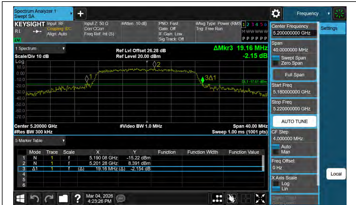
11A-Ant2-5200
