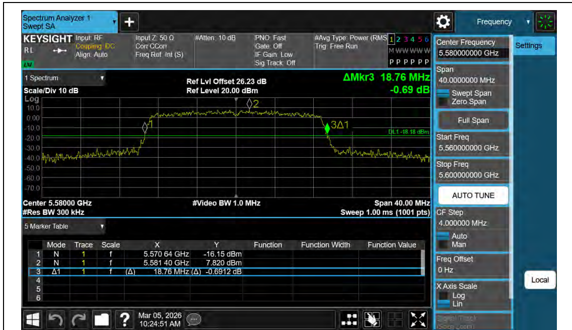
11AC20MIMO-Ant2-5580
