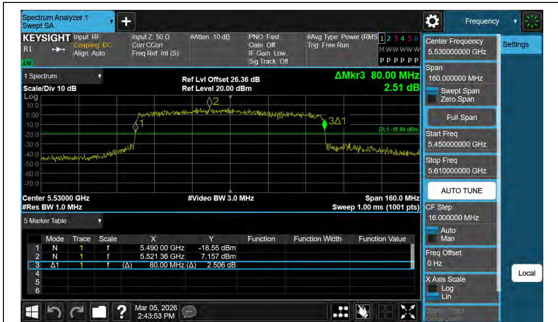
11AX80MIMO-Ant2-5530
