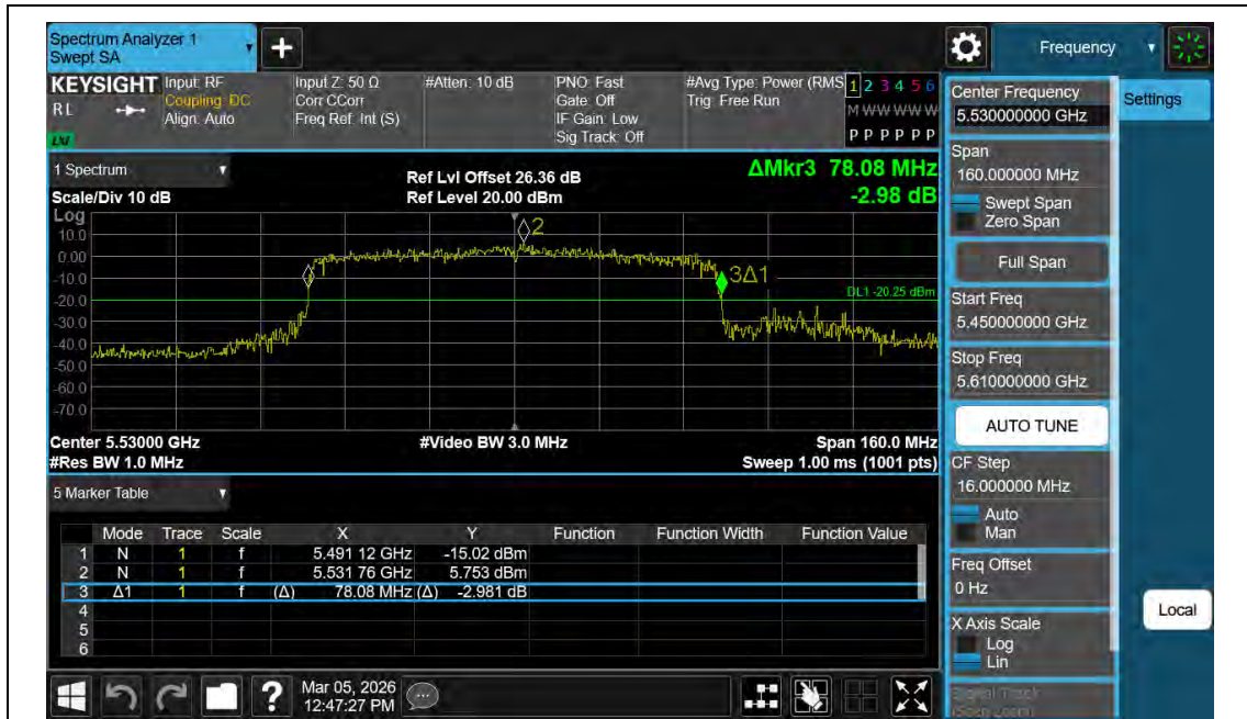
11AC80MIMO-Ant2-5530
