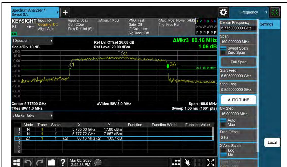
11AX80MIMO-Ant2-5775
