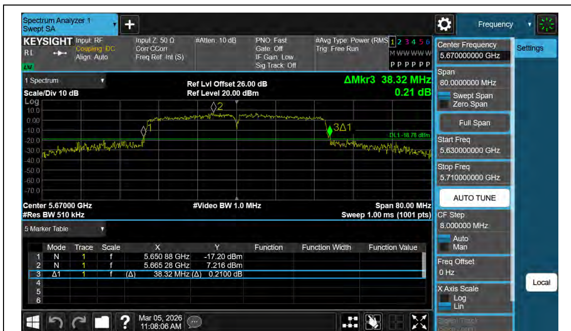
11AC40MIMO-Ant2-5670
