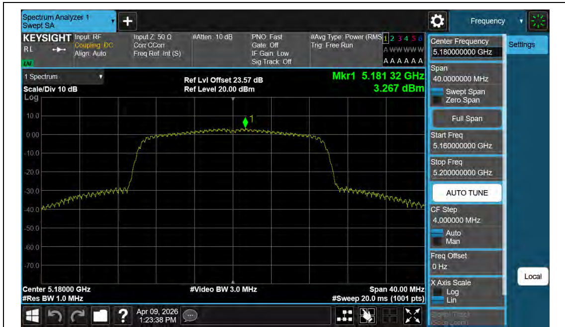
11AX20MIMO-Ant2-5180-PASS
