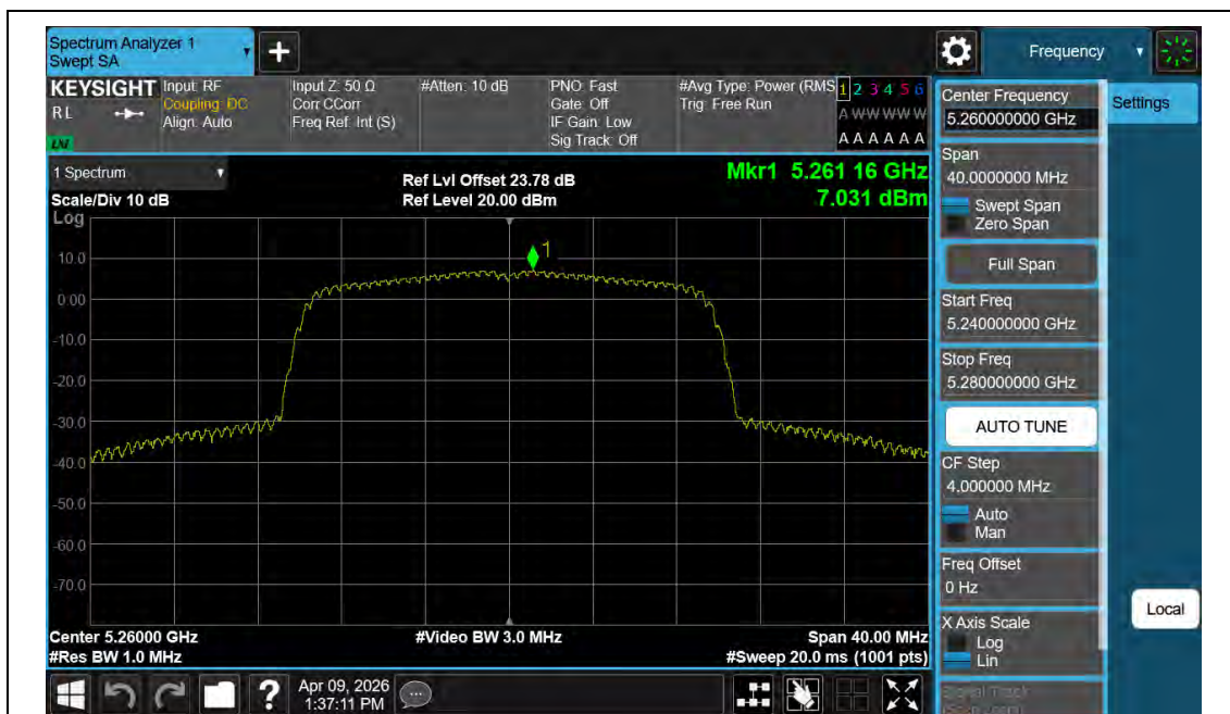
11AX20MIMO-Ant2-5260-PASS
