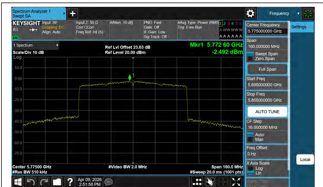
11AX80MIMO-Ant2-5775-PASS
