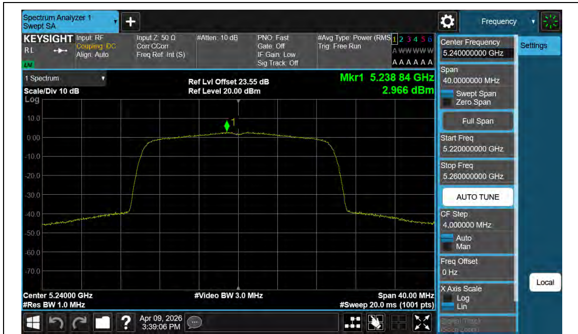
11BE20MIMO-Ant2-5240-PASS
