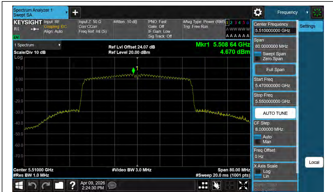
11AX40MIMO-Ant2-5510-PASS
