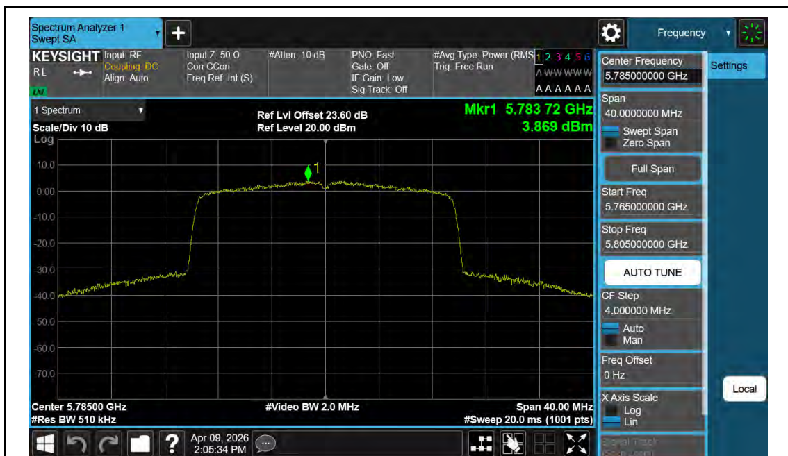
11AX20MIMO-Ant2-5785-PASS
