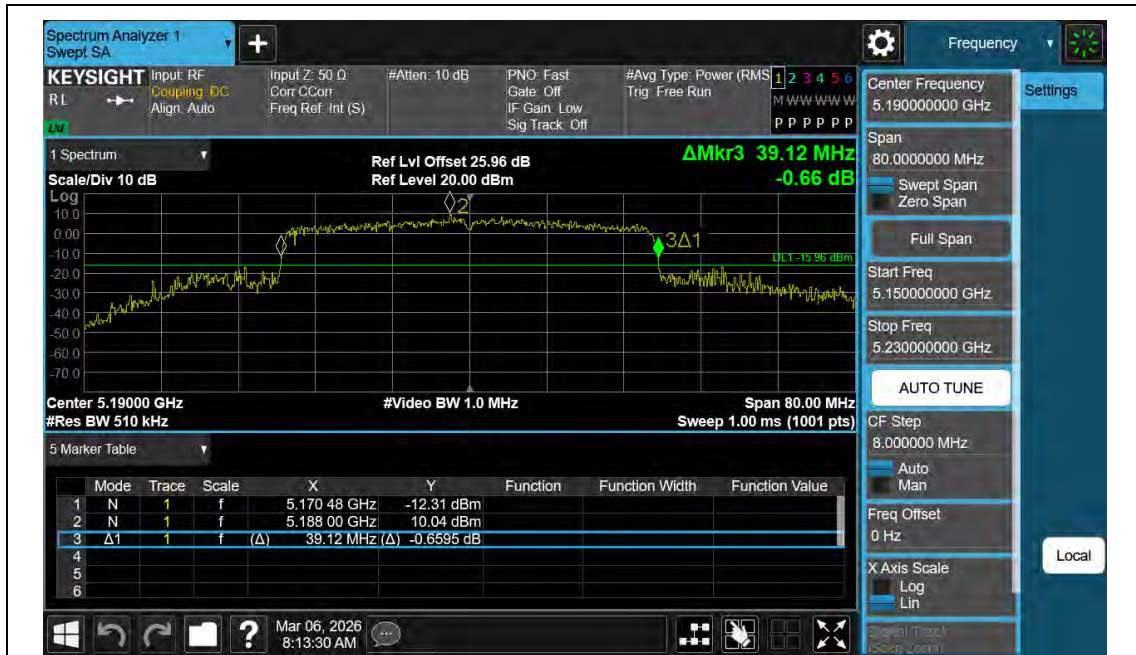
11BE40MIMO-Ant2-5190
