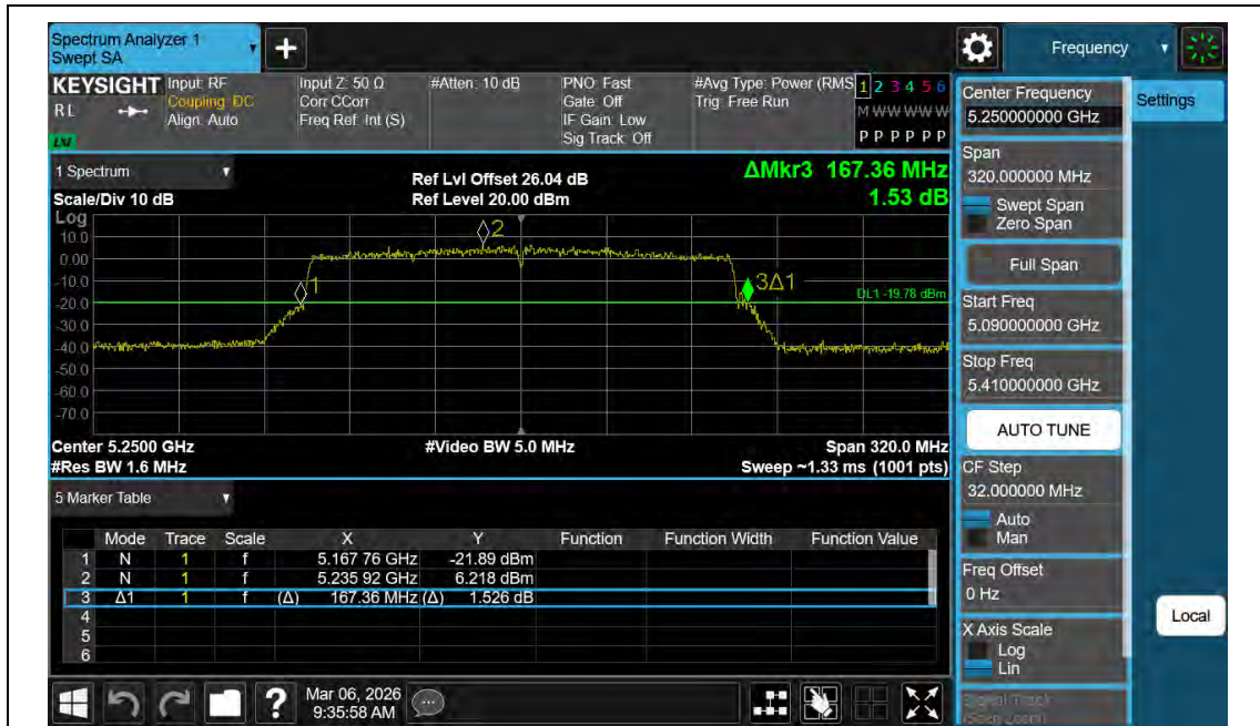
11BE160MIMO-Ant2-5250
