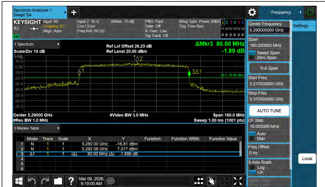
11BE80MIMO-Ant2-5290
