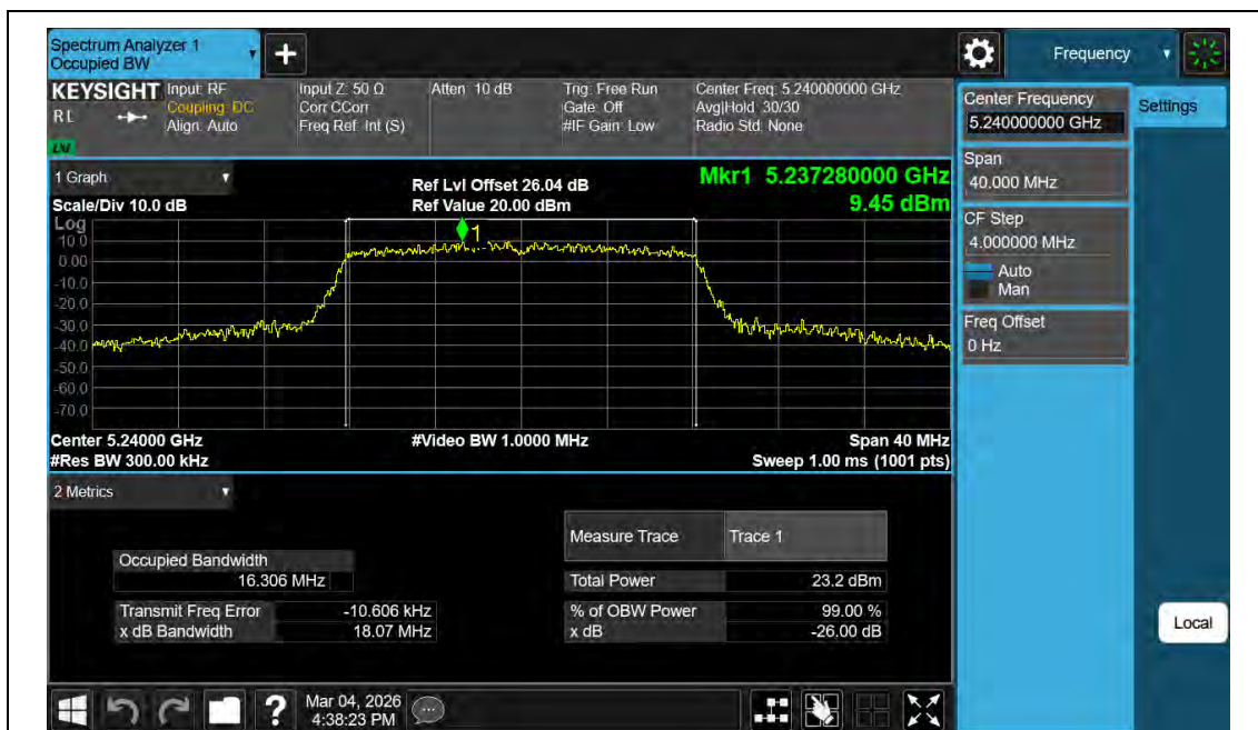
11A-Ant2-5240
