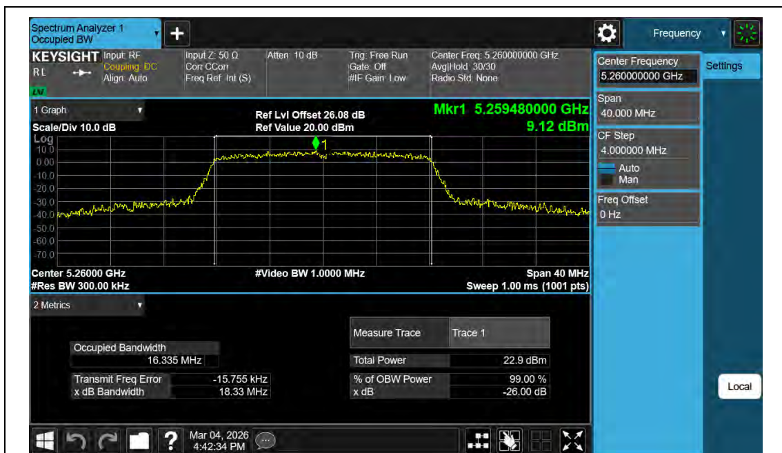
11A-Ant2-5260
