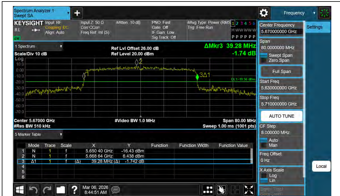
11BE40MIMO-Ant2-5670
