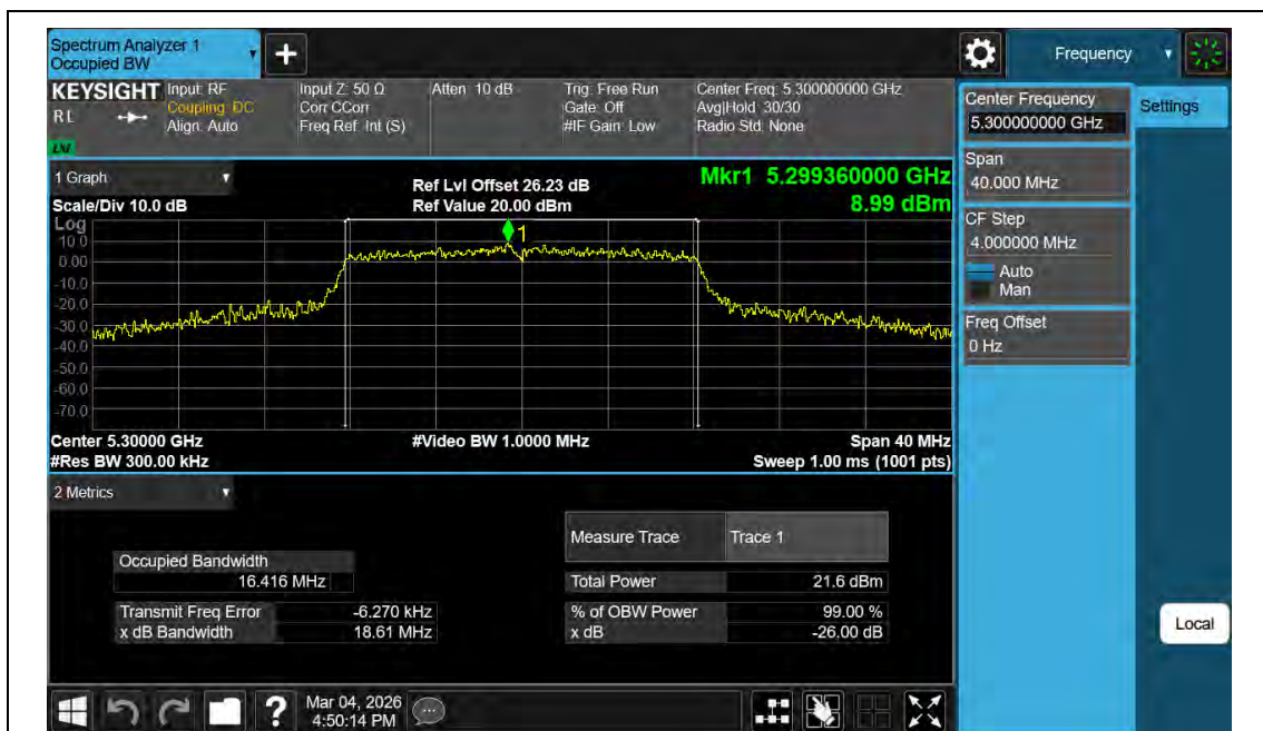
11A-Ant2-5300
