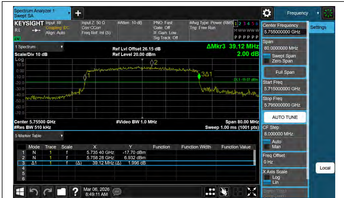
11BE40MIMO-Ant2-5755
