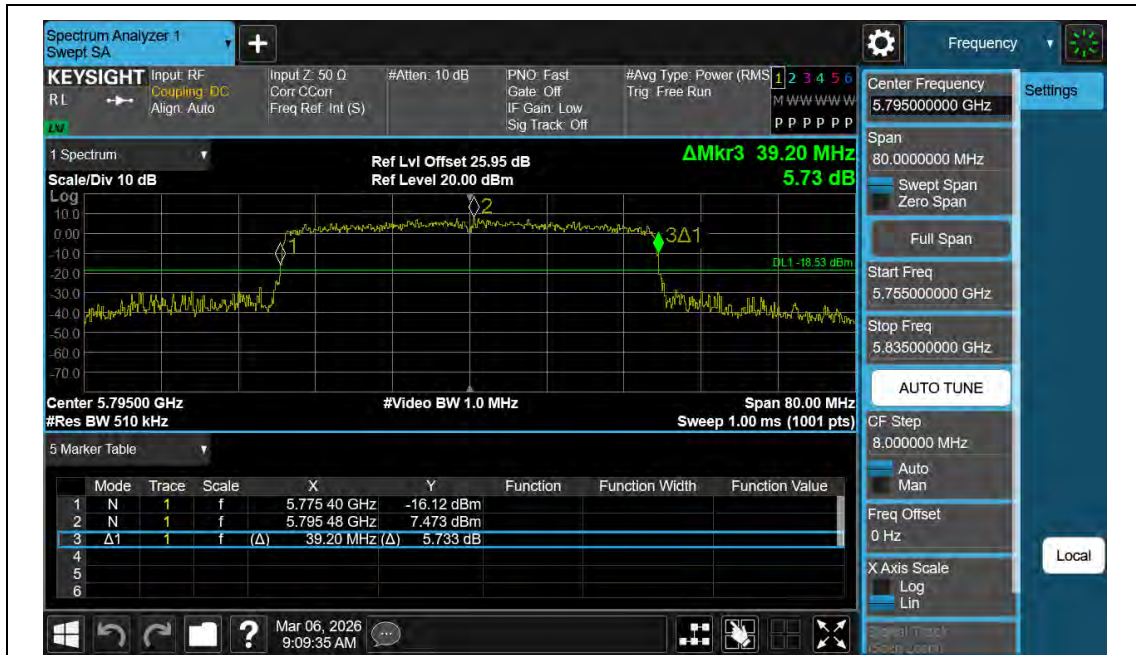
11BE40MIMO-Ant2-5795
