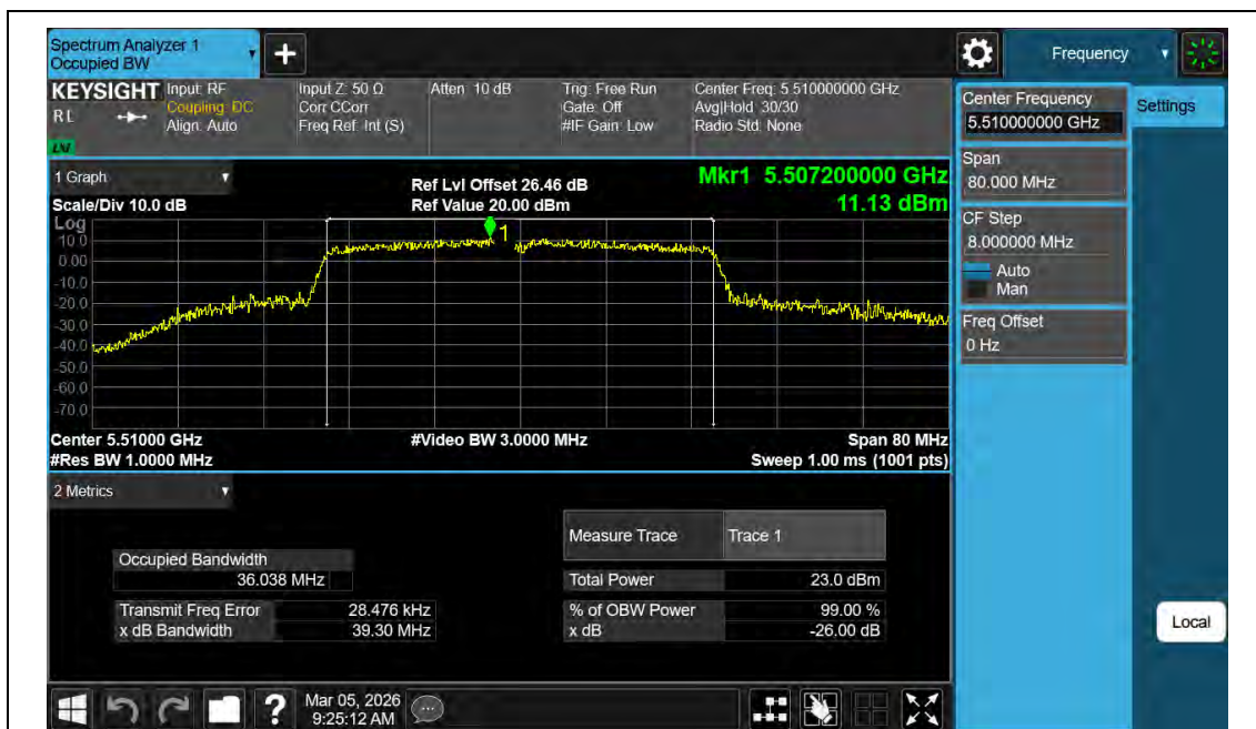
11N40MIMO-Ant2-5510
