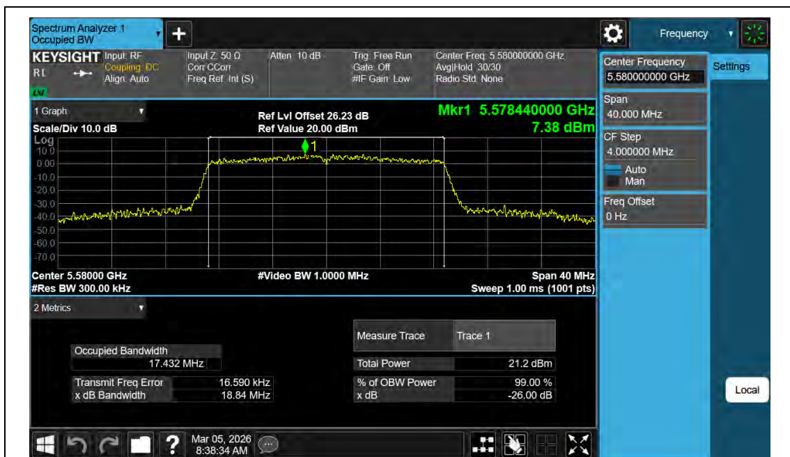
11N20MIMO-Ant2-5580
