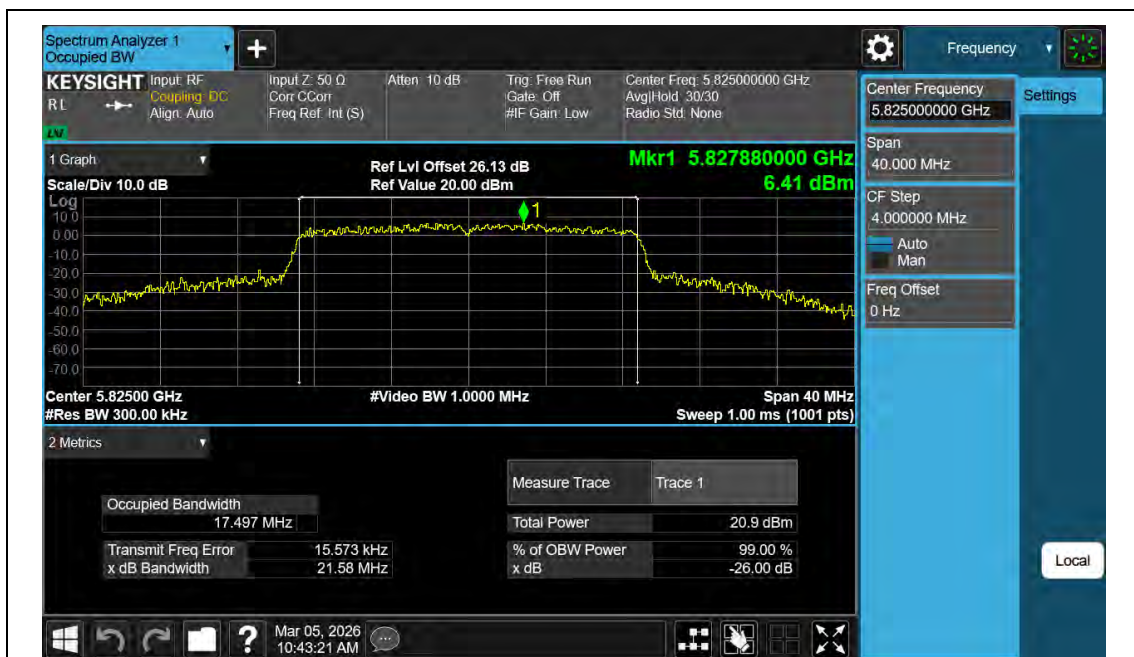
11AC20MIMO-Ant2-5825
