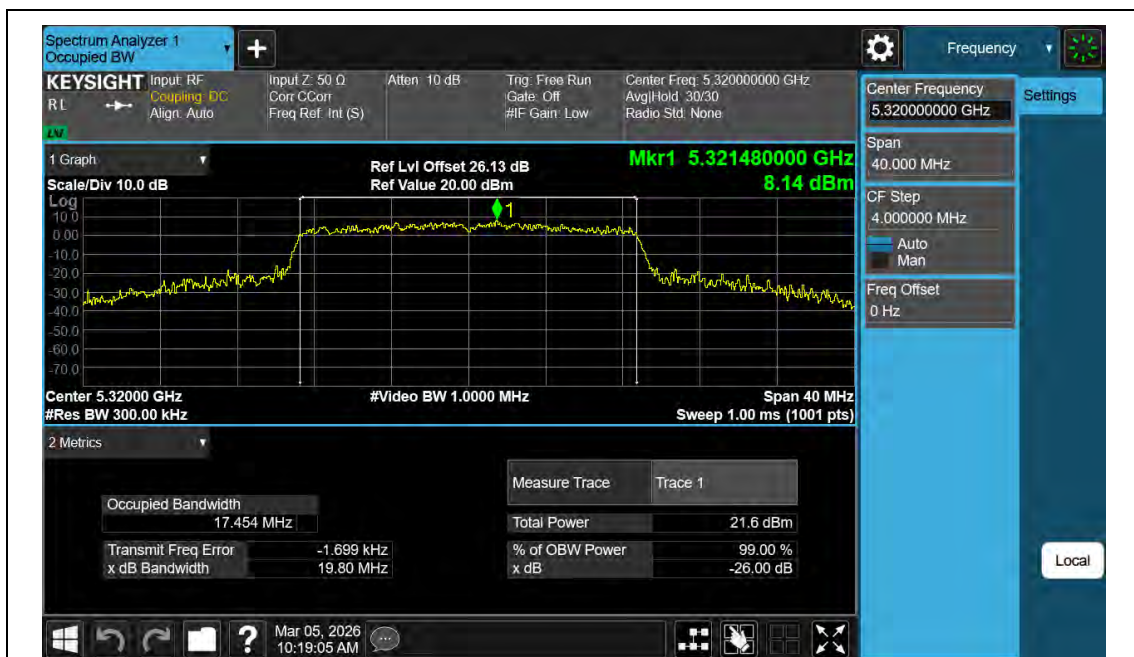
11AC20MIMO-Ant2-5320
