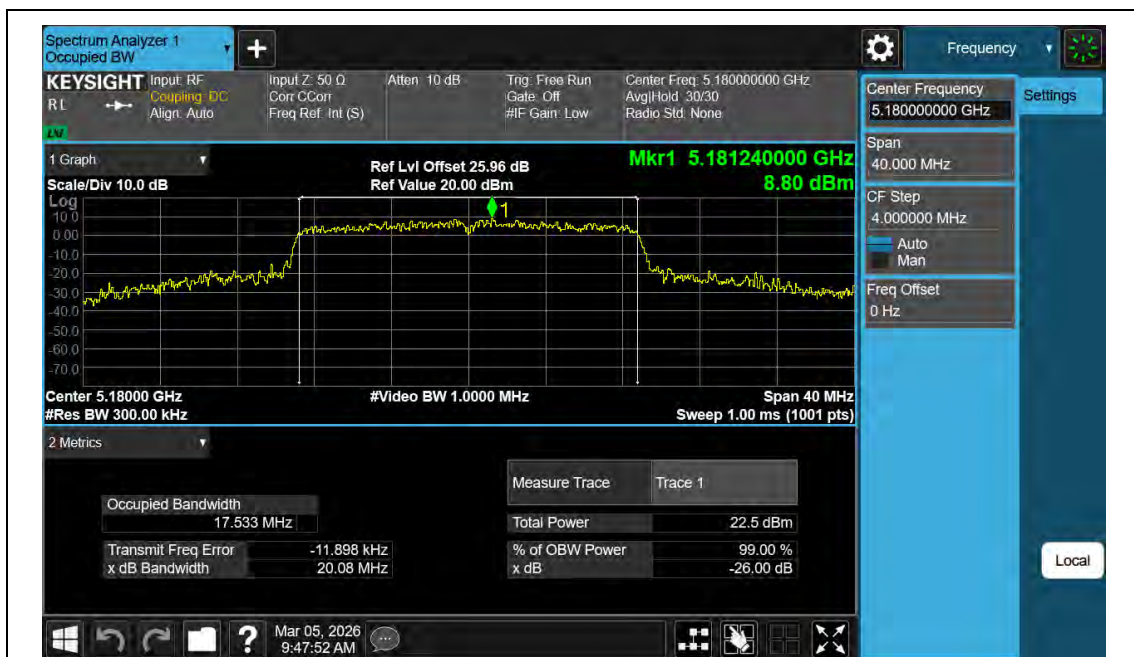
11AC20MIMO-Ant2-5180
