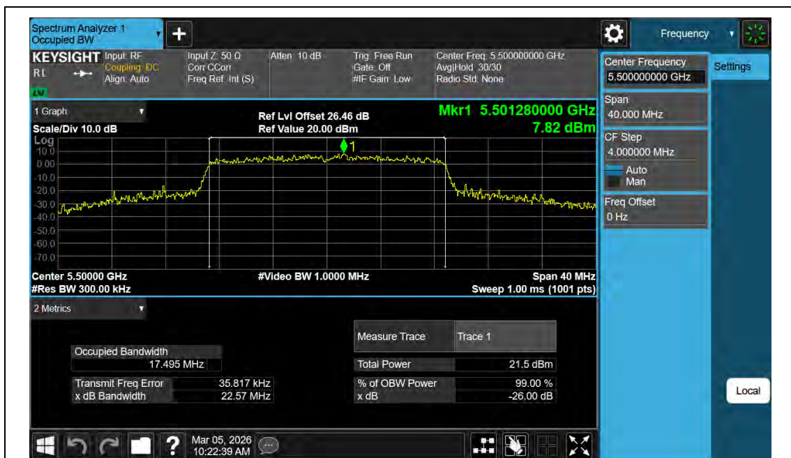
11AC20MIMO-Ant2-5500
