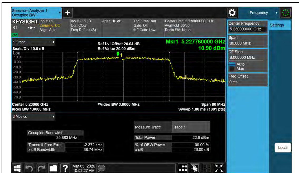
11AC40MIMO-Ant2-5230
