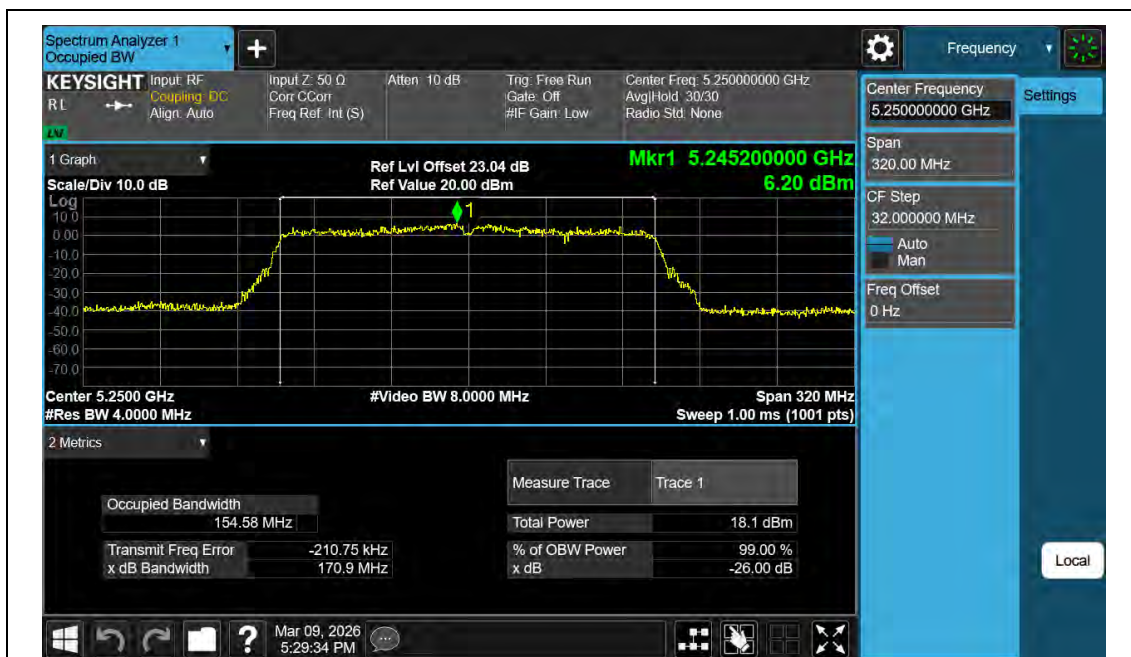
11AC160MIMO-Ant2-5250
