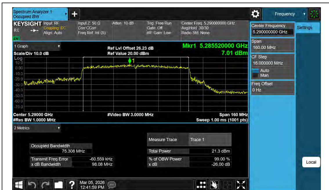
11AC80MIMO-Ant2-5290
