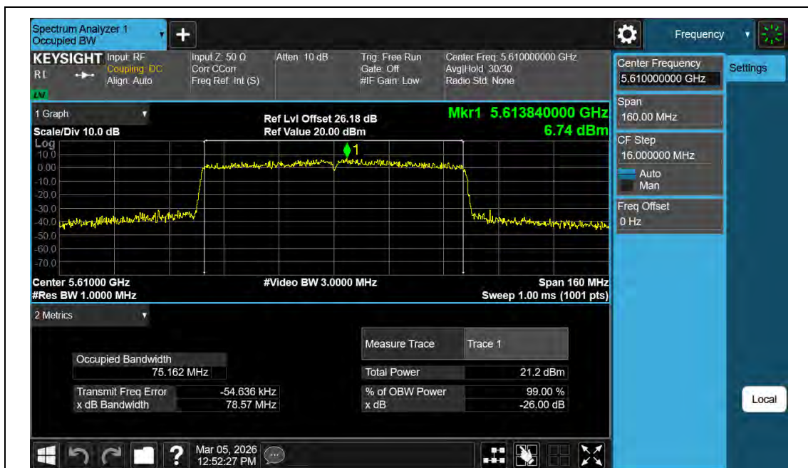
11AC80MIMO-Ant2-5610
