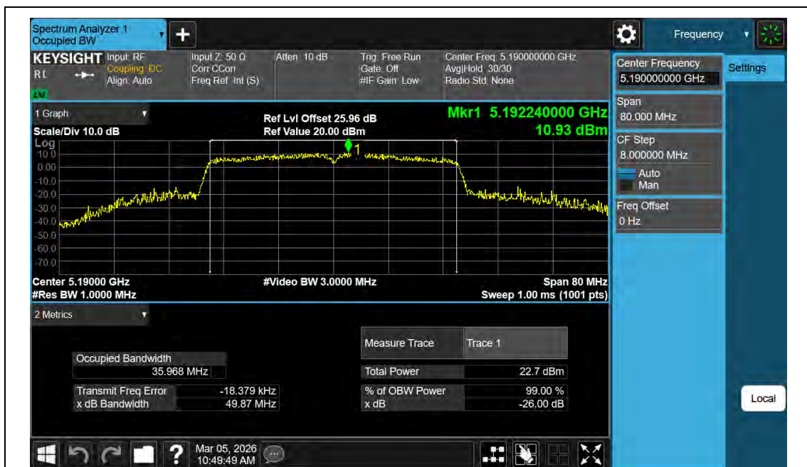
11AC40MIMO-Ant2-5190
