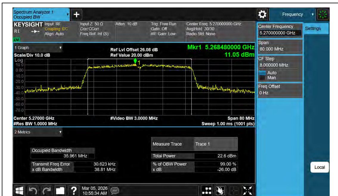
11AC40MIMO-Ant2-5270
