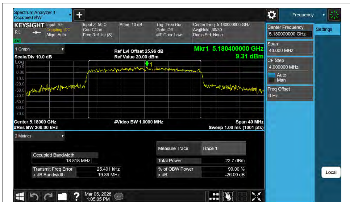
11AX20MIMO-Ant2-5180
