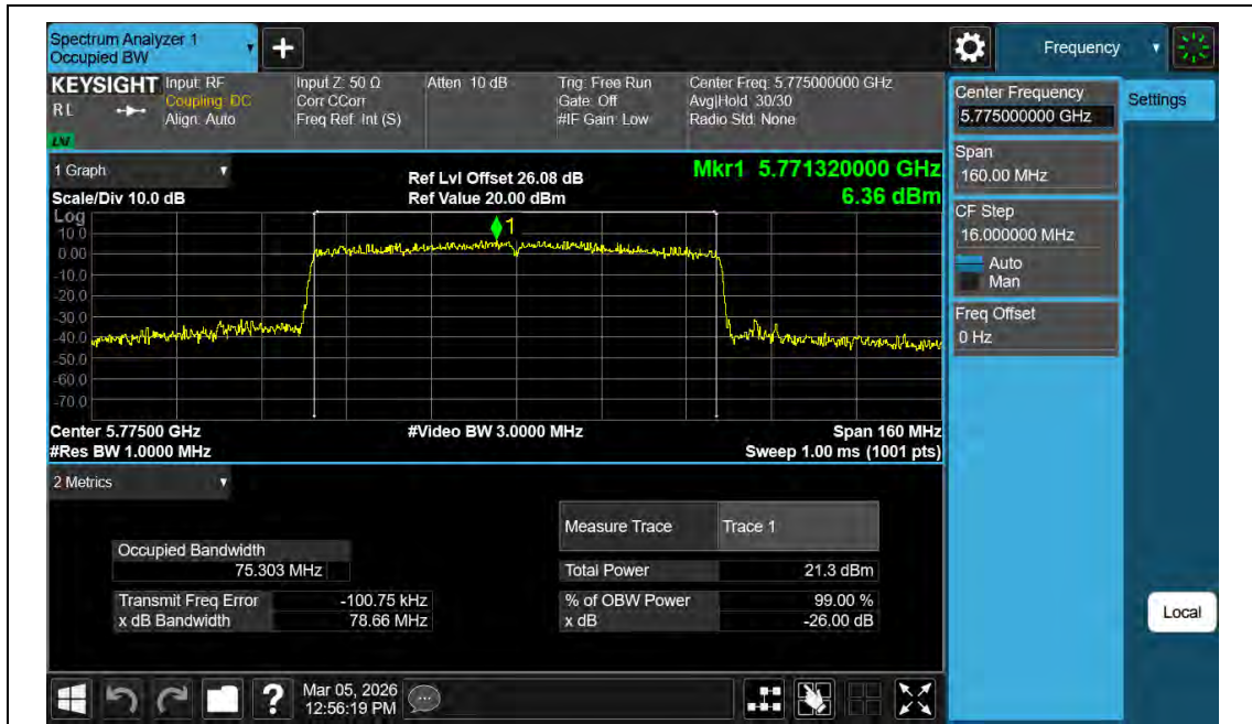
11AC80MIMO-Ant2-5775
