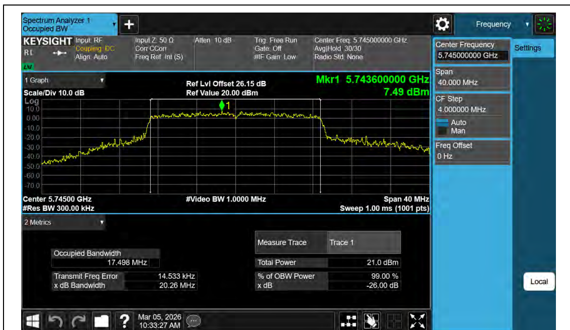
11AC20MIMO-Ant2-5745
