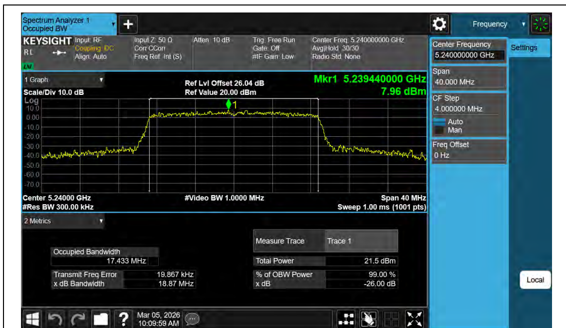
11AC20MIMO-Ant2-5240
