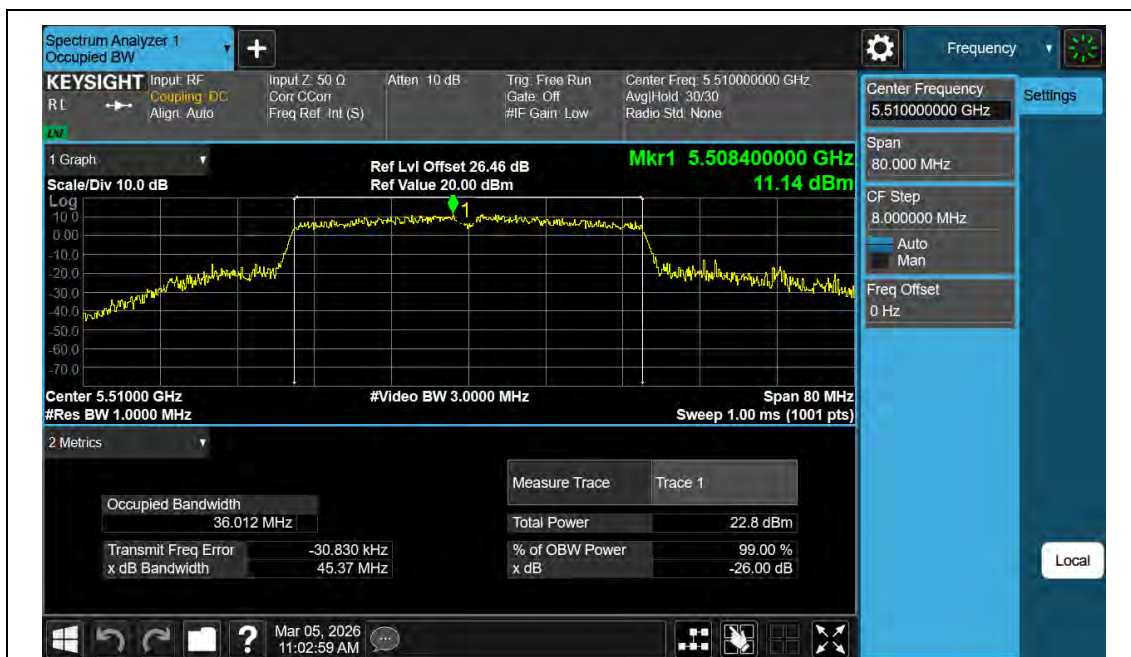
11AC40MIMO-Ant2-5510
