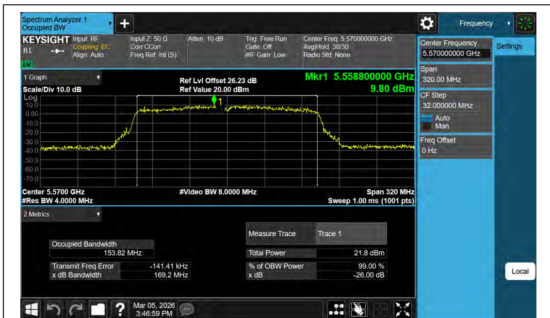
11AC160MIMO-Ant2-5570
