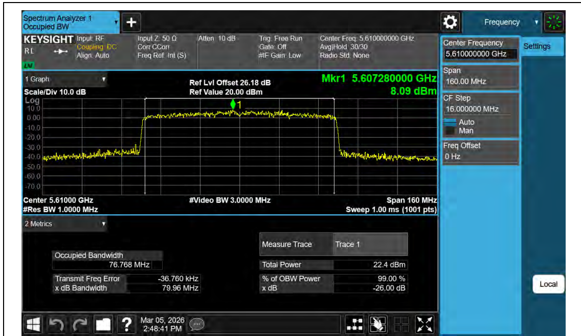
11AX80MIMO-Ant2-5610
