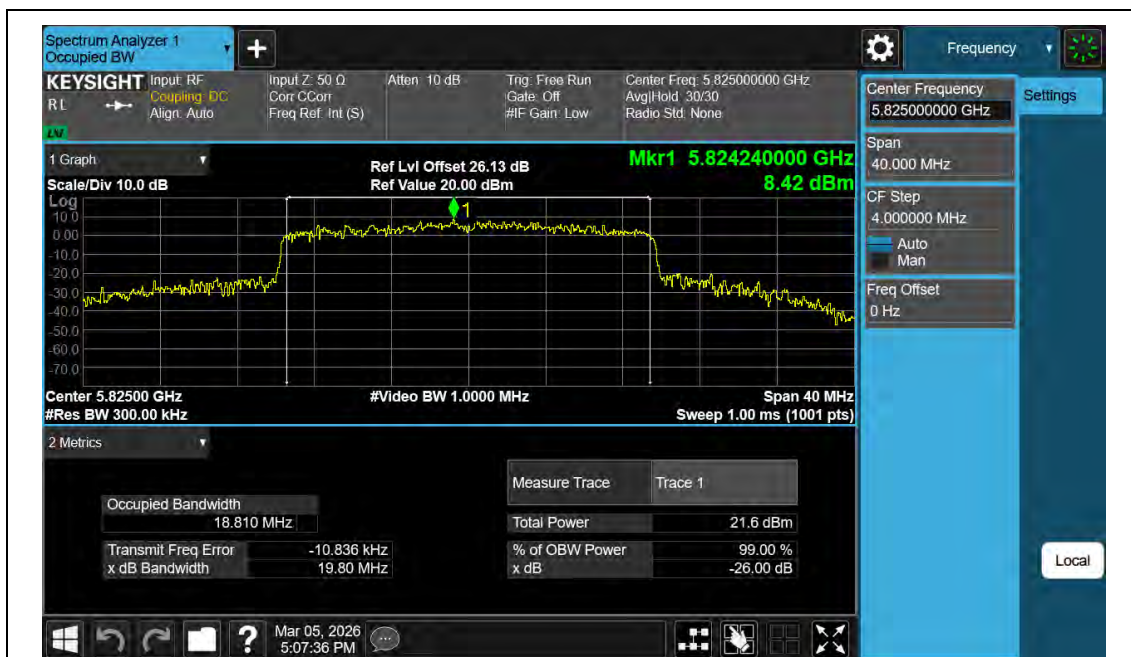
11BE20MIMO-Ant2-5825
