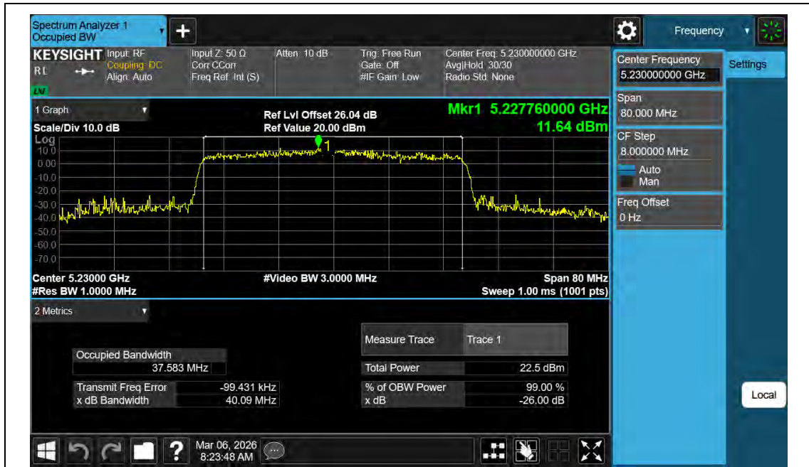
11BE40MIMO-Ant2-5230
