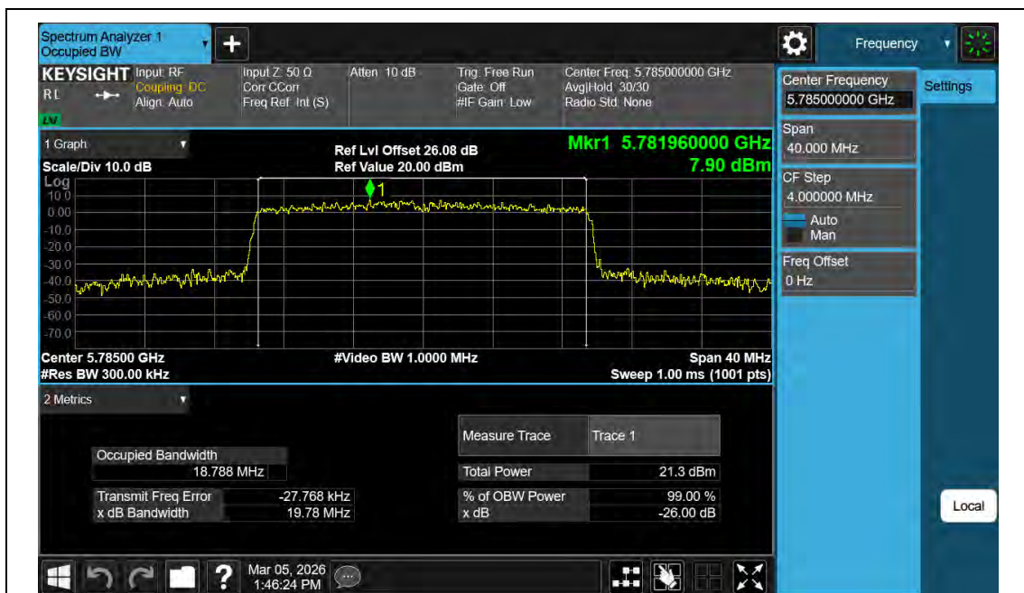
11AX20MIMO-Ant2-5785
