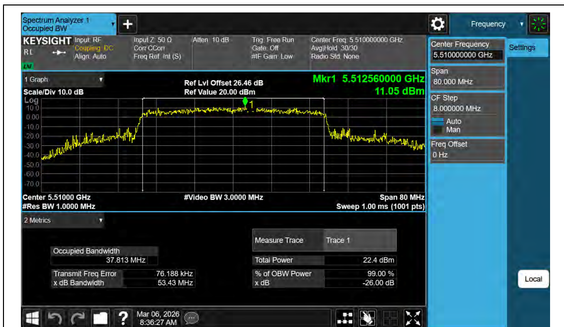
11BE40MIMO-Ant2-5510
