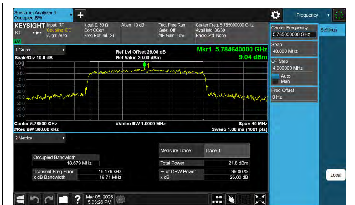
11BE20MIMO-Ant2-5785
