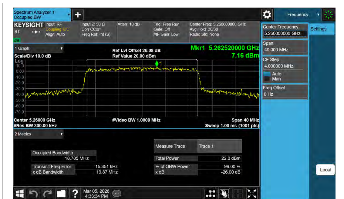
11BE20MIMO-Ant2-5260
