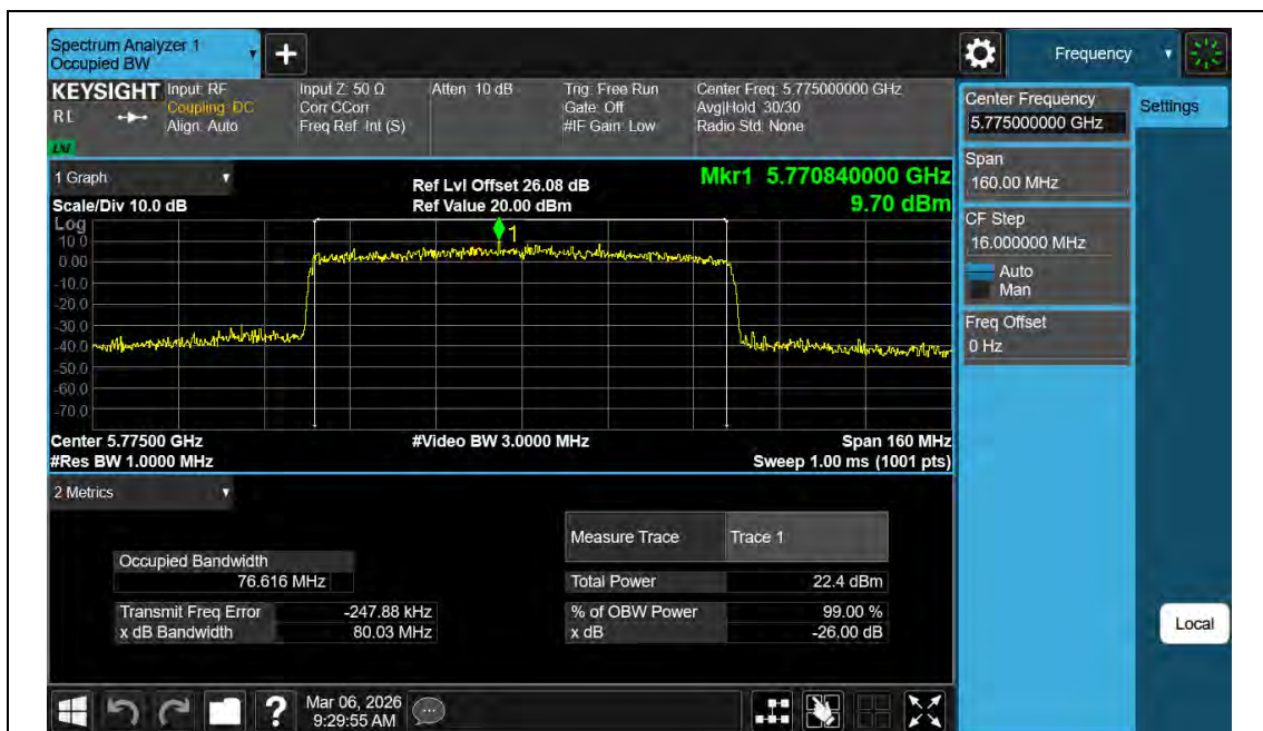
11BE80MIMO-Ant2-5775
