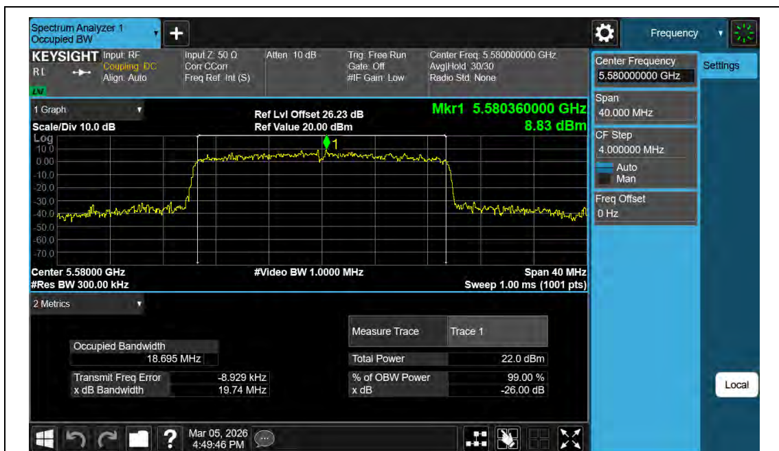
11BE20MIMO-Ant2-5580
