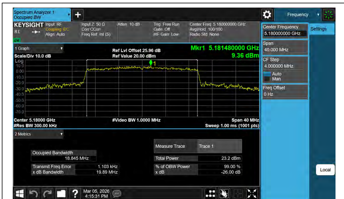
11BE20MIMO-Ant2-5180
