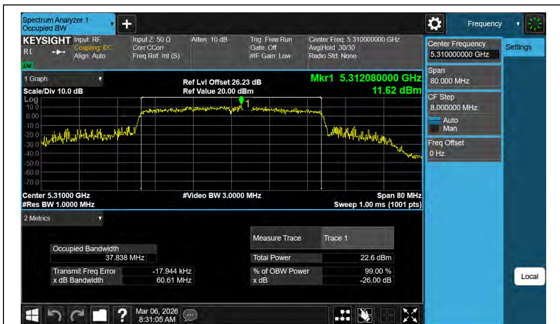
11BE40MIMO-Ant2-5310
