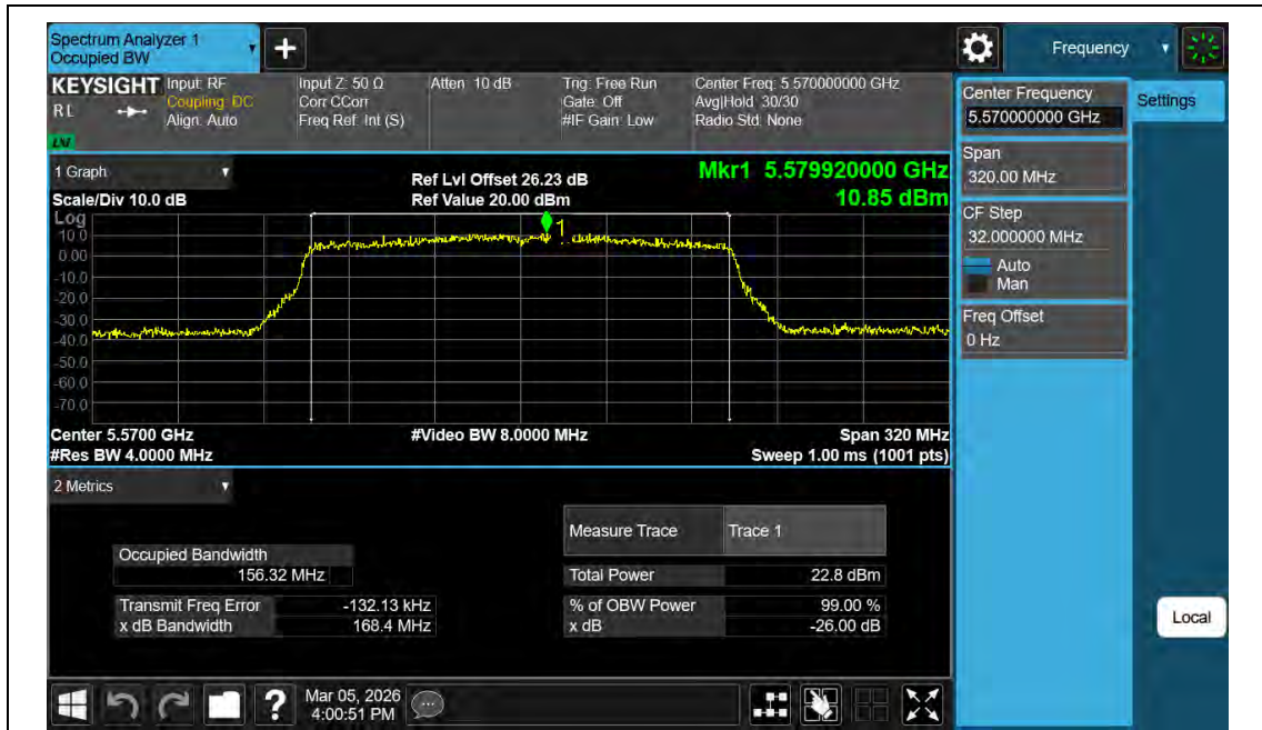
11AX160MIMO-Ant2-5570
