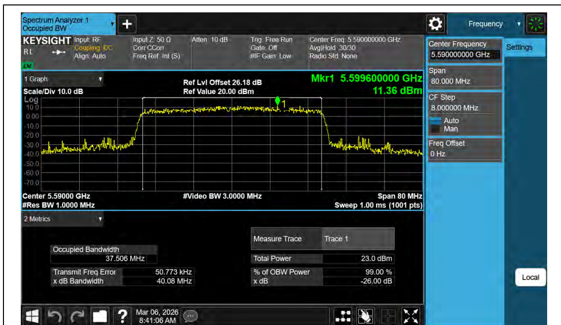
11BE40MIMO-Ant2-5590
