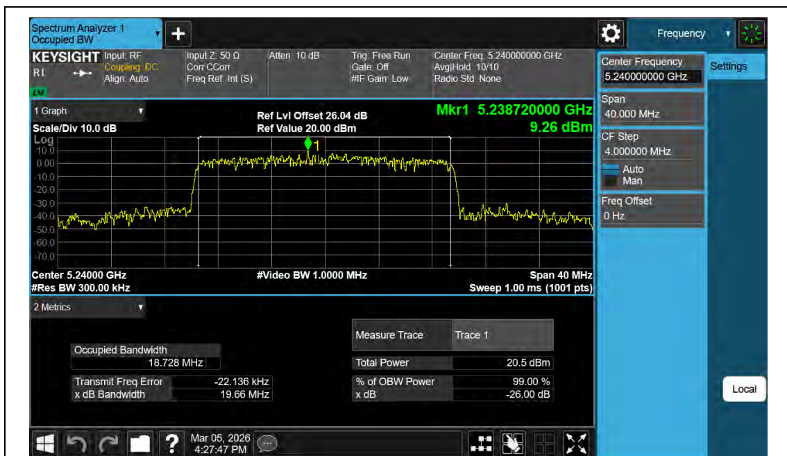
11BE20MIMO-Ant2-5240
