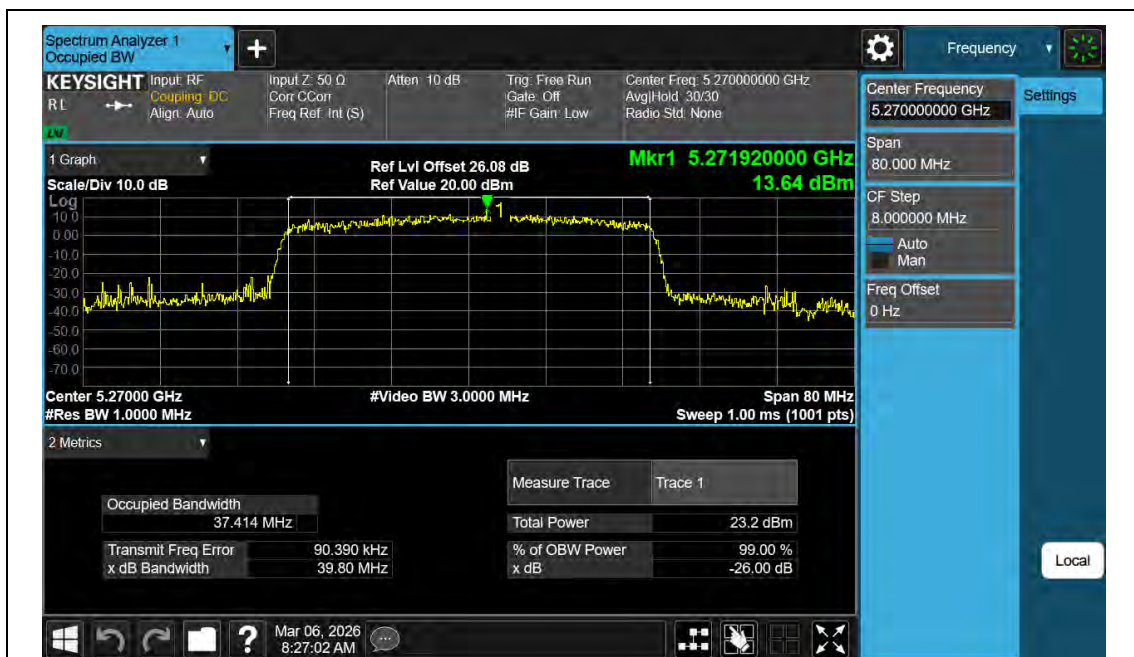
11BE40MIMO-Ant2-5270
