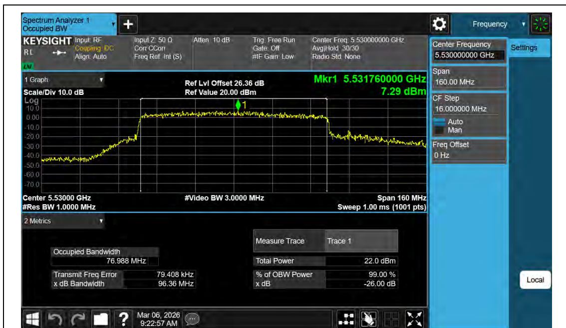
11BE80MIMO-Ant2-5530
