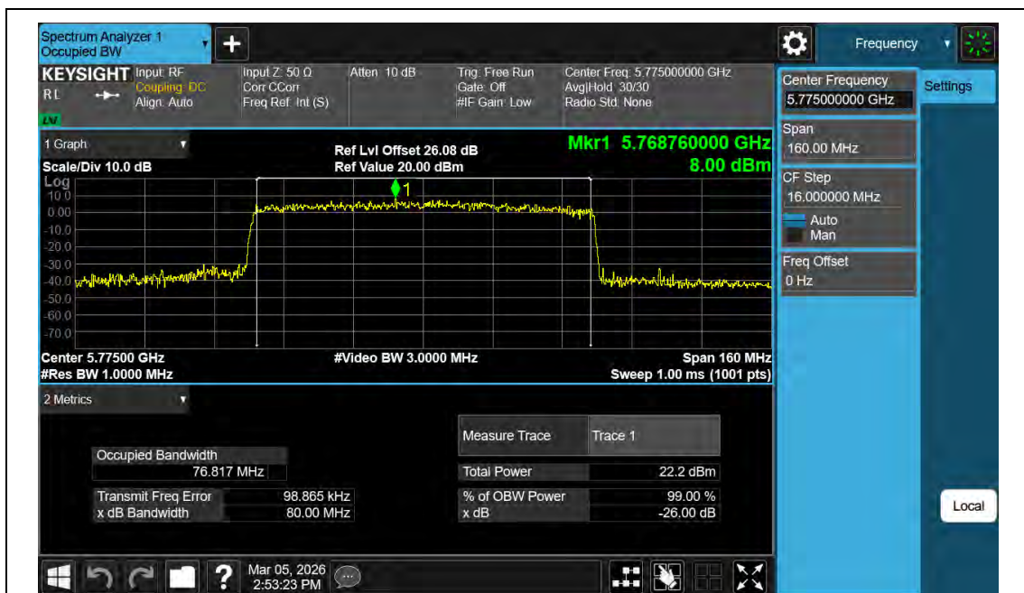
11AX80MIMO-Ant2-5775
