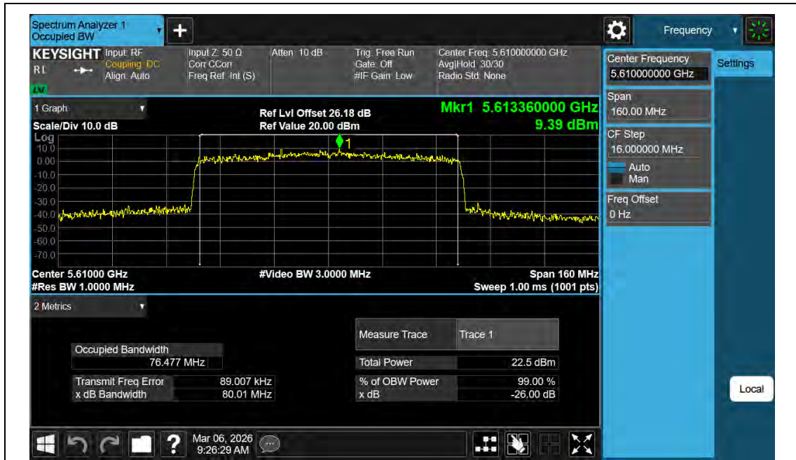
11BE80MIMO-Ant2-5610
